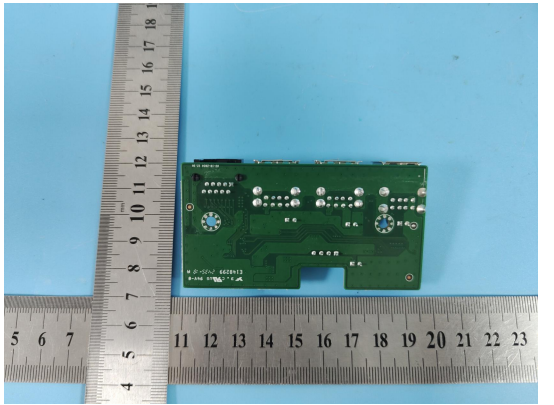
INTERNAL PHOTO OF SAMPLE PCB
