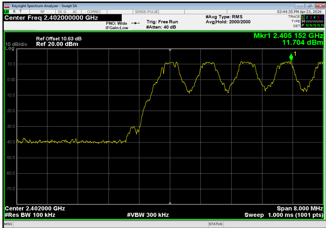
Band Edge(Hopping) 1-DH5 2402MHz Hopping Emission
