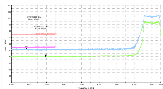
802.11ac VHT20 -Channel 52: Peak + Average
