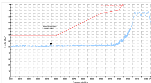
802.11a-Channel 149: Peak
