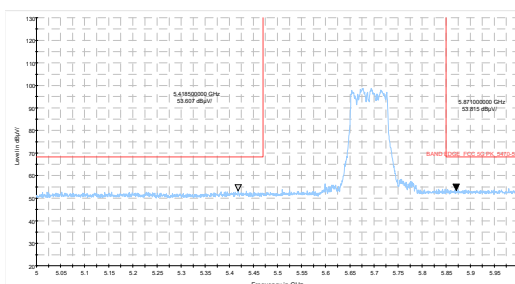
802.11ac VHT80- Channel 138: Peak
