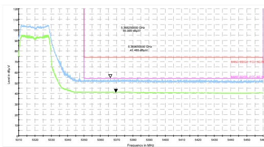
802.11ac VHT20 -Channel 64: Peak + Average
