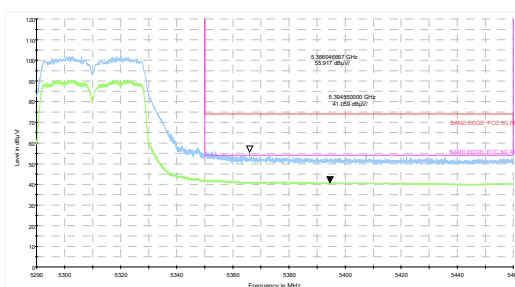
802.11ac VHT40-Channel 62: Peak + Average
