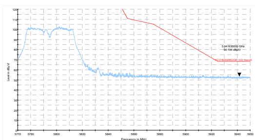
802.11ac VHT40-Channel 159: Peak
