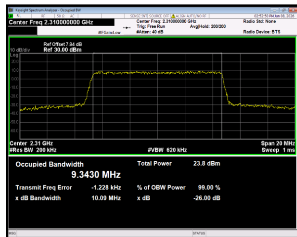
n30 SCS=15kHz CP_256QAM BW=10MHz Channel=462000 RB=52@0
