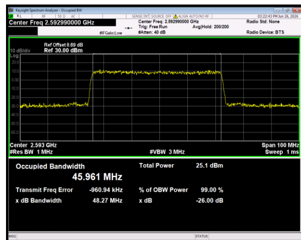
n41 SCS=30kHz DFT_64QAM BW=50MHz Channel=518598 RB=128@0
