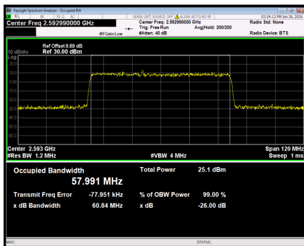
n41 SCS=30kHz DFT_64QAM BW=60MHz Channel=518598 RB=162@0
