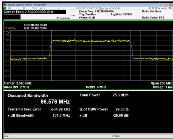
n41 SCS=30kHz DFT_64QAM BW=100MHz Channel=518598 RB=270@0
