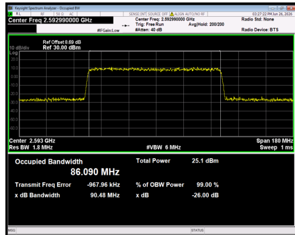
n41 SCS=30kHz DFT_64QAM BW=90MHz Channel=518598 RB=240@0
