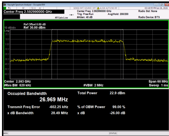
n41 SCS=30kHz DFT_256QAM BW=30MHz Channel=518598 RB=75@0
