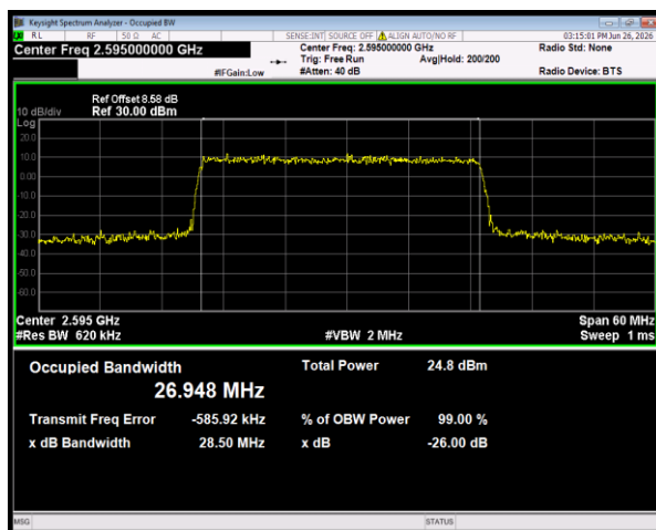
n38 SCS=30kHz DFT_QPSK BW=30MHz Channel=519000 RB=75@0
