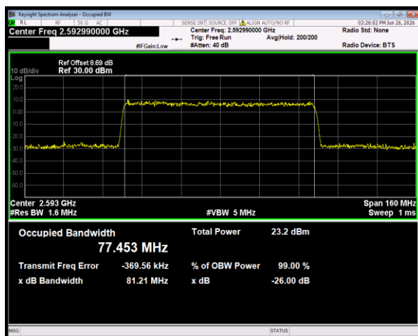
n41 SCS=30kHz DFT_256QAM BW=80MHz Channel=518598 RB=216@0
