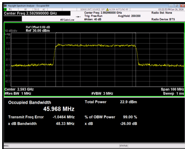
n41 SCS=30kHz DFT_256QAM BW=50MHz Channel=518598 RB=128@0
