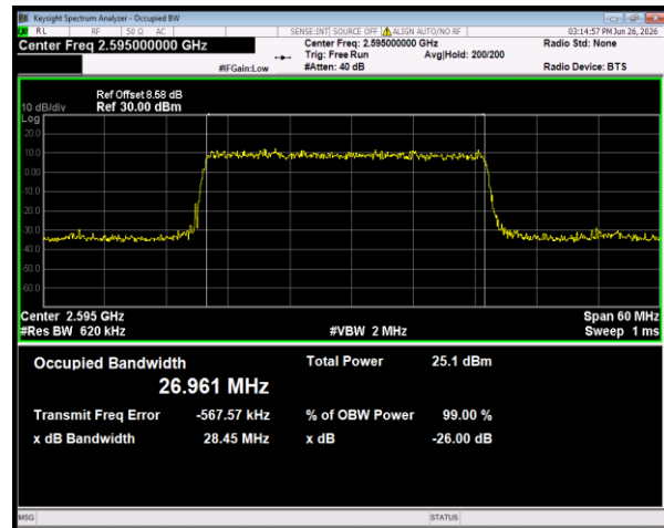
n38 SCS=30kHz DFT_BPSK BW=30MHz Channel=519000 RB=75@0
