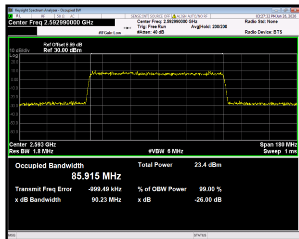
n41 SCS=30kHz DFT_256QAM BW=90MHz Channel=518598 RB=240@0
