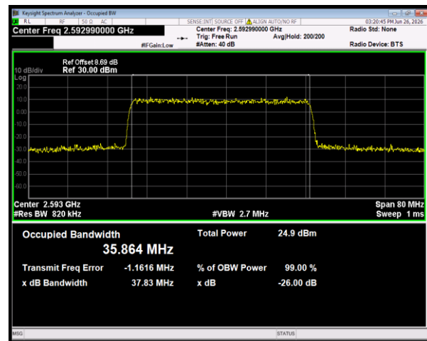
n41 SCS=30kHz DFT_64QAM BW=40MHz Channel=518598 RB=100@0
