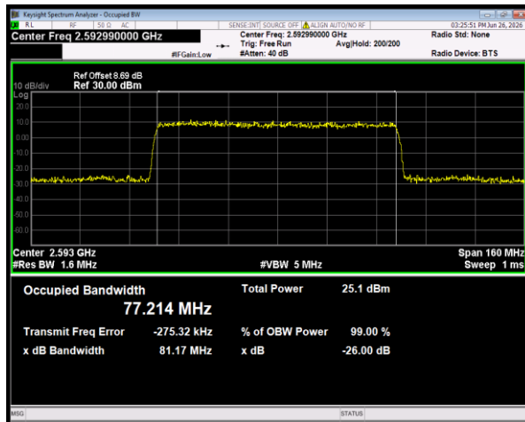
n41 SCS=30kHz DFT_64QAM BW=80MHz Channel=518598 RB=216@0
