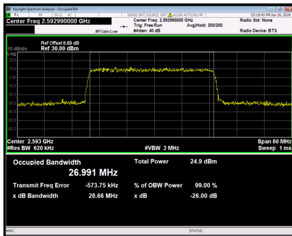
n41 SCS=30kHz DFT_64QAM BW=30MHz Channel=518598 RB=75@0
