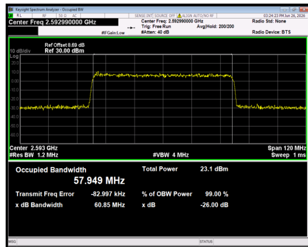
n41 SCS=30kHz DFT_256QAM BW=60MHz Channel=518598 RB=162@0
