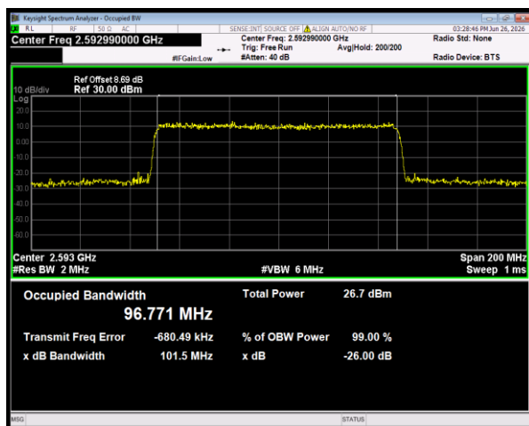
n41 SCS=30kHz DFT_QPSK BW=100MHz Channel=518598 RB=270@0
