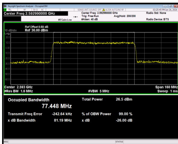
n41 SCS=30kHz DFT_QPSK BW=80MHz Channel=518598 RB=216@0
