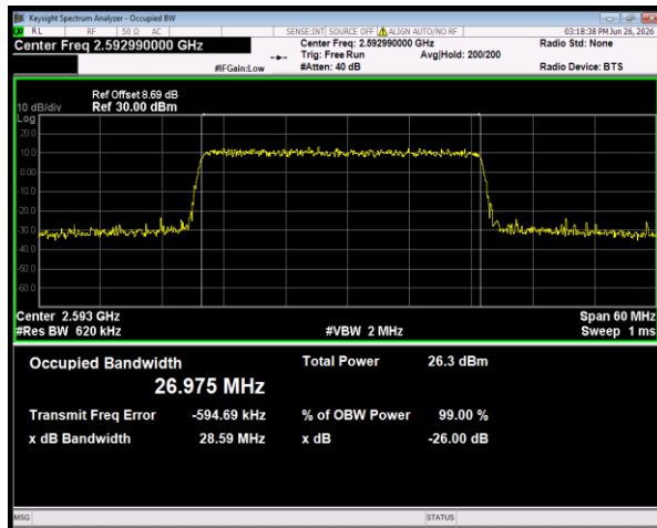
n41 SCS=30kHz DFT_QPSK BW=30MHz Channel=518598 RB=75@0
