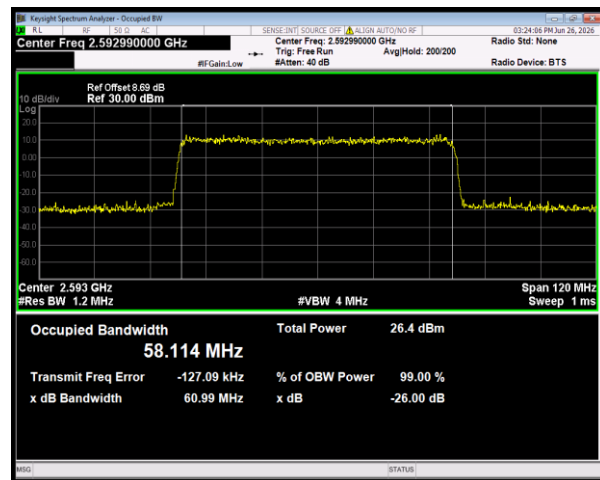
n41 SCS=30kHz DFT_QPSK BW=60MHz Channel=518598 RB=162@0
