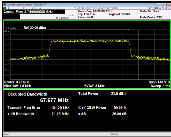
n78(3700-3800) SCS=30kHz CP_64QAM BW=70MHz Channel=650000 RB=189@0
