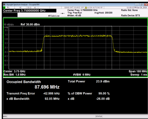
n78(3700-3800) SCS=30kHz CP_64QAM BW=90MHz Channel=650000 RB=245@0
