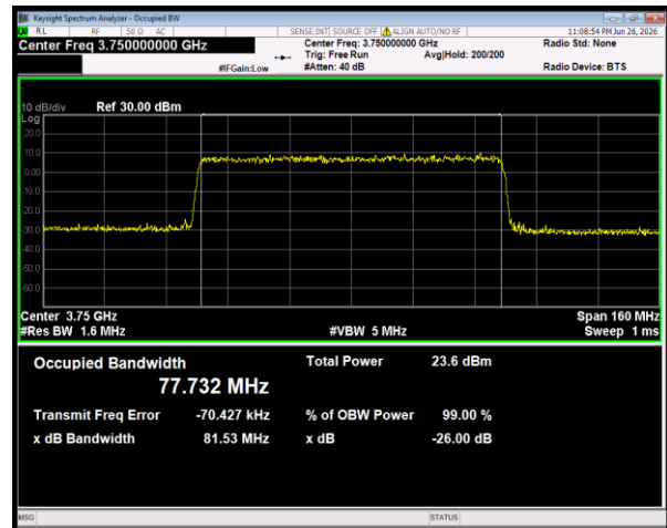
n78(3700-3800) SCS=30kHz CP_64QAM BW=80MHz Channel=650000 RB=217@0
