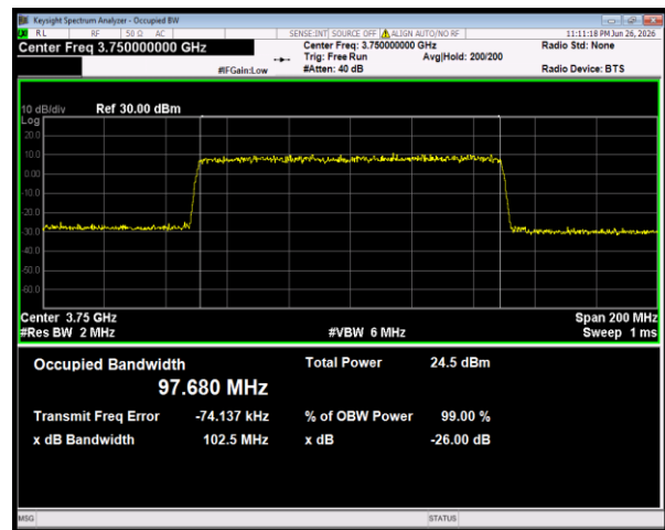
n78(3700-3800) SCS=30kHz CP_QPSK BW=100MHz Channel=650000 RB=273@0
