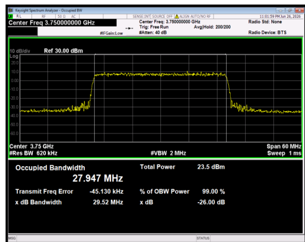
n78(3700-3800) SCS=30kHz CP_QPSK BW=30MHz Channel=650000 RB=78@0
