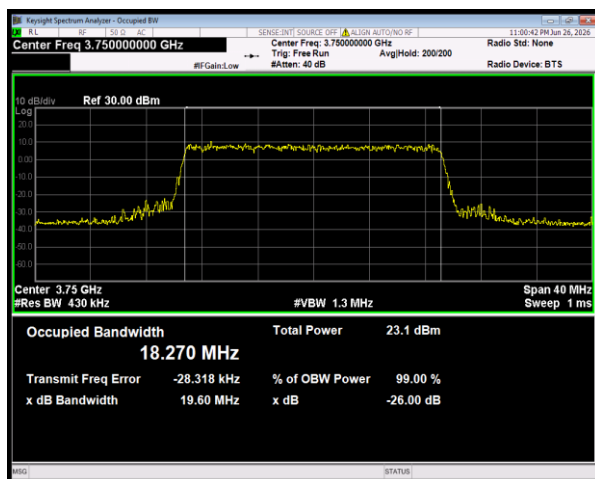
n78(3700-3800) SCS=30kHz CP_QPSK BW=20MHz Channel=650000 RB=51@0
