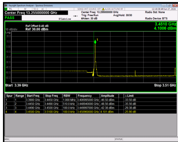
n77(3450-3550) SCS=30kHz CP_16QAM BW=60MHz LowChannel=632000 RB=1@0
