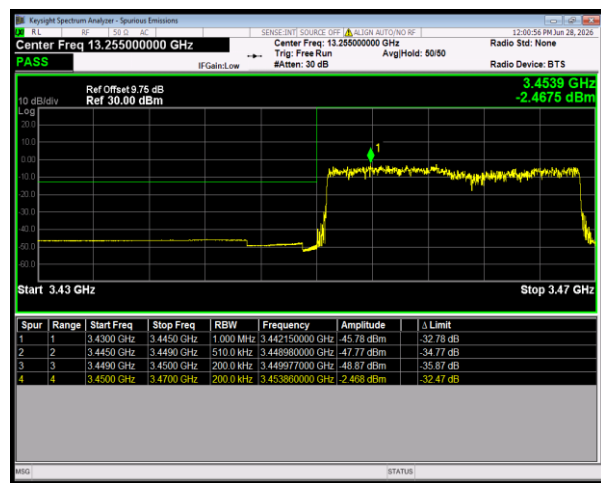
n77(3450-3550) SCS=30kHz DFT_BPSK BW=20MHz LowChannel=630668 RB=50@0
