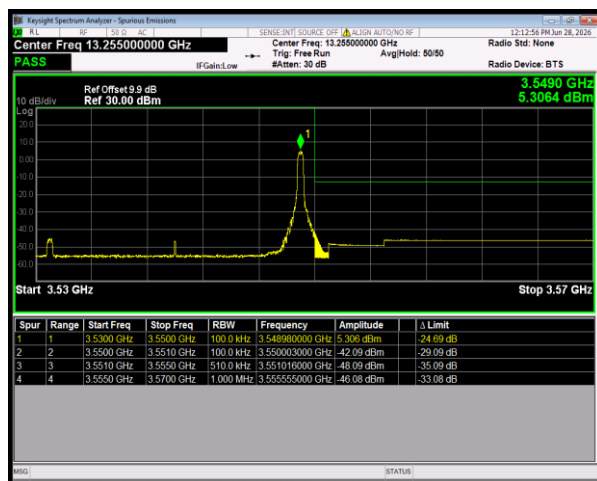
n77(3450-3550) SCS=30kHz DFT_QPSK BW=20MHz HighChannel=636000 RB=1@50
