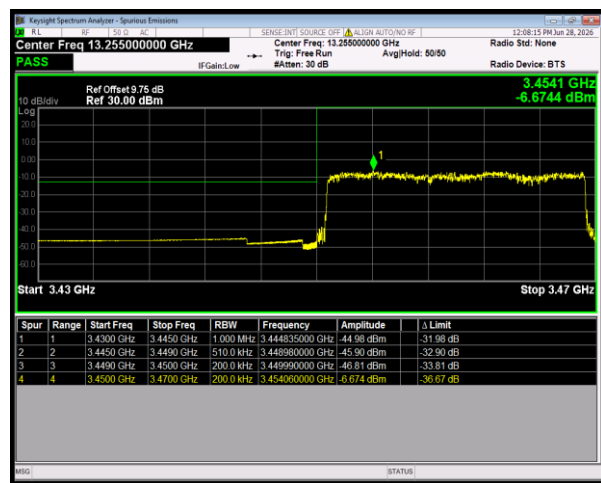
n77(3450-3550) SCS=30kHz CP_16QAM BW=20MHz LowChannel=630668 RB=51@0
