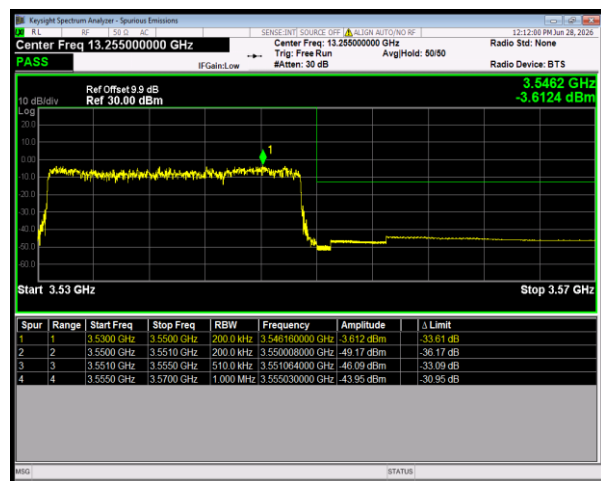
n77(3450-3550) SCS=30kHz DFT_QPSK BW=20MHz HighChannel=636000 RB=50@0
