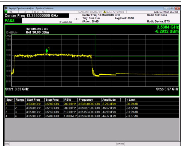
n77(3450-3550) SCS=30kHz CP_16QAM BW=20MHz HighChannel=636000 RB=51@0
