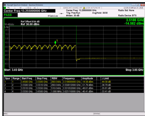
n77(3450-3550) SCS=30kHz CP_QPSK BW=100MHz HighChannel=633334 RB=273@0
