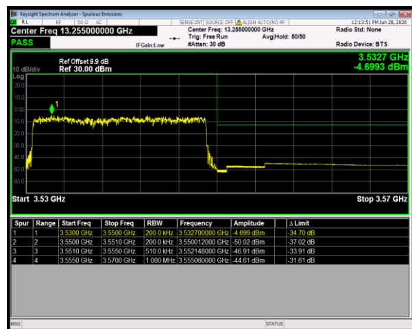
n77(3450-3550) SCS=30kHz DFT_16QAM BW=20MHz HighChannel=636000 RB=50@0
