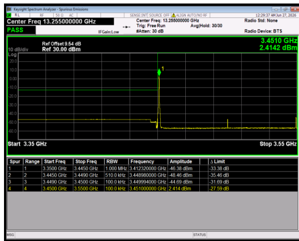
n77(3450-3550) SCS=30kHz CP_QPSK BW=100MHz LowChannel=633334 RB=1@0
