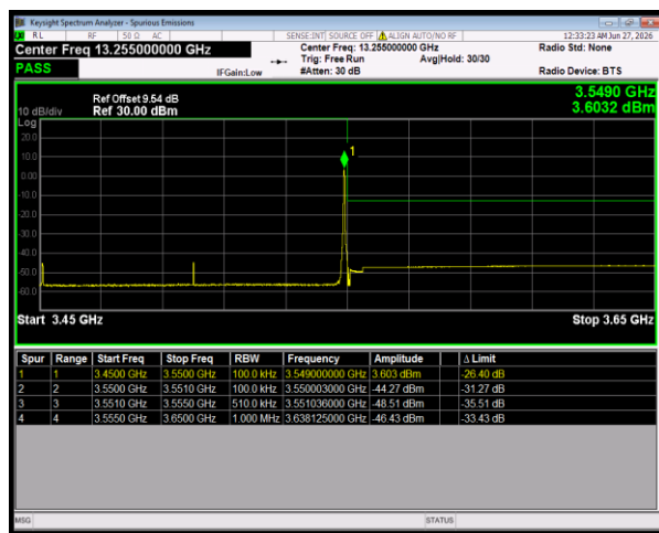
n77(3450-3550) SCS=30kHz DFT_QPSK BW=100MHz HighChannel=633334 RB=1@272
