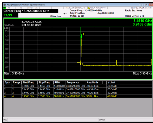
n77(3450-3550) SCS=30kHz DFT_QPSK BW=100MHz LowChannel=633334 RB=1@0
