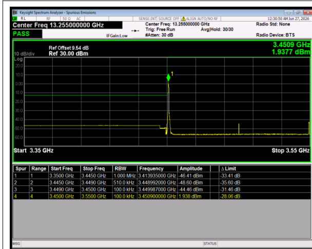
n77(3450-3550) SCS=30kHz CP_16QAM BW=100MHz LowChannel=633334 RB=1@0
