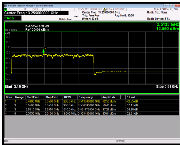
n77(3450-3550) SCS=30kHz CP_16QAM BW=60MHz HighChannel=634666 RB=162@0
