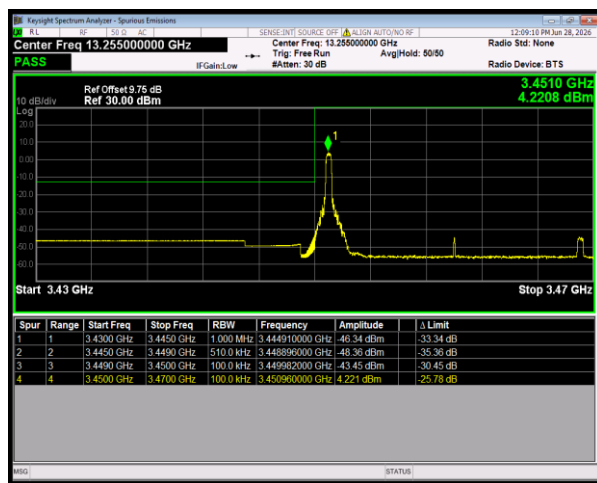
n77(3450-3550) SCS=30kHz CP_16QAM BW=20MHz LowChannel=630668 RB=1@0
