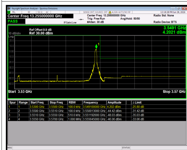
n77(3450-3550) SCS=30kHz CP_16QAM BW=20MHz HighChannel=636000 RB=1@50
