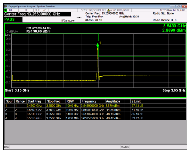
n77(3450-3550) SCS=30kHz DFT_BPSK BW=100MHz HighChannel=633334 RB=1@272
