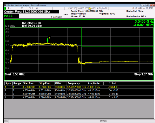
n77(3450-3550) SCS=30kHz DFT_BPSK BW=20MHz HighChannel=636000 RB=50@0
