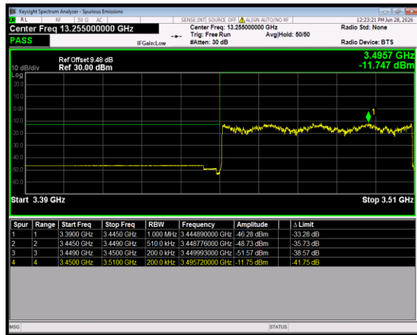
n77(3450-3550) SCS=30kHz DFT_16QAM BW=60MHz LowChannel=632000 RB=162@0
