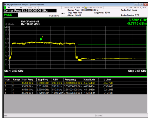
n77(3450-3550) SCS=30kHz CP_QPSK BW=20MHz HighChannel=636000 RB=51@0
