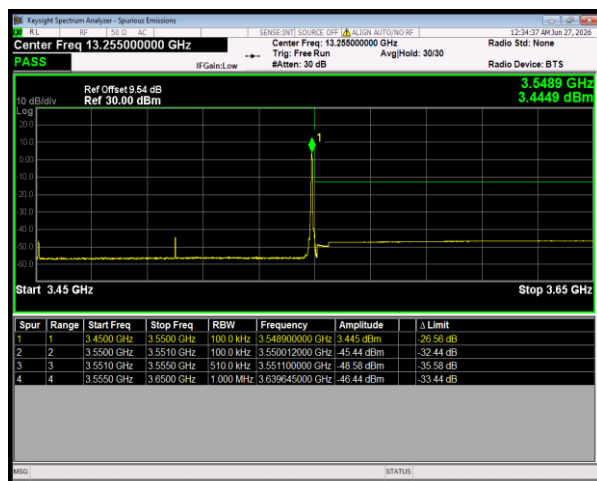
n77(3450-3550) SCS=30kHz DFT_16QAM BW=100MHz HighChannel=633334 RB=1@272
