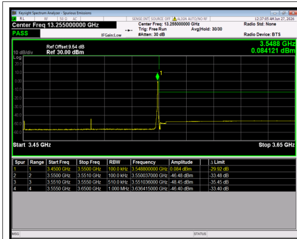
n77(3450-3550) SCS=30kHz CP_16QAM BW=100MHz HighChannel=633334 RB=1@272
