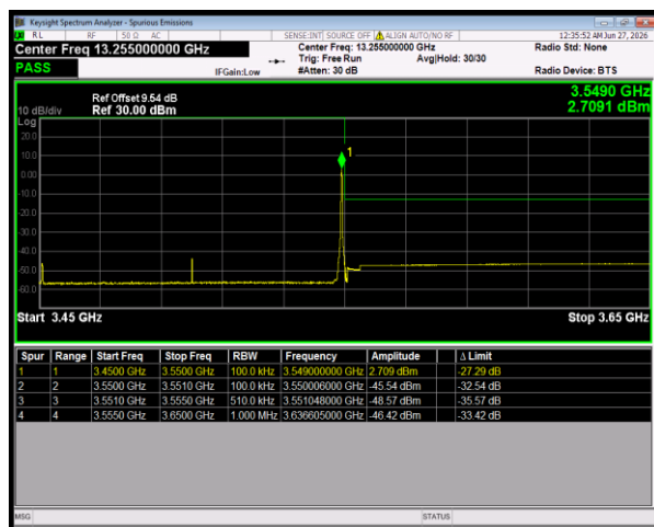
n77(3450-3550) SCS=30kHz CP_QPSK BW=100MHz HighChannel=633334 RB=1@272
