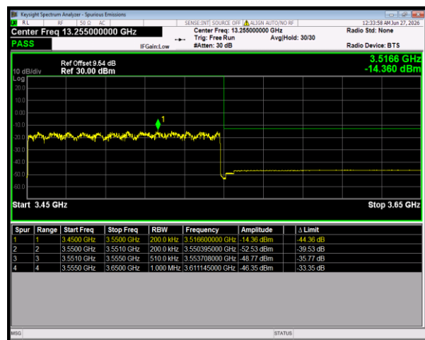
n77(3450-3550) SCS=30kHz DFT_16QAM BW=100MHz HighChannel=633334 RB=270@0
