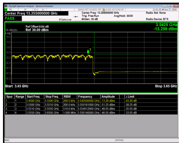
n77(3450-3550) SCS=30kHz DFT_BPSK BW=100MHz HighChannel=633334 RB=270@0
