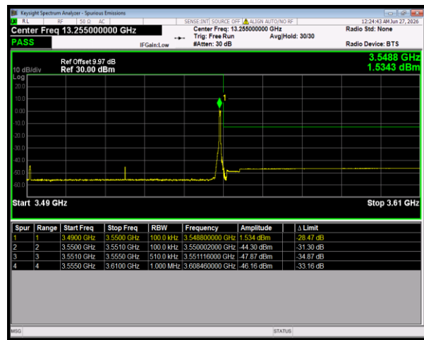
n77(3450-3550) SCS=30kHz CP_16QAM BW=60MHz HighChannel=634666 RB=1@161
