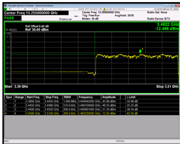
n77(3450-3550) SCS=30kHz CP_16QAM BW=60MHz LowChannel=632000 RB=162@0
