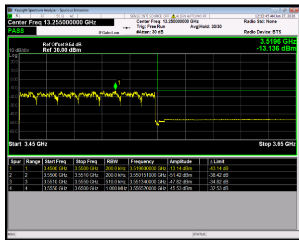
n77(3450-3550) SCS=30kHz DFT_QPSK BW=100MHz HighChannel=633334 RB=270@0
