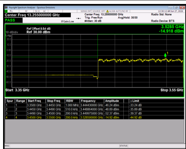
n77(3450-3550) SCS=30kHz CP_16QAM BW=100MHz LowChannel=633334 RB=273@0
