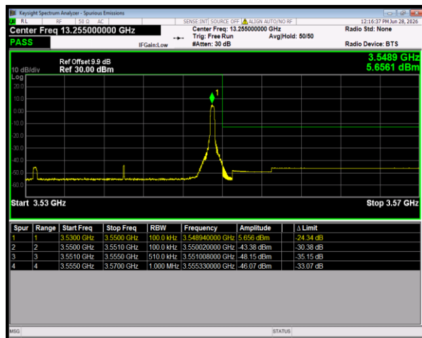
n77(3450-3550) SCS=30kHz CP_QPSK BW=20MHz HighChannel=636000 RB=1@50
