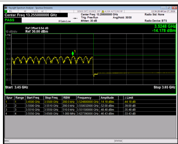
n77(3450-3550) SCS=30kHz CP_16QAM BW=100MHz HighChannel=633334 RB=273@0
