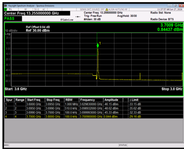
n78(3700-3800) SCS=30kHz CP_16QAM BW=100MHz LowChannel=650000 RB=1@0
