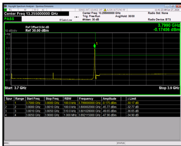
n78(3700-3800) SCS=30kHz DFT_QPSK BW=100MHz HighChannel=650000 RB=1@272
