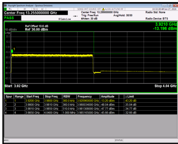
n77(3700-3980) SCS=30kHz DFT_QPSK BW=60MHz HighChannel=663332 RB=162@0
