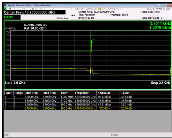
n78(3700-3800) SCS=30kHz DFT_BPSK BW=100MHz LowChannel=650000 RB=1@0
