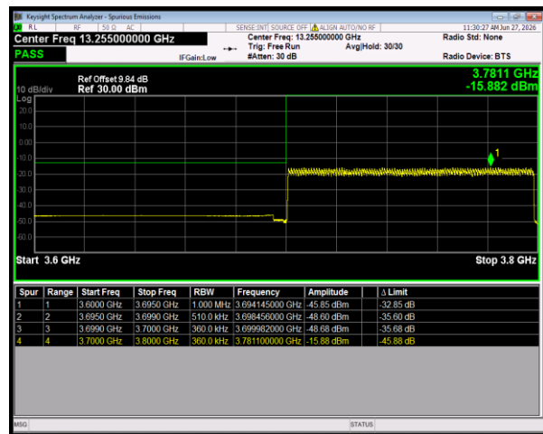
n78(3700-3800) SCS=30kHz DFT_BPSK BW=100MHz LowChannel=650000 RB=270@0
