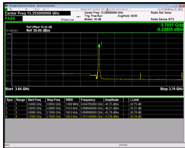
n78(3700-3800) SCS=30kHz DFT_16QAM BW=60MHz LowChannel=648668 RB=1@0
