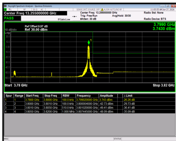
n78(3700-3800) SCS=30kHz DFT_BPSK BW=20MHz HighChannel=652666 RB=1@50
