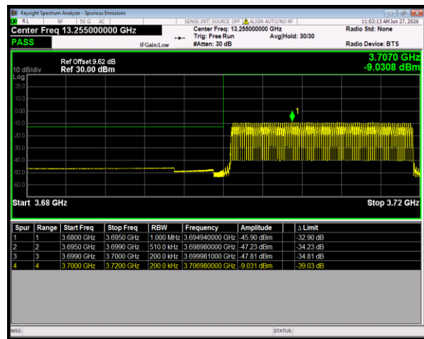
n78(3700-3800) SCS=30kHz CP_16QAM BW=20MHz LowChannel=647334 RB=51@0
