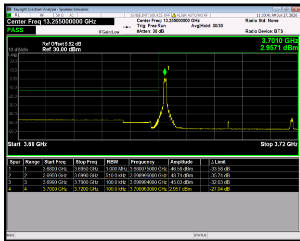
n78(3700-3800) SCS=30kHz DFT_16QAM BW=20MHz LowChannel=647334 RB=1@0
