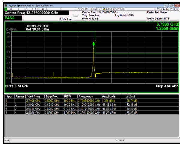
n78(3700-3800) SCS=30kHz DFT_BPSK BW=60MHz HighChannel=651332 RB=1@161
