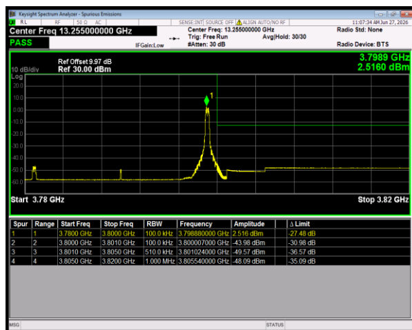
n78(3700-3800) SCS=30kHz DFT_QPSK BW=20MHz HighChannel=652666 RB=1@50
