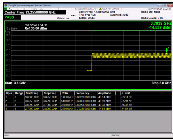
n78(3700-3800) SCS=30kHz CP_16QAM BW=100MHz LowChannel=650000 RB=273@0
