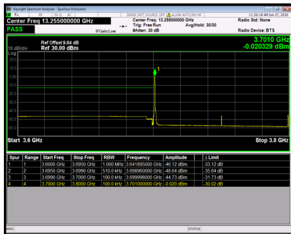
n78(3700-3800) SCS=30kHz CP_QPSK BW=100MHz LowChannel=650000 RB=1@0
