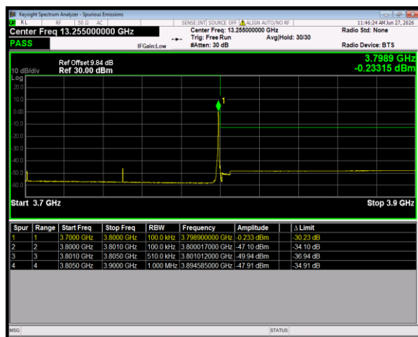
n78(3700-3800) SCS=30kHz CP_16QAM BW=100MHz HighChannel=650000 RB=1@272
