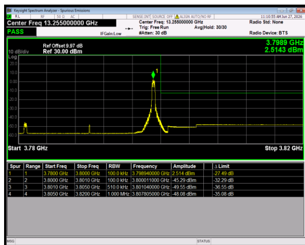
n78(3700-3800) SCS=30kHz CP_QPSK BW=20MHz HighChannel=652666 RB=1@50
