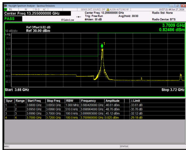
n78(3700-3800) SCS=30kHz DFT_BPSK BW=20MHz LowChannel=647334 RB=1@0
