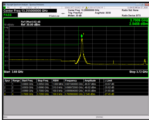
n78(3700-3800) SCS=30kHz CP_16QAM BW=20MHz LowChannel=647334 RB=1@0
