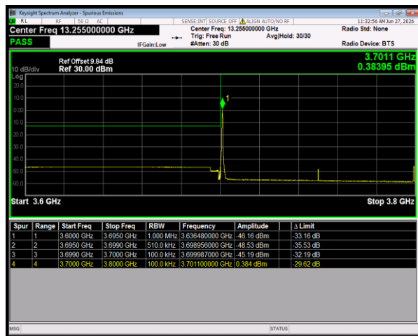
n78(3700-3800) SCS=30kHz DFT_QPSK BW=100MHz LowChannel=650000 RB=1@0
