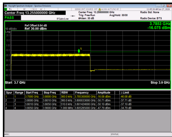
n78(3700-3800) SCS=30kHz CP_16QAM BW=100MHz HighChannel=650000 RB=273@0
