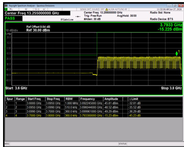
n78(3700-3800) SCS=30kHz DFT_QPSK BW=100MHz LowChannel=650000 RB=270@0
