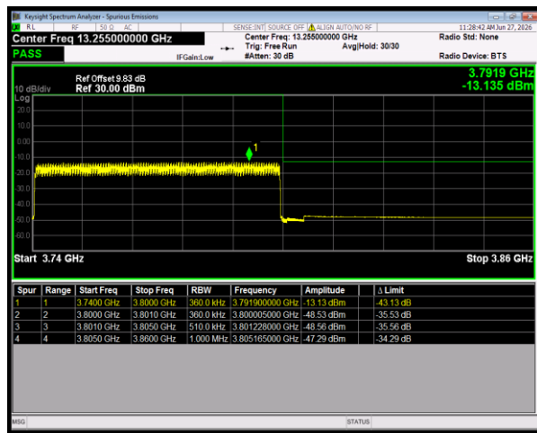
n78(3700-3800) SCS=30kHz CP_16QAM BW=60MHz HighChannel=651332 RB=162@0
