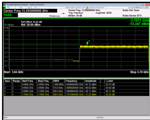
n78(3700-3800) SCS=30kHz DFT_BPSK BW=60MHz LowChannel=648668 RB=162@0
