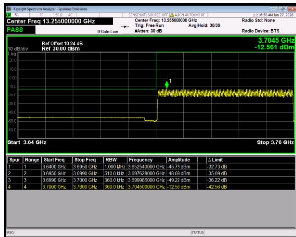
n78(3700-3800) SCS=30kHz DFT_16QAM BW=60MHz LowChannel=648668 RB=162@0
