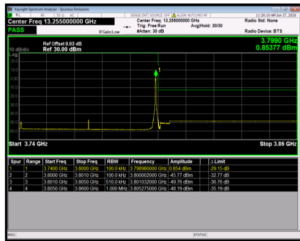
n78(3700-3800) SCS=30kHz DFT_16QAM BW=60MHz HighChannel=651332 RB=1@161
