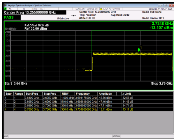
n78(3700-3800) SCS=30kHz CP_16QAM BW=60MHz LowChannel=648668 RB=162@0
