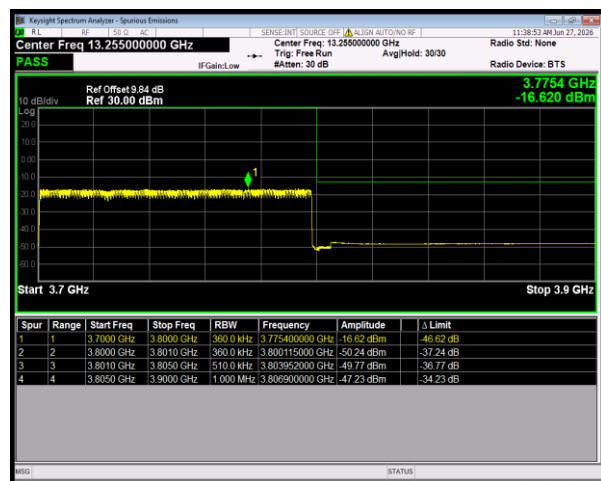
n78(3700-3800) SCS=30kHz DFT_BPSK BW=100MHz HighChannel=650000 RB=270@0
