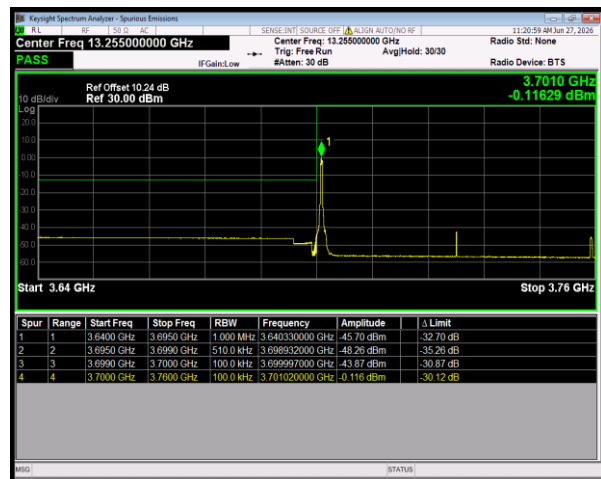
n78(3700-3800) SCS=30kHz CP_16QAM BW=60MHz LowChannel=648668 RB=1@0
