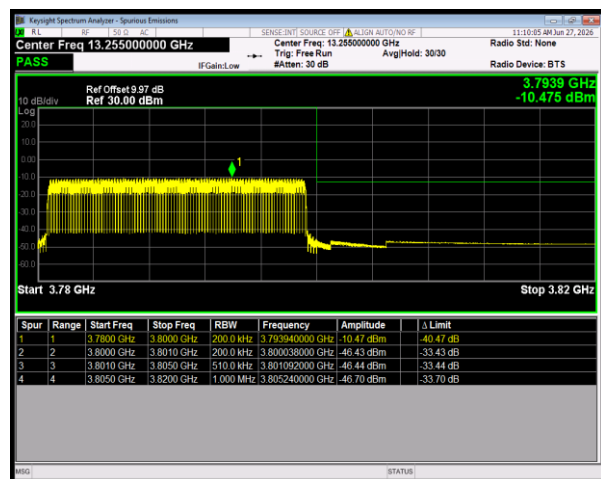
n78(3700-3800) SCS=30kHz CP_QPSK BW=20MHz HighChannel=652666 RB=51@0
