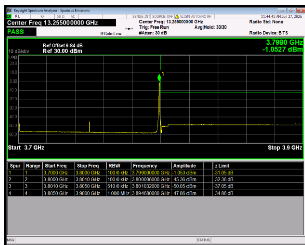
n78(3700-3800) SCS=30kHz CP_QPSK BW=100MHz HighChannel=650000 RB=1@272
