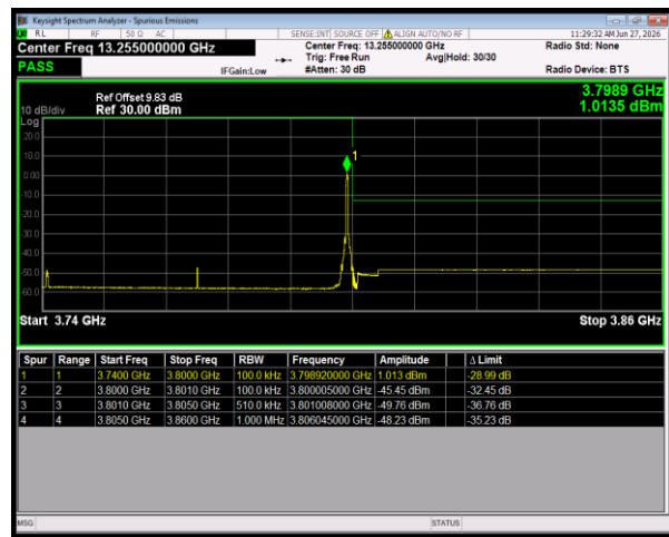
n78(3700-3800) SCS=30kHz CP_16QAM BW=60MHz HighChannel=651332 RB=1@161
