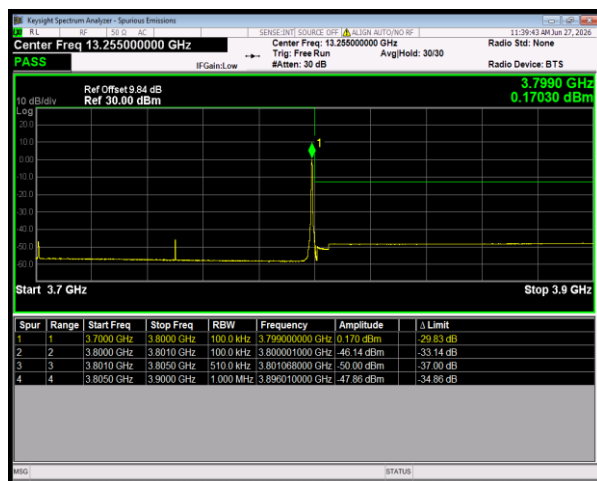
n78(3700-3800) SCS=30kHz DFT_BPSK BW=100MHz HighChannel=650000 RB=1@272
