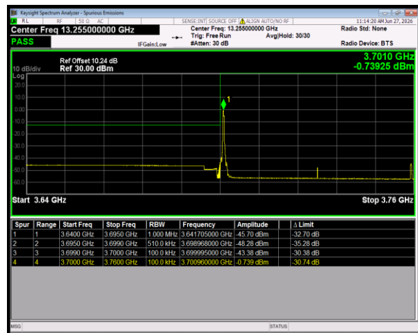
n78(3700-3800) SCS=30kHz DFT_BPSK BW=60MHz LowChannel=648668 RB=1@0
