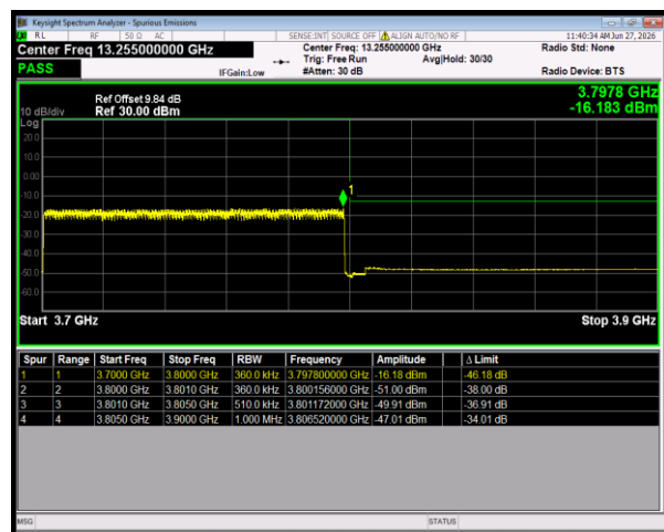
n78(3700-3800) SCS=30kHz DFT_QPSK BW=100MHz HighChannel=650000 RB=270@0
