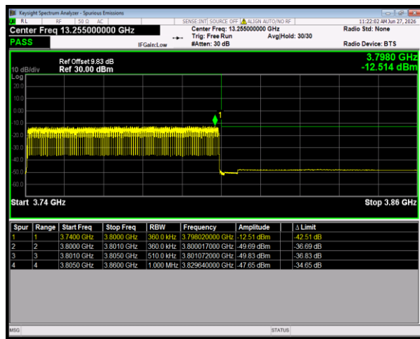
n78(3700-3800) SCS=30kHz DFT_BPSK BW=60MHz HighChannel=651332 RB=162@0
