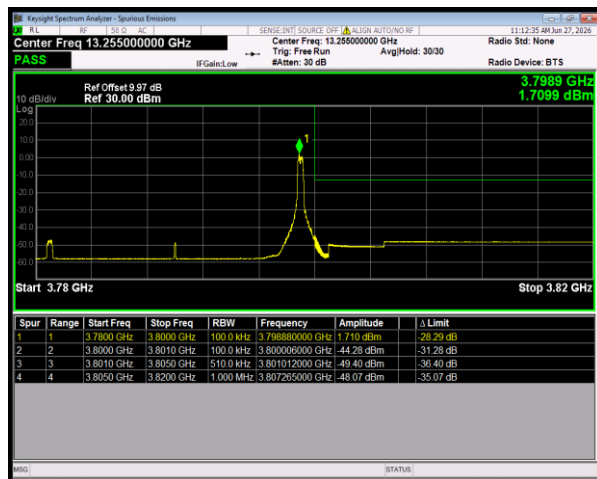
n78(3700-3800) SCS=30kHz CP_16QAM BW=20MHz HighChannel=652666 RB=1@50
