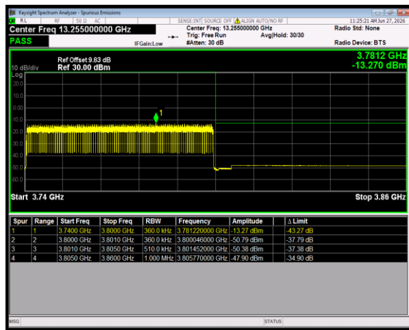
n78(3700-3800) SCS=30kHz DFT_16QAM BW=60MHz HighChannel=651332 RB=162@0
