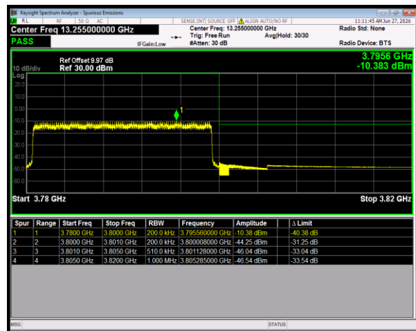
n78(3700-3800) SCS=30kHz CP_16QAM BW=20MHz HighChannel=652666 RB=51@0
