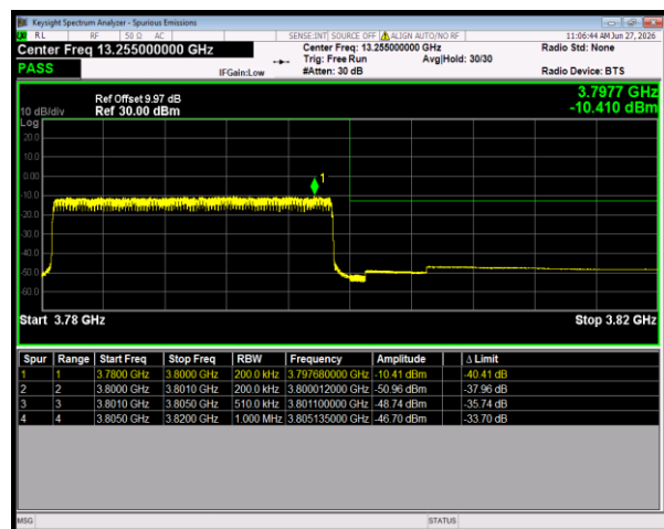
n78(3700-3800) SCS=30kHz DFT_QPSK BW=20MHz HighChannel=652666 RB=50@0
