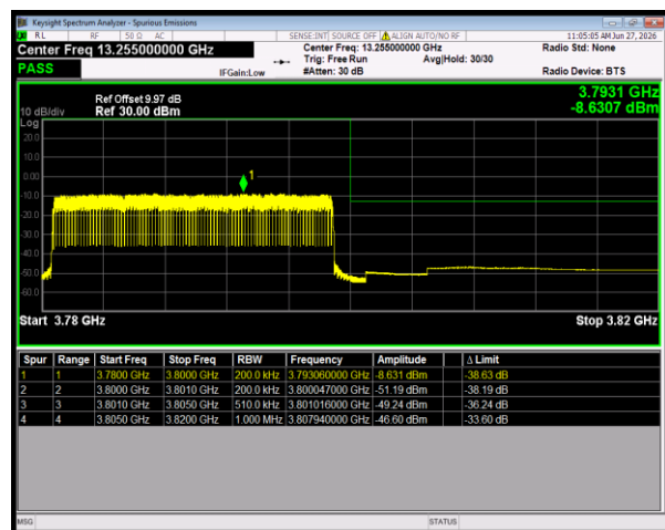
n78(3700-3800) SCS=30kHz DFT_BPSK BW=20MHz HighChannel=652666 RB=50@0
