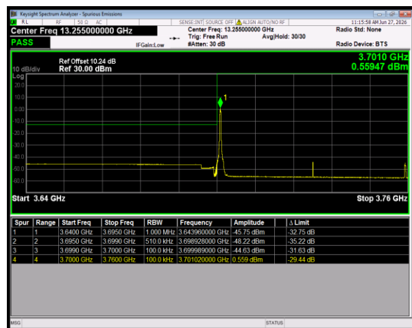
n78(3700-3800) SCS=30kHz DFT_QPSK BW=60MHz LowChannel=648668 RB=1@0
