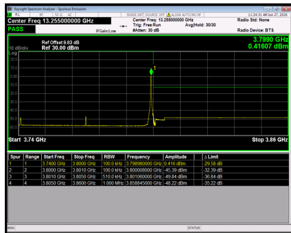
n78(3700-3800) SCS=30kHz DFT_QPSK BW=60MHz HighChannel=651332 RB=1@161
