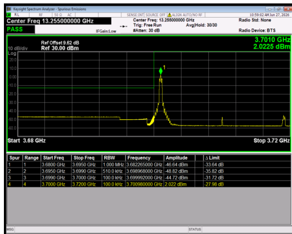
n78(3700-3800) SCS=30kHz DFT_QPSK BW=20MHz LowChannel=647334 RB=1@0
