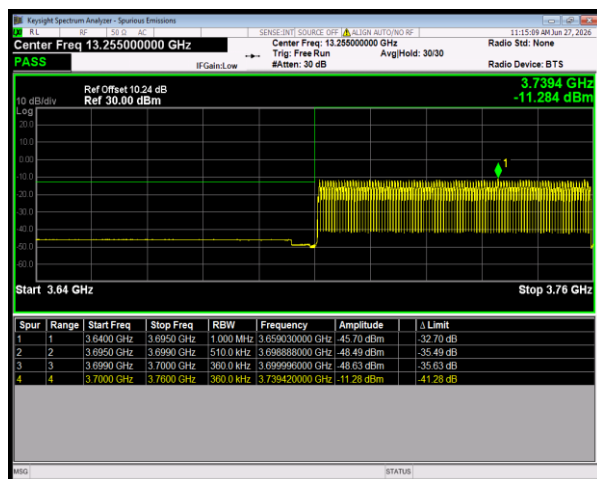
n78(3700-3800) SCS=30kHz DFT_QPSK BW=60MHz LowChannel=648668 RB=162@0
