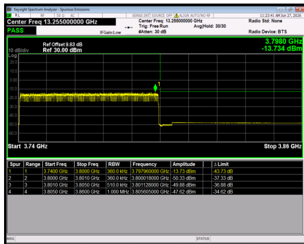
n78(3700-3800) SCS=30kHz DFT_QPSK BW=60MHz HighChannel=651332 RB=162@0
