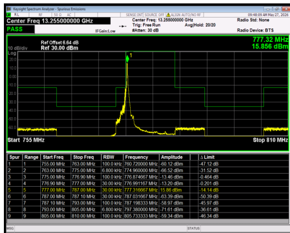
n13 SCS=15kHz DFT_BPSK BW=5MHz LowChannel=155900 RB=1@0
