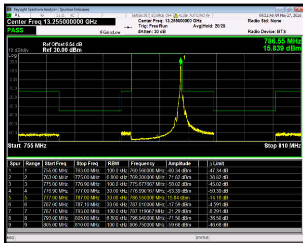
n13 SCS=15kHz DFT_QPSK BW=10MHz HighChannel=156400 RB=1@51
