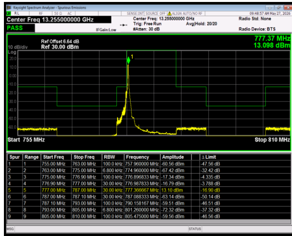
n13 SCS=15kHz CP_QPSK BW=5MHz LowChannel=155900 RB=1@0
