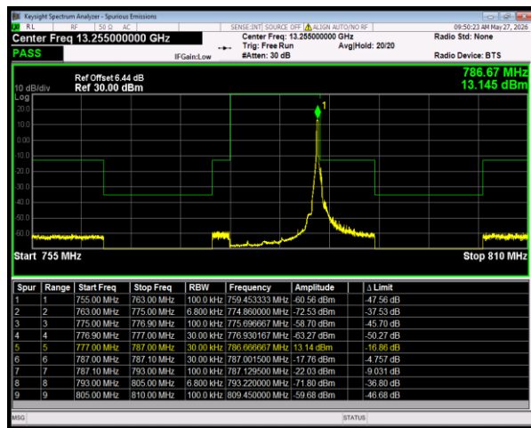
n13 SCS=15kHz CP_QPSK BW=5MHz HighChannel=156900 RB=1@24
