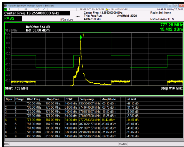
n13 SCS=15kHz DFT_16QAM BW=5MHz LowChannel=155900 RB=1@0
