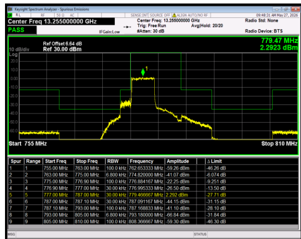
n13 SCS=15kHz DFT_16QAM BW=5MHz LowChannel=155900 RB=25@0
