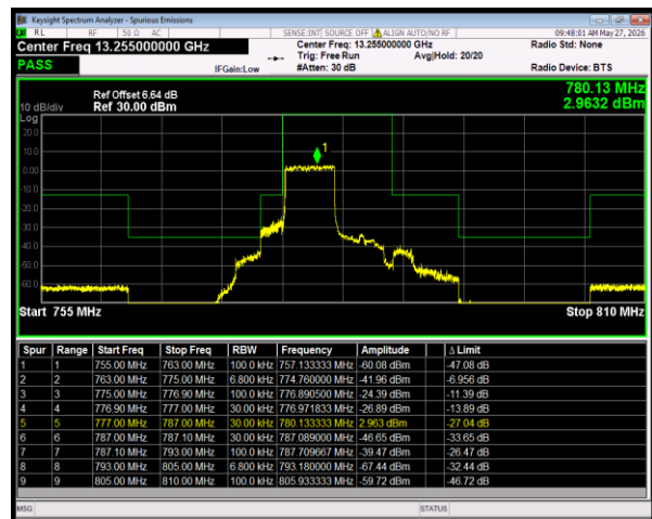
n13 SCS=15kHz DFT_BPSK BW=5MHz LowChannel=155900 RB=25@0
