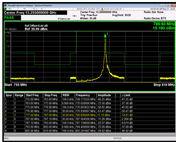
n13 SCS=15kHz DFT_16QAM BW=5MHz HighChannel=156900 RB=1@24
