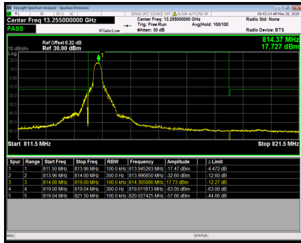
n26(814-824) SCS=15kHz CP_QPSK BW=5MHz LowChannel=163300 RB=1@0
