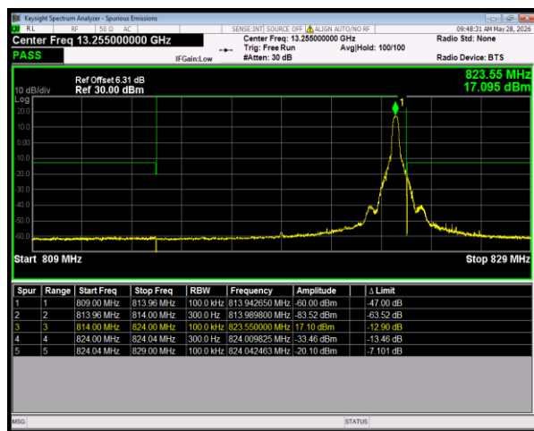
n26(814-824) SCS=15kHz CP_QPSK BW=10MHz HighChannel=163800 RB=1@51
