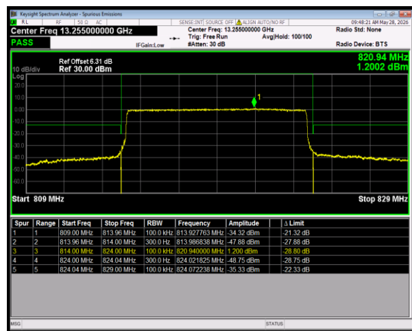
n26(814-824) SCS=15kHz CP_QPSK BW=10MHz HighChannel=163800 RB=52@0
