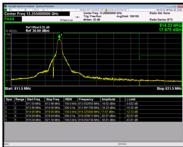
n26(814-824) SCS=15kHz CP_16QAM BW=5MHz LowChannel=163300 RB=1@0
