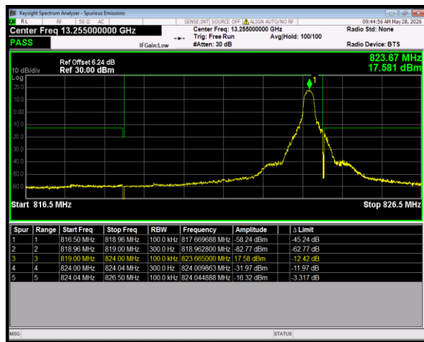
n26(814-824) SCS=15kHz CP_QPSK BW=5MHz HighChannel=164300 RB=1@24
