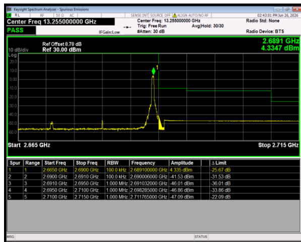
n41 SCS=30kHz DFT_16QAM BW=20MHz HighChannel=535998 RB=1@50
