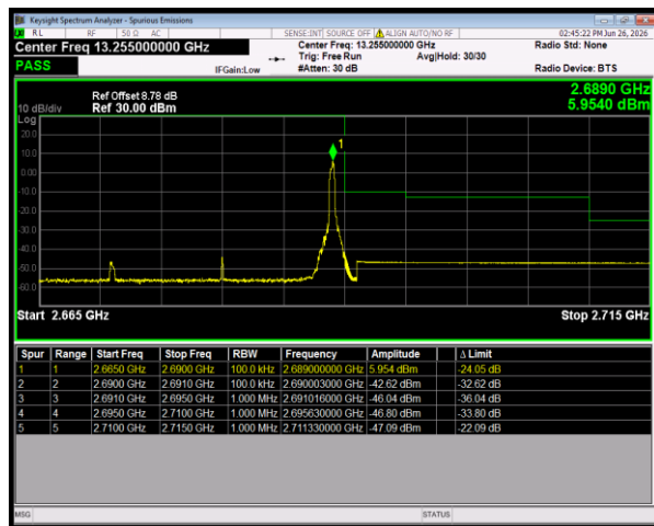
n41 SCS=30kHz CP_16QAM BW=20MHz HighChannel=535998 RB=1@50
