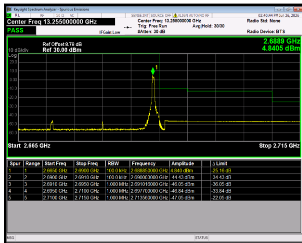
n41 SCS=30kHz DFT_BPSK BW=20MHz HighChannel=535998 RB=1@50
