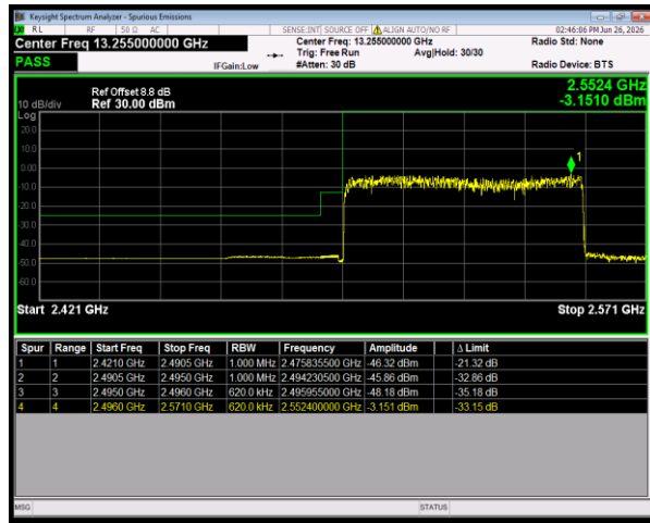
n41 SCS=30kHz DFT_BPSK BW=60MHz LowChannel=505200 RB=162@0
