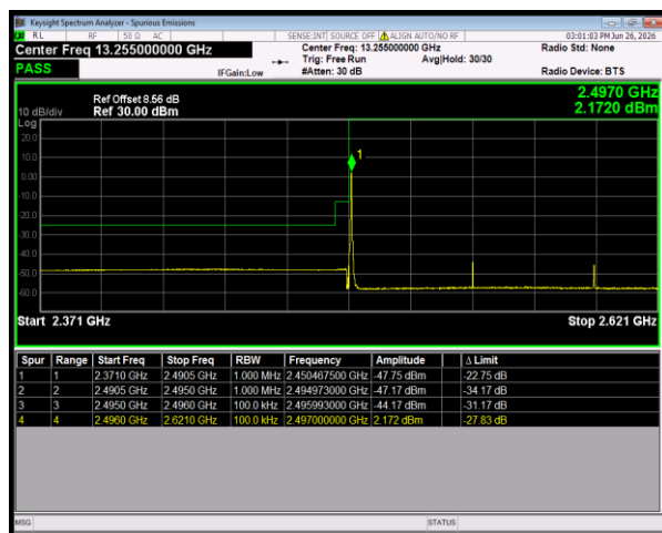
n41 SCS=30kHz CP_QPSK BW=100MHz LowChannel=509202 RB=1@0
