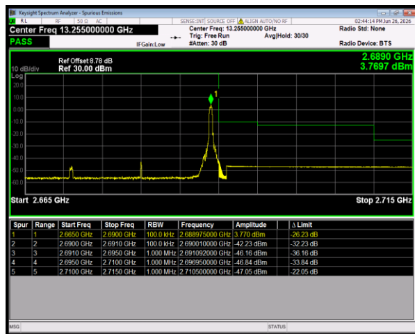
n41 SCS=30kHz CP_QPSK BW=20MHz HighChannel=535998 RB=1@50
