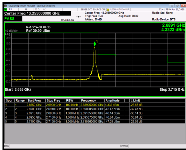
n41 SCS=30kHz DFT_QPSK BW=20MHz HighChannel=535998 RB=1@50
