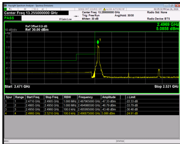
n41 SCS=30kHz DFT_BPSK BW=20MHz LowChannel=501204 RB=1@0
