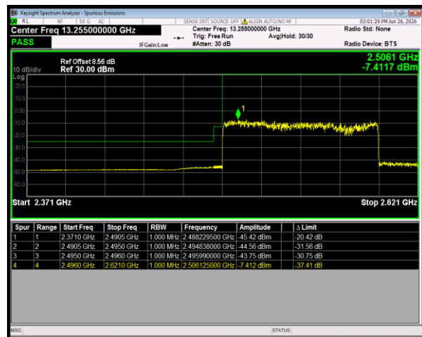
n41 SCS=30kHz CP_16QAM BW=100MHz LowChannel=509202 RB=273@0
