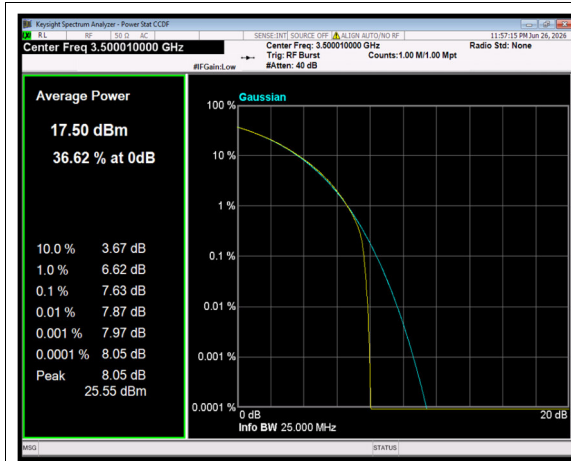
n77(3450-3550) SCS=30kHz CP_16QAM BW=20MHz Channel=633334 RB=51@0
