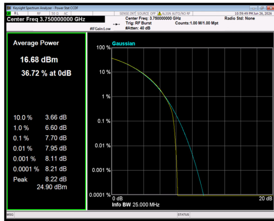
n78(3700-3800) SCS=30kHz CP_16QAM BW=20MHz Channel=650000 RB=51@0
