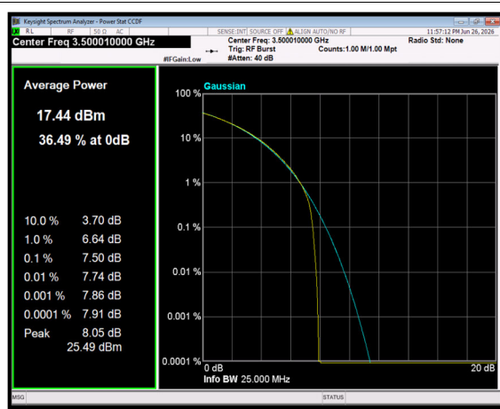
n77(3450-3550) SCS=30kHz CP_QPSK BW=20MHz Channel=633334 RB=51@0
