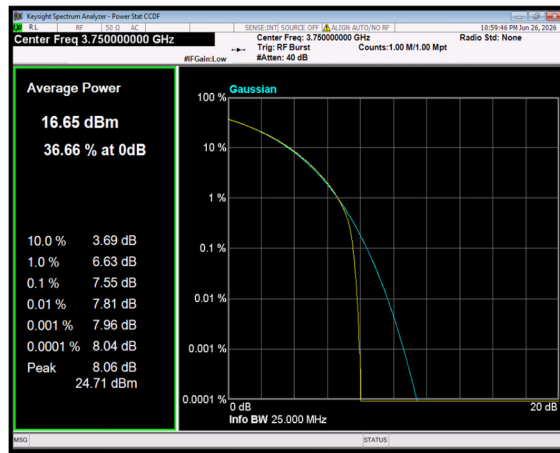
n78(3700-3800) SCS=30kHz CP_QPSK BW=20MHz Channel=650000 RB=51@0
