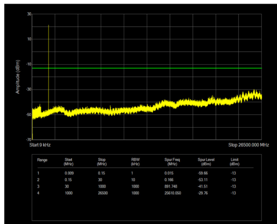
n2 SCS=15kHz DFT_QPSK BW=20MHz Channel=376000 RB=1@105
