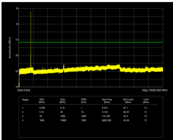
n5 SCS=15kHz DFT_QPSK BW=5MHz Channel=165300 RB=1@24
