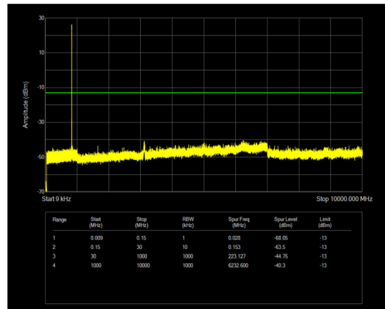
n5 SCS=15kHz DFT_QPSK BW=5MHz Channel=165300 RB=1@0
