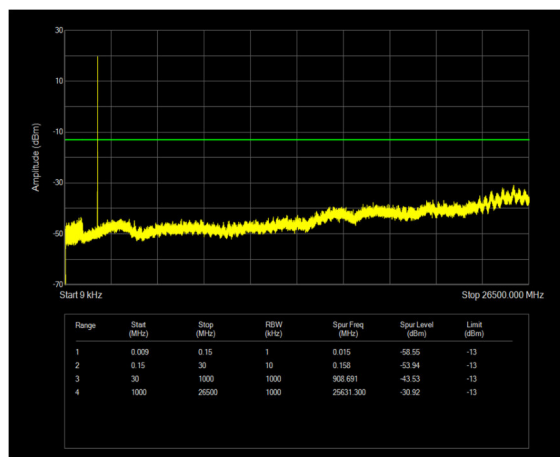
n2 SCS=15kHz CP_QPSK BW=10MHz Channel=371000 RB=1@51
