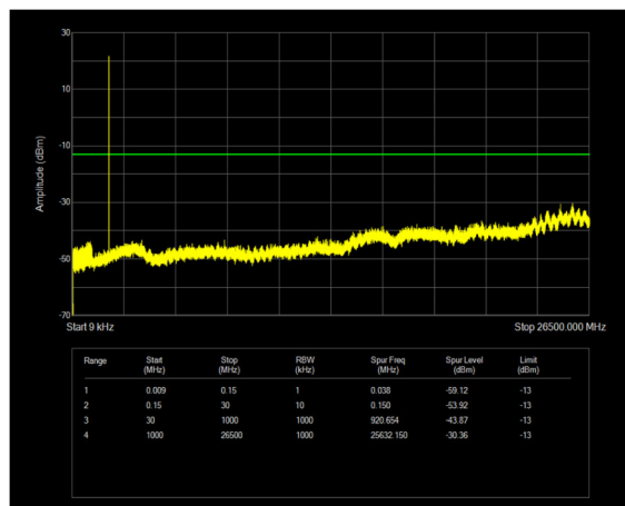
n2 SCS=15kHz DFT_QPSK BW=20MHz Channel=372000 RB=1@105
