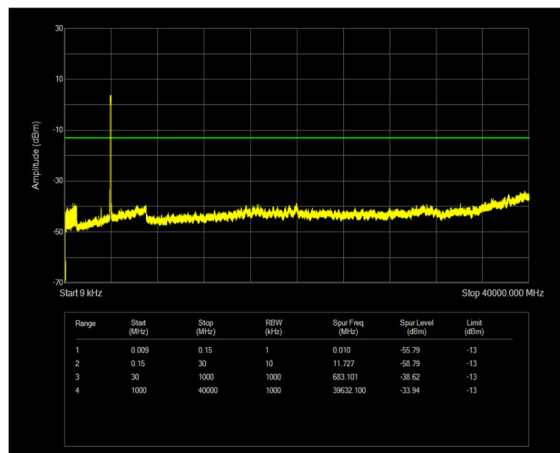
n77(3700-3980) SCS=30kHz DFT_QPSK BW=100MHz Channel=662000 RB=270@0
