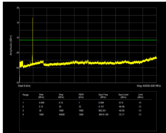
n77(3700-3980) SCS=30kHz DFT_QPSK BW=100MHz Channel=650000 RB=1@272
