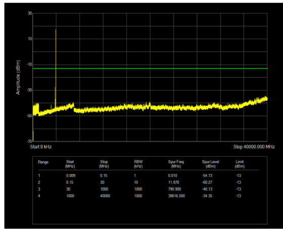
n77(3700-3980) SCS=30kHz DFT_QPSK BW=100MHz Channel=656000 RB=1@272
