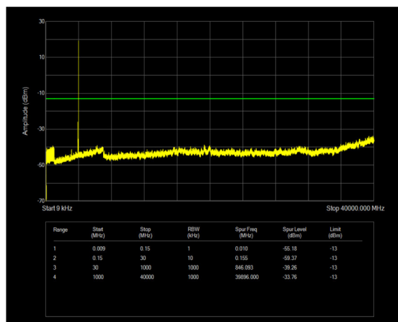
n77(3700-3980) SCS=30kHz CP_QPSK BW=100MHz Channel=662000 RB=1@272
