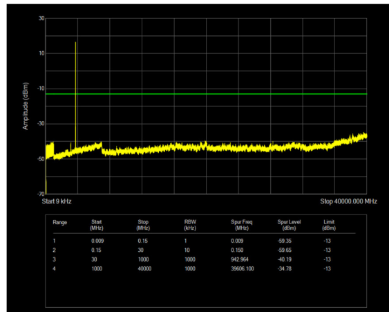
n77(3700-3980) SCS=30kHz CP_QPSK BW=20MHz Channel=647334 RB=1@50
