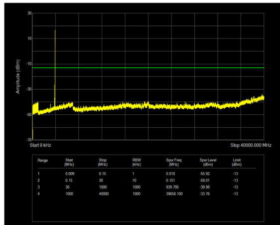
n77(3700-3980) SCS=30kHz CP_QPSK BW=100MHz Channel=656000 RB=1@272
