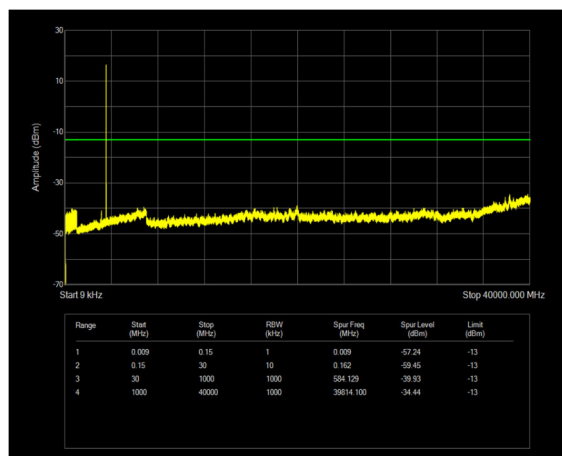
n77(3450-3550) SCS=30kHz DFT_QPSK BW=20MHz Channel=636000 RB=1@0
