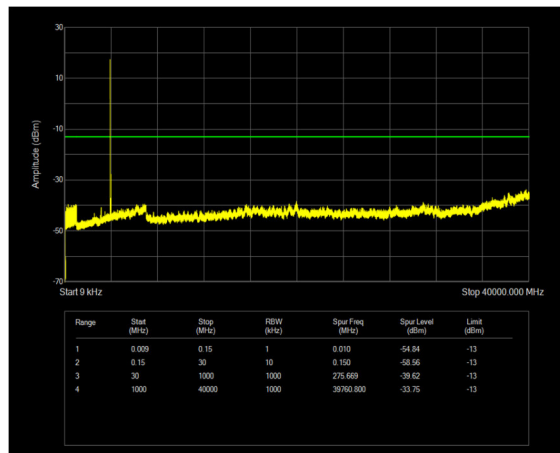
n77(3700-3980) SCS=30kHz DFT_QPSK BW=100MHz Channel=662000 RB=1@0
