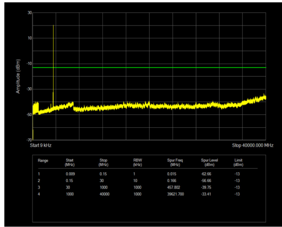
n77(3450-3550) SCS=30kHz CP_QPSK BW=60MHz Channel=634666 RB=1@161
