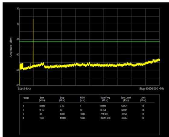
n77(3700-3980) SCS=30kHz CP_QPSK BW=60MHz Channel=656000 RB=1@161
