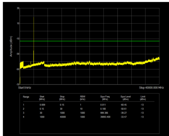
n77(3700-3980) SCS=30kHz CP_QPSK BW=60MHz Channel=663332 RB=1@161
