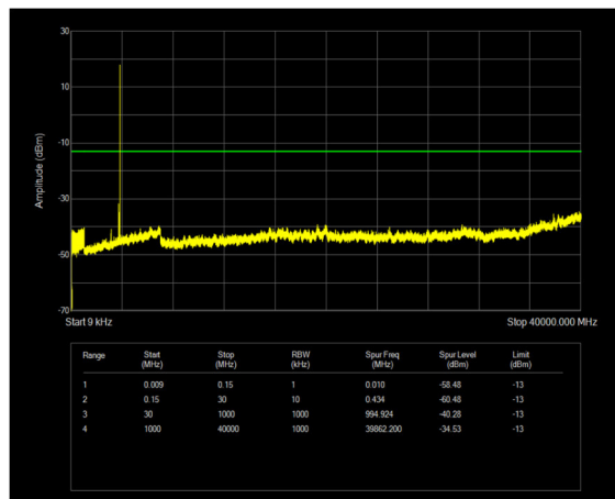
n77(3700-3980) SCS=30kHz CP_QPSK BW=100MHz Channel=650000 RB=1@272
