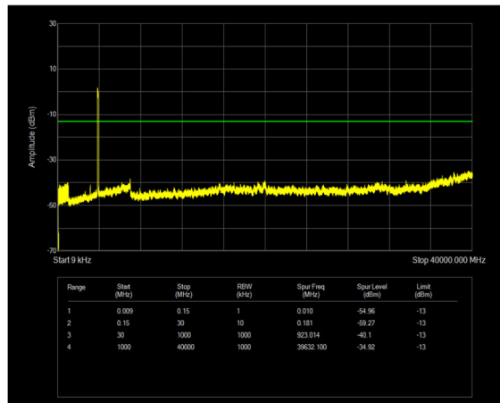
n77(3700-3980) SCS=30kHz CP_QPSK BW=100MHz Channel=656000 RB=273@0
