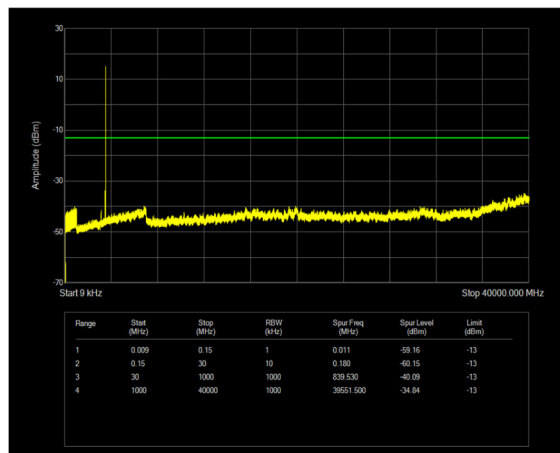
n77(3450-3550) SCS=30kHz DFT_QPSK BW=60MHz Channel=632000 RB=1@161
