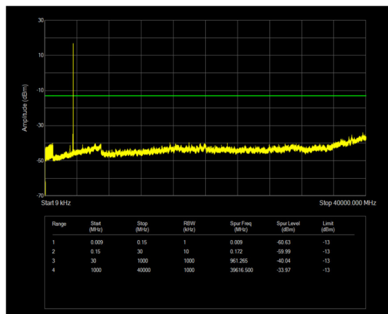
n77(3450-3550) SCS=30kHz DFT_QPSK BW=60MHz Channel=633334 RB=1@161
