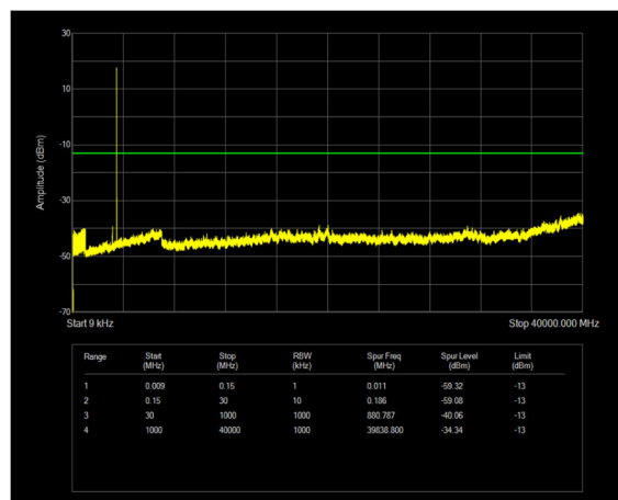
n77(3450-3550) SCS=30kHz DFT_QPSK BW=20MHz Channel=630668 RB=1@0
