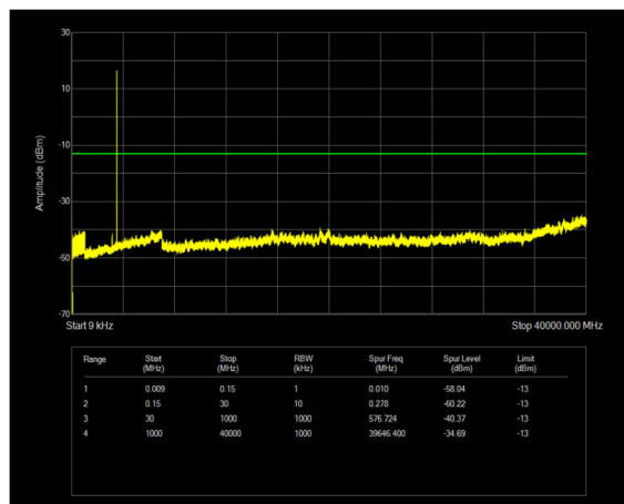
n77(3450-3550) SCS=30kHz DFT_QPSK BW=20MHz Channel=633334 RB=1@0
