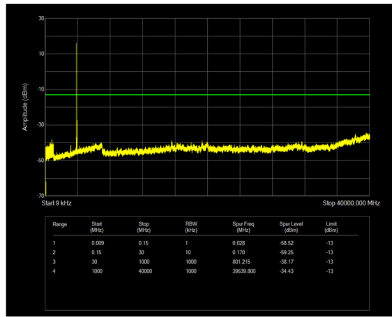
n77(3700-3980) SCS=30kHz DFT_QPSK BW=100MHz Channel=656000 RB=1@0
