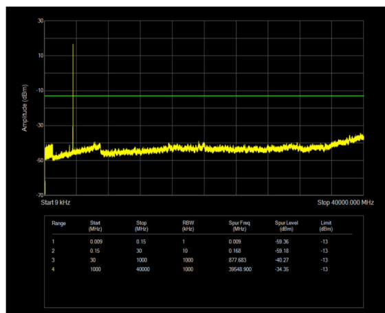
n77(3450-3550) SCS=30kHz DFT_QPSK BW=20MHz Channel=636000 RB=1@50
