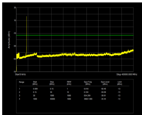
n77(3450-3550) SCS=30kHz DFT_QPSK BW=20MHz Channel=630668 RB=1@50
