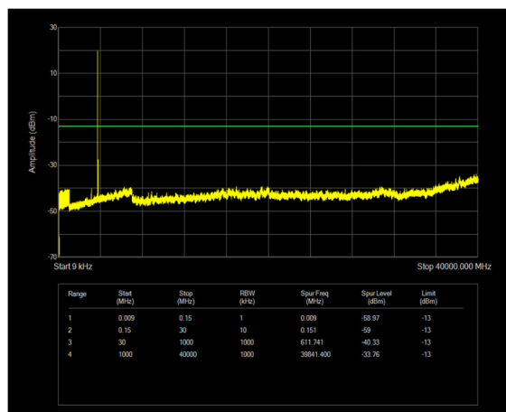
n77(3700-3980) SCS=30kHz CP_QPSK BW=60MHz Channel=648668 RB=1@0
