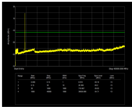
n77(3450-3550) SCS=30kHz CP_QPSK BW=60MHz Channel=634666 RB=1@0
