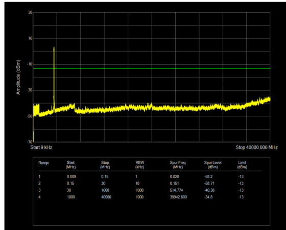
n77(3450-3550) SCS=30kHz DFT_QPSK BW=100MHz Channel=633334 RB=270@0
