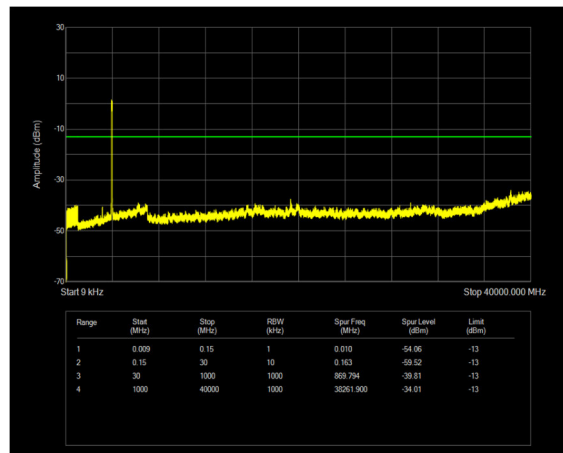
n77(3700-3980) SCS=30kHz CP_QPSK BW=100MHz Channel=662000 RB=273@0
