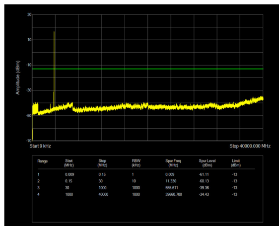
n77(3700-3980) SCS=30kHz CP_QPSK BW=60MHz Channel=648668 RB=1@161
