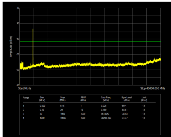
n77(3700-3980) SCS=30kHz DFT_QPSK BW=100MHz Channel=650000 RB=270@0
