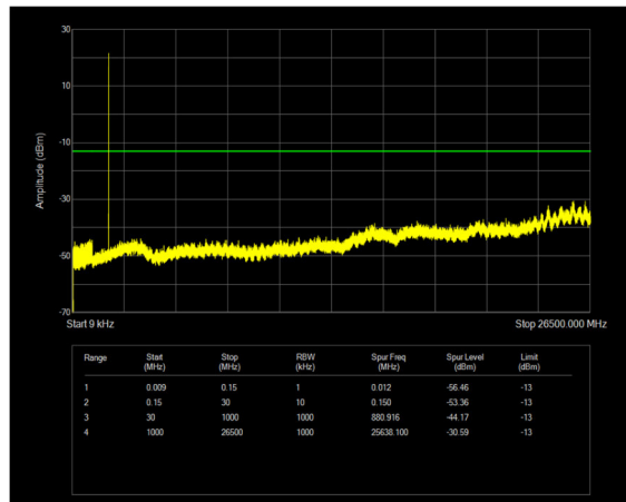
n25 SCS=15kHz DFT_QPSK BW=5MHz Channel=370500 RB=1@24
