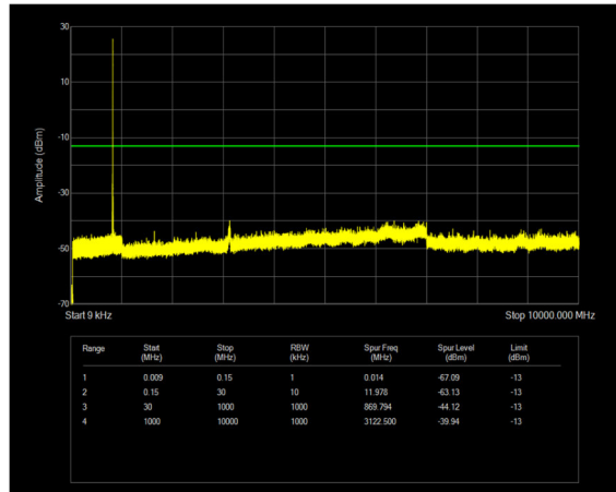
n26(814-824) SCS=15kHz CP_QPSK BW=5MHz Channel=163300 RB=1@24
