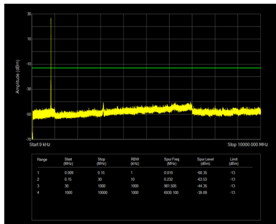
n26(824-849) SCS=15kHz CP_QPSK BW=5MHz Channel=165300 RB=1@24
