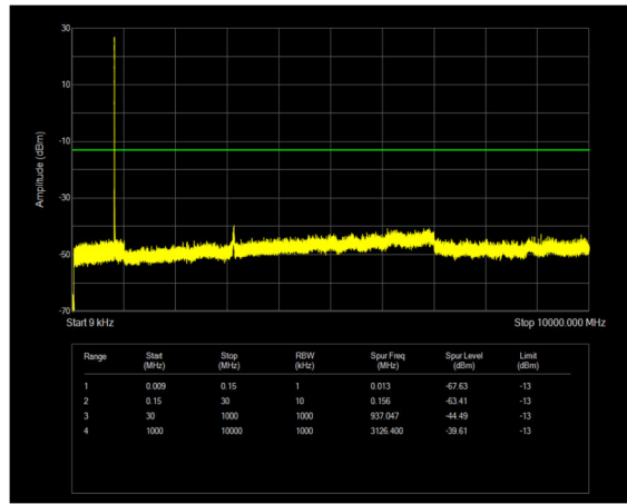
n26(814-824) SCS=15kHz CP_QPSK BW=5MHz Channel=163300 RB=1@0
