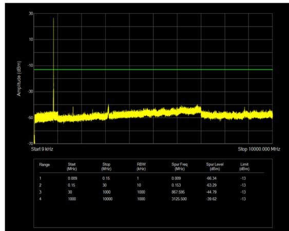
n26(814-824) SCS=15kHz DFT_QPSK BW=5MHz Channel=163300 RB=1@24
