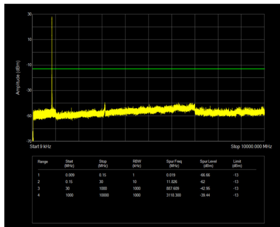
n26(824-849) SCS=15kHz DFT_QPSK BW=5MHz Channel=167300 RB=1@24
