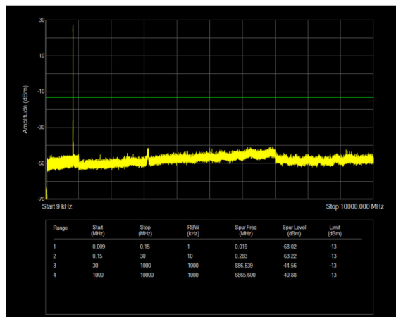
n26(824-849) SCS=15kHz DFT_QPSK BW=5MHz Channel=165300 RB=1@24
