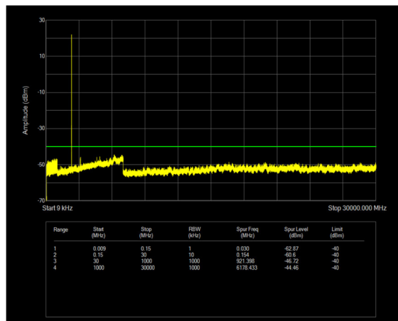
n30 SCS=15kHz CP_QPSK BW=5MHz Channel=461500 RB=1@0
