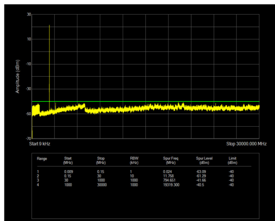
n30 SCS=15kHz CP_QPSK BW=5MHz Channel=461500 RB=1@24
