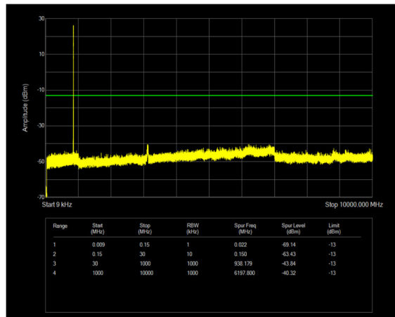
n26(824-849) SCS=15kHz DFT_QPSK BW=5MHz Channel=169300 RB=1@24
