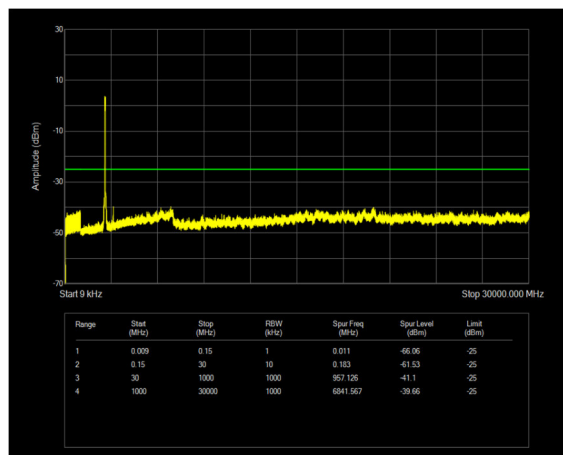
n41 SCS=30kHz CP_QPSK BW=60MHz Channel=518598 RB=162@0
