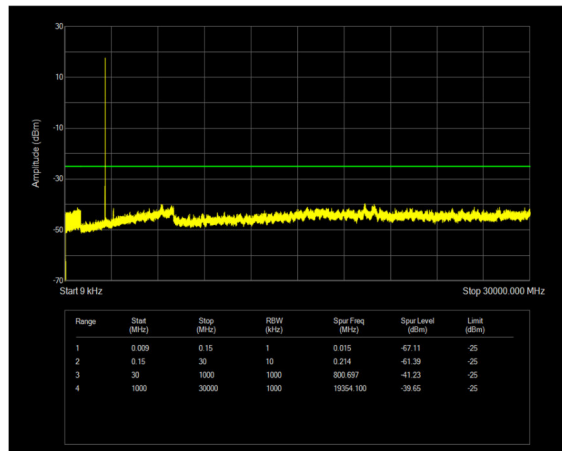
n38 SCS=30kHz DFT_QPSK BW=20MHz Channel=516000 RB=1@50
