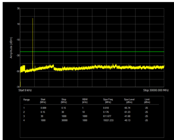
n38 SCS=30kHz CP_QPSK BW=40MHz Channel=520000 RB=1@105
