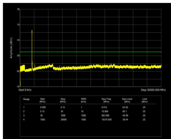
n41 SCS=30kHz CP_QPSK BW=60MHz Channel=505200 RB=162@0
