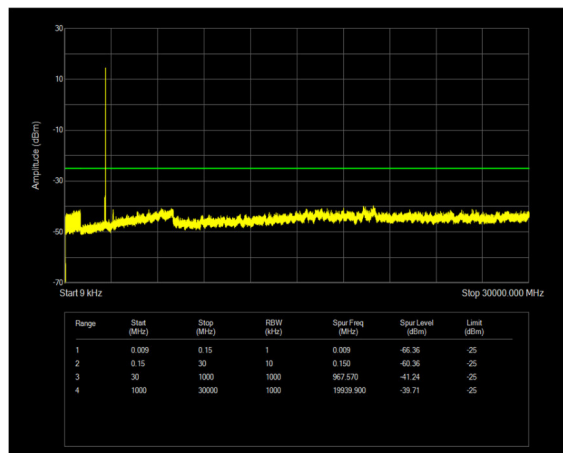
n41 SCS=30kHz CP_QPSK BW=60MHz Channel=518598 RB=1@161
