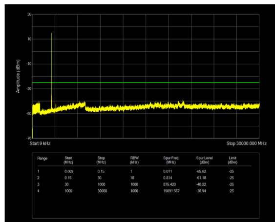
n41 SCS=30kHz CP_QPSK BW=60MHz Channel=505200 RB=1@161
