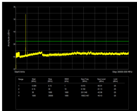
n38 SCS=30kHz DFT_QPSK BW=40MHz Channel=520000 RB=1@105
