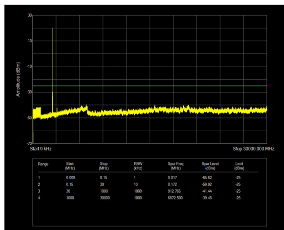
n41 SCS=30kHz CP_QPSK BW=60MHz Channel=505200 RB=1@0
