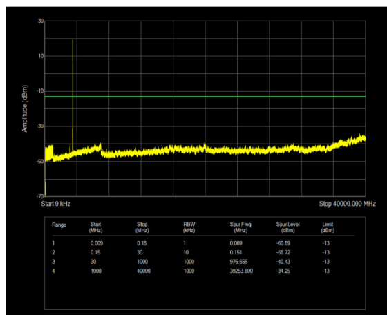
n77(3450-3500) SCS=30kHz CP_QPSK BW=20MHz Channel=630668 RB=1@50
