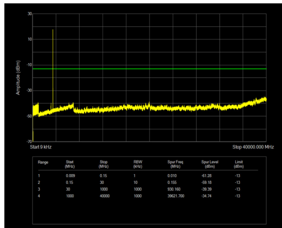
n77(3450-3500) SCS=30kHz DFT_QPSK BW=20MHz Channel=630668 RB=1@0
