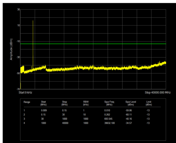
n77(3450-3500) SCS=30kHz CP_QPSK BW=20MHz Channel=630668 RB=1@0
