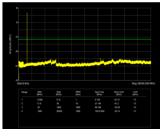
n66 SCS=15kHz DFT_QPSK BW=5MHz Channel=342500 RB=1@24
