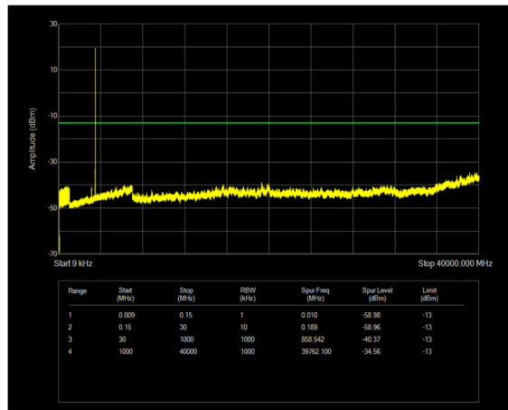
n77(3450-3550) SCS=30kHz CP_QPSK BW=20MHz Channel=630668 RB=1@50
