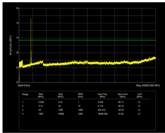
n77(3450-3550) SCS=30kHz CP_QPSK BW=100MHz Channel=633334 RB=1@0
