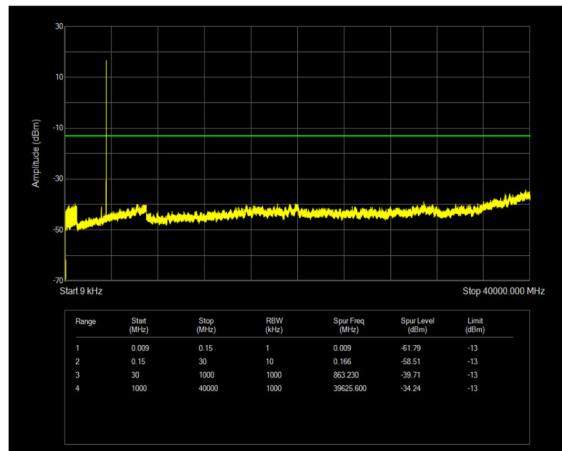
n77(3450-3550) SCS=30kHz CP_QPSK BW=20MHz Channel=636000 RB=1@50
