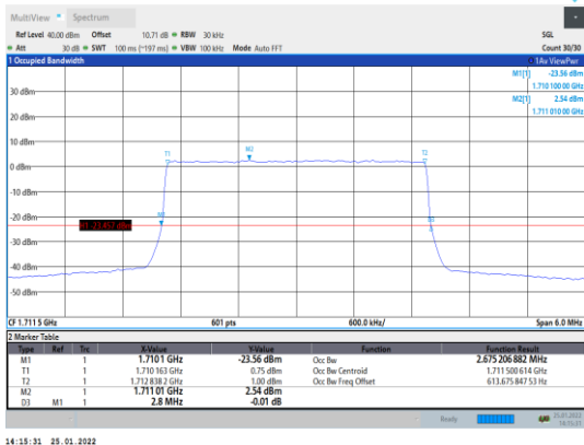
Band4-3MHz-QPSK-19965-15RB#0
