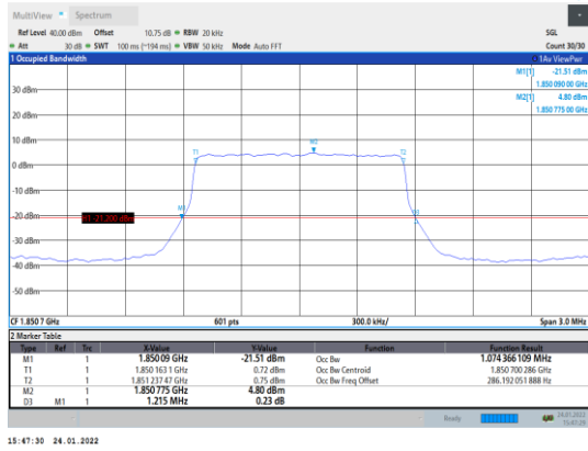
Band2-1.4MHz-QPSK-18607-6RB#0
