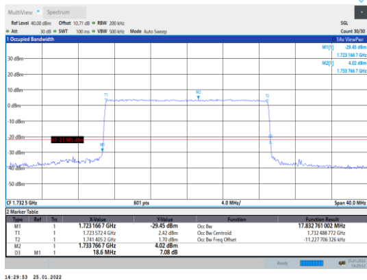
Band4-20MHz-QPSK-20175-100RB#0
