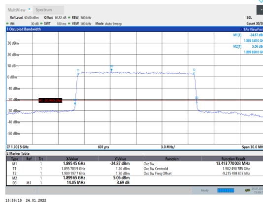
Band2-15MHz-16QAM-19125-75RB#0
