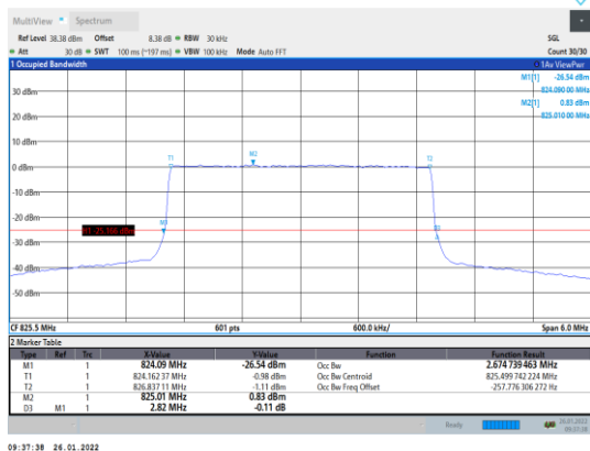
Band5-3MHz-QPSK-20415-15RB#0
