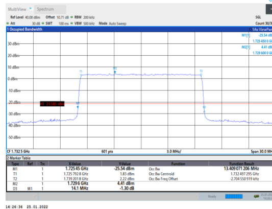
Band4-15MHz-16QAM-20175-75RB#0
