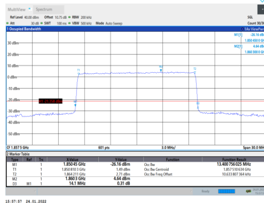
Band2-15MHz-16QAM-18675-75RB#0
