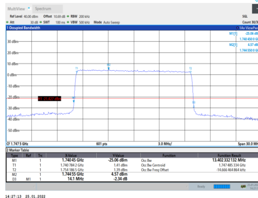
Band4-15MHz-16QAM-20325-75RB#0
