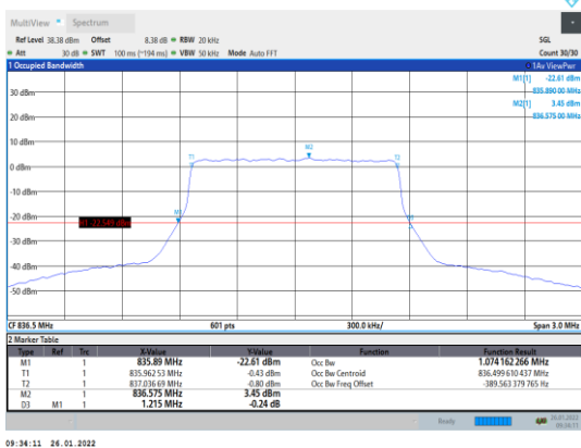
Band5-1.4MHz-QPSK-20525-6RB#0
