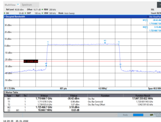
Band4-20MHz-16QAM-20050-100RB#0
