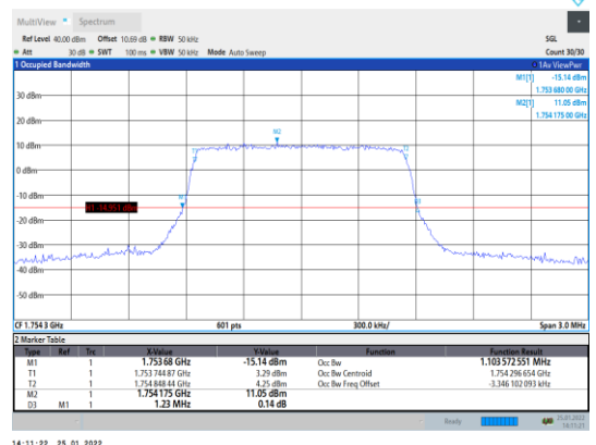
Band4-1.4MHz-16QAM-20393-6RB#0
