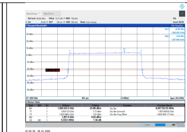
Band2-10MHz-16QAM-18650-50RB#0
