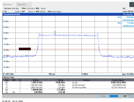
Band2-5MHz-QPSK-19175-25RB#0
