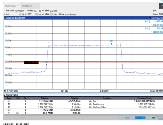
Band4-15MHz-16QAM-20025-75RB#0
