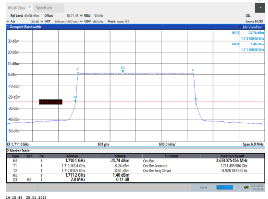
Band4-3MHz-16QAM-19965-15RB#0
