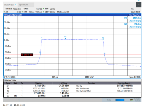
Band4-3MHz-16QAM-20385-15RB#0
