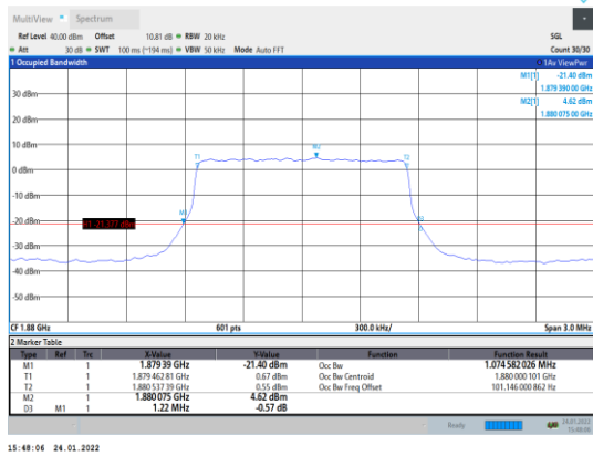
Band2-1.4MHz-QPSK-18900-6RB#0
