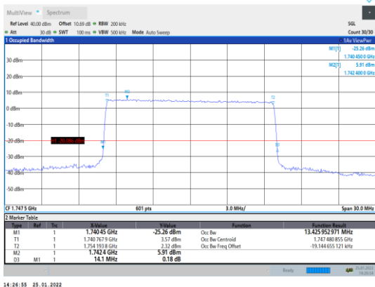
Band4-15MHz-QPSK-20325-75RB#0
