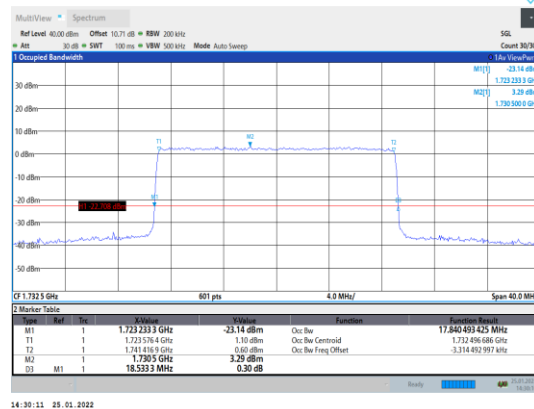
Band4-20MHz-16QAM-20175-100RB#0
