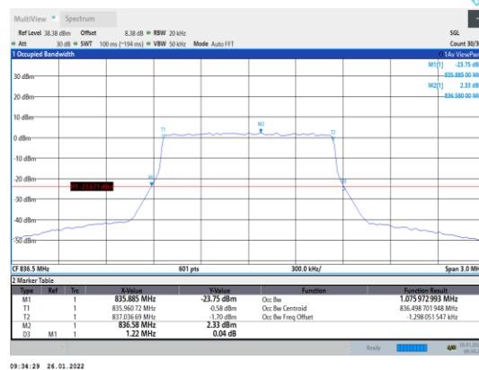
Band5-1.4MHz-16QAM-20525-6RB#0
