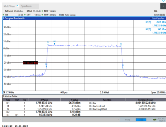
Band4-10MHz-QPSK-20350-50RB#0
