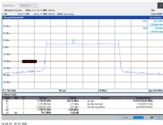
Band4-15MHz-QPSK-20175-75RB#0
