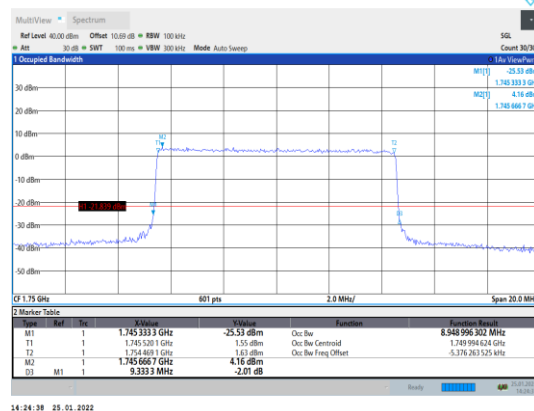
Band4-10MHz-16QAM-20350-50RB#0
