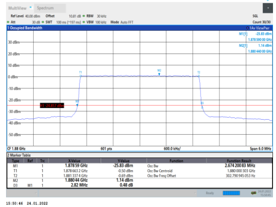
Band2-3MHz-16QAM-18900-15RB#0
