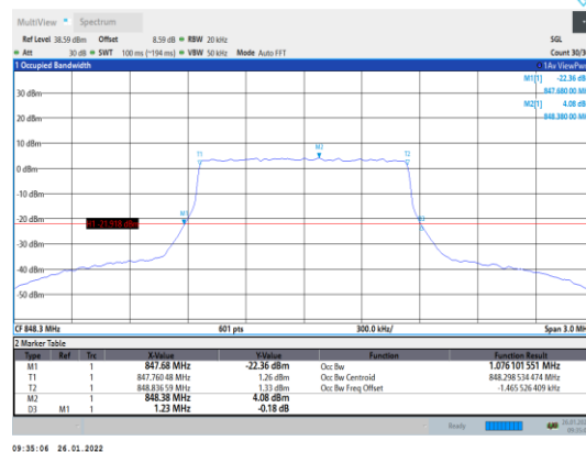
Band5-1.4MHz-16QAM-20643-6RB#0
