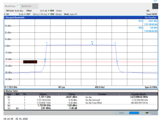
Band4-3MHz-16QAM-20175-15RB#0
