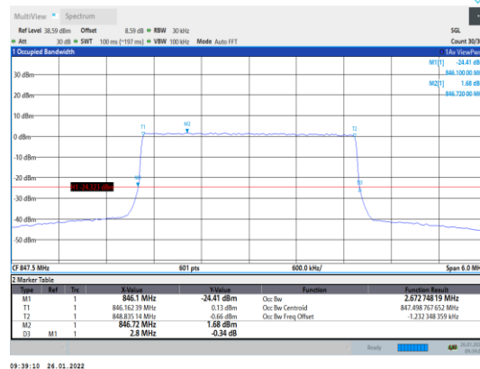
Band5-3MHz-16QAM-20635-15RB#0
