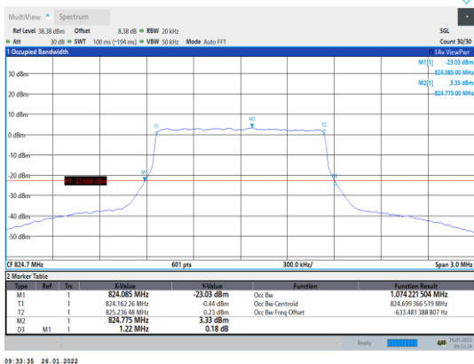
Band5-1.4MHz-QPSK-20407-6RB#0
