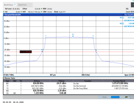
Band5-1.4MHz-16QAM-20407-6RB#0
