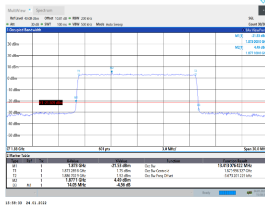
Band2-15MHz-16QAM-18900-75RB#0
