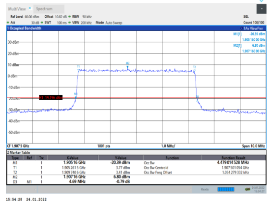
Band2-5MHz-16QAM-19175-25RB#0
