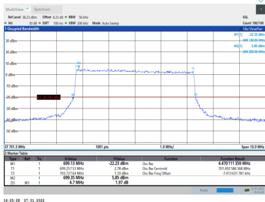
Band12-5MHz-QPSK-23035-25RB#0
