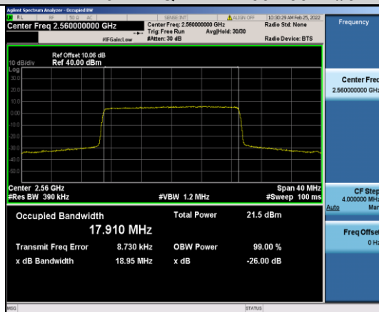
Band7-20MHz-QPSK-21350-100RB#0
