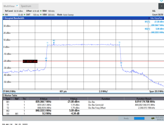
Band5-10MHz-QPSK-20600-50RB#0
