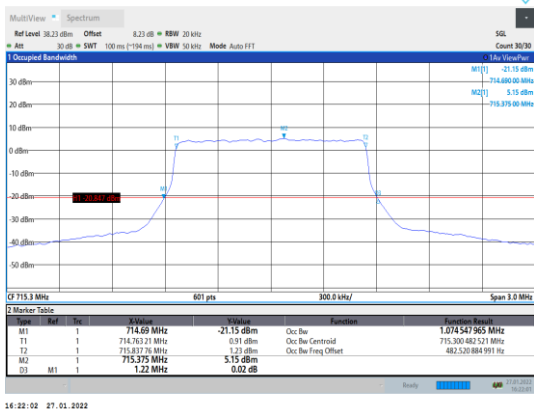
Band12-1.4MHz-QPSK-23173-6RB#0
