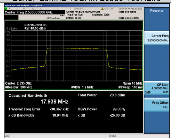
Band7-20MHz-16QAM-21100-100RB#0
