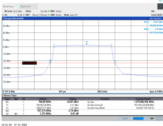
Band12-1.4MHz-QPSK-23095-6RB#0
