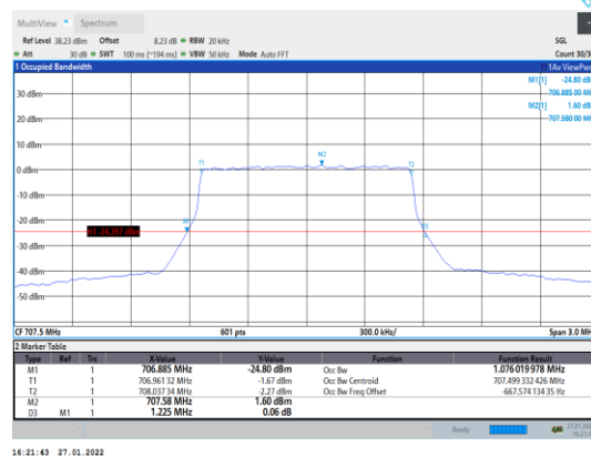
Band12-1.4MHz-16QAM-23095-6RB#0
