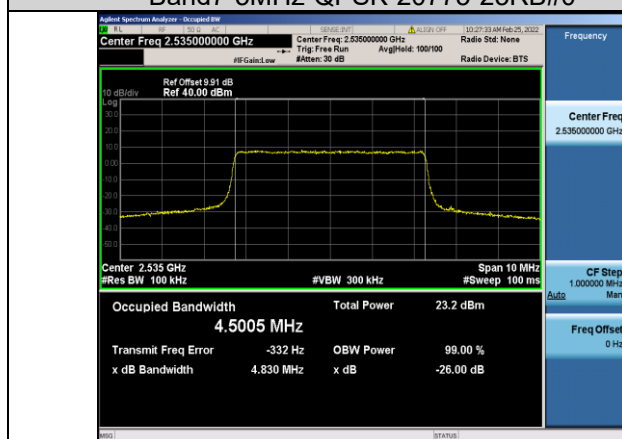
Band7-5MHz-QPSK-21100-25RB#0
