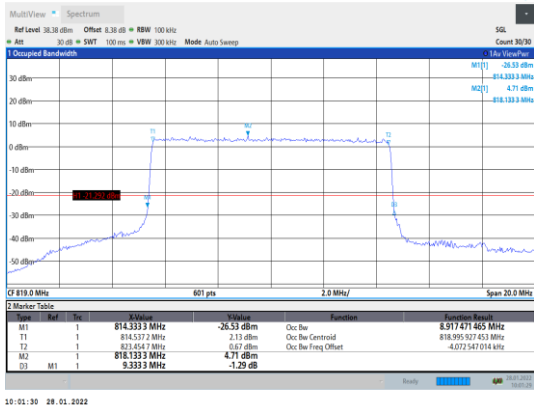
Band26-10MHz-QPSK-26740-50RB#0
