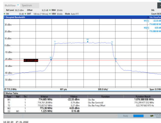
Band12-1.4MHz-16QAM-23173-6RB#0
