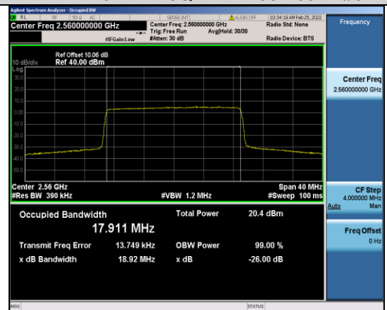
Band7-20MHz-16QAM-21350-100RB#0
