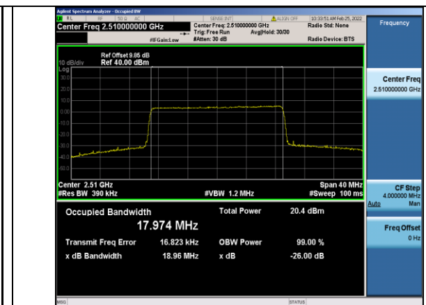
Band7-20MHz-16QAM-20850-100RB#0
