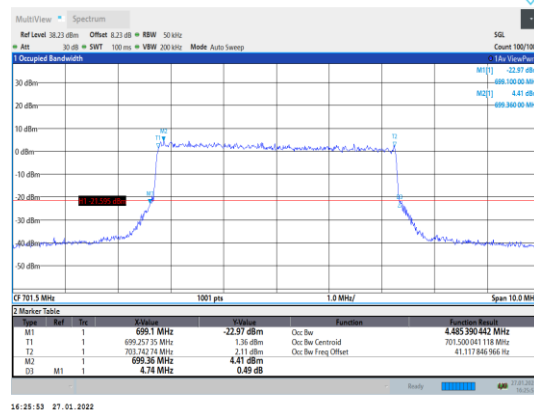
Band12-5MHz-16QAM-23035-25RB#0
