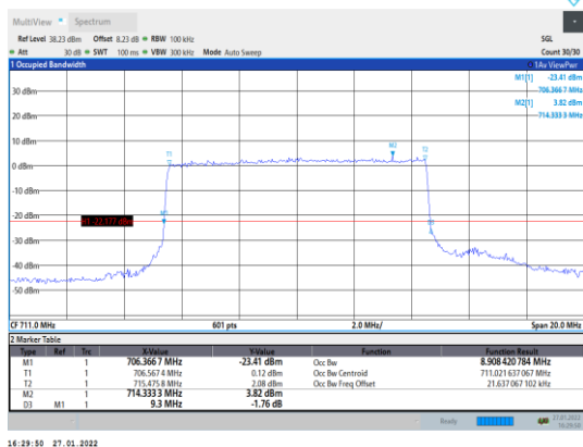
Band12-10MHz-QPSK-23130-50RB#0
