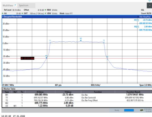
Band12-1.4MHz-QPSK-23017-6RB#0
