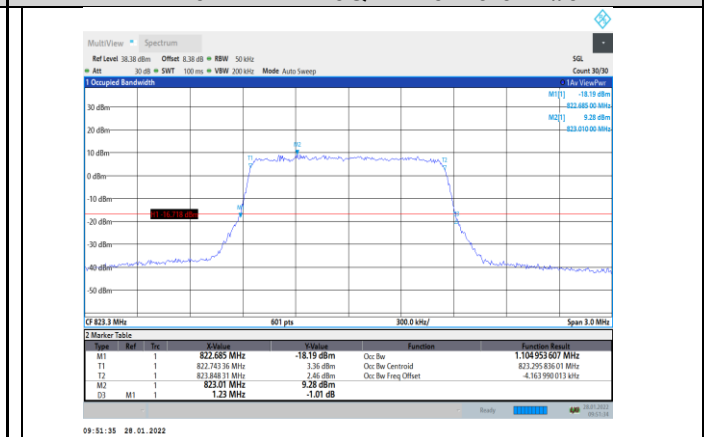
Band26-1.4MHz-16QAM-26783-6RB#0
