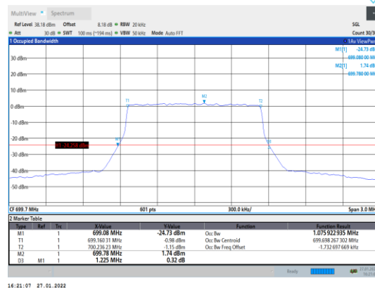
Band12-1.4MHz-16QAM-23017-6RB#0
