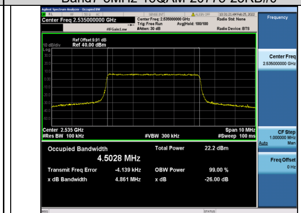
Band7-5MHz-16QAM-21100-25RB#0
