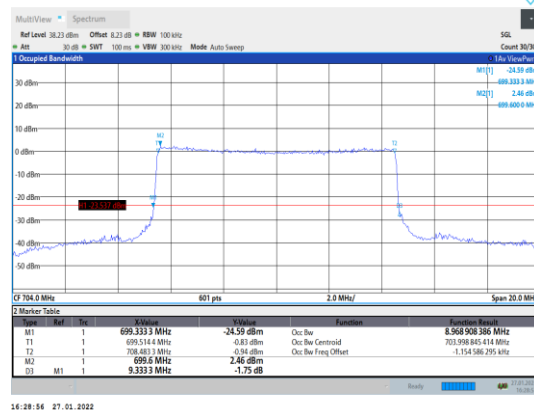
Band12-10MHz-16QAM-23060-50RB#0
