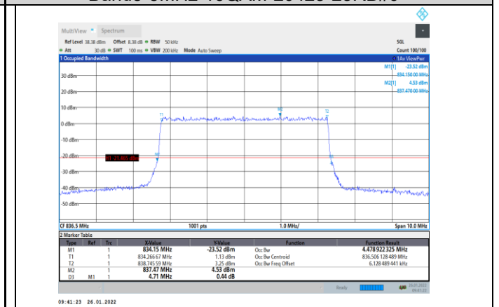
Band5-5MHz-16QAM-20525-25RB#0
