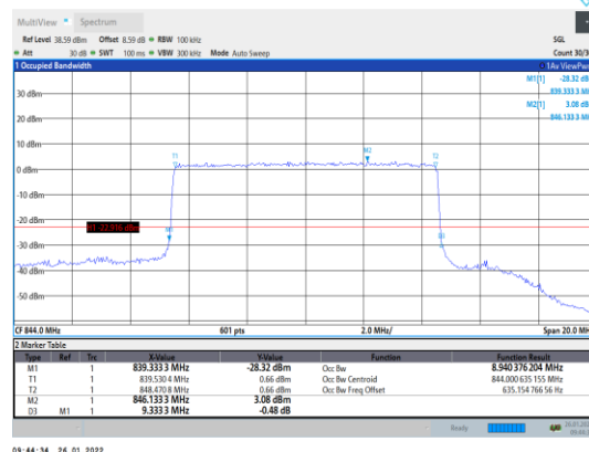
Band5-10MHz-16QAM-20600-50RB#0
