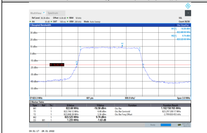
Band26-1.4MHz-QPSK-26783-6RB#0
