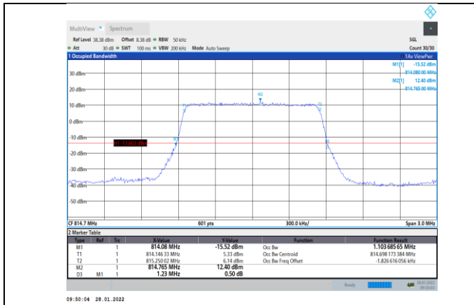
Band26-1.4MHz-QPSK-26697-6RB#0
