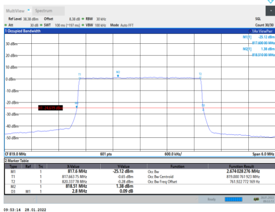
Band26-3MHz-QPSK-26740-15RB#0
