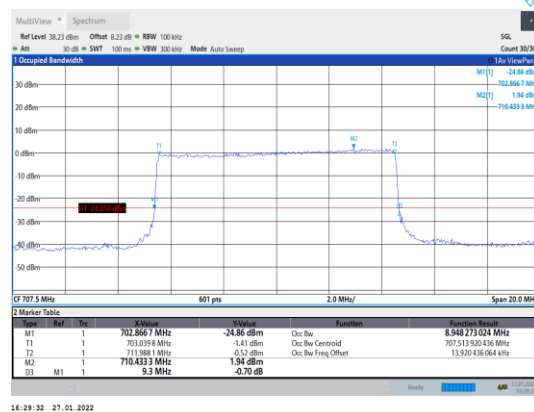
Band12-10MHz-16QAM-23095-50RB#0
