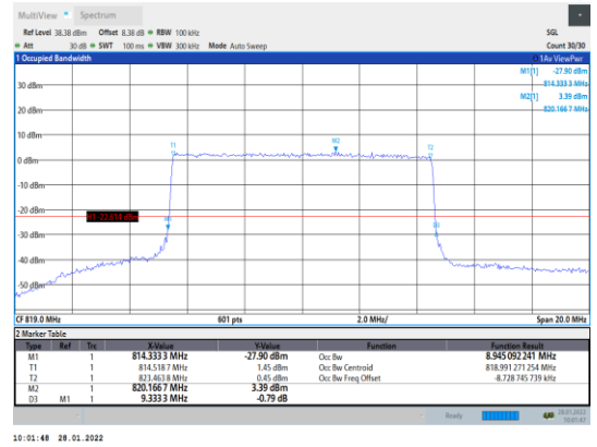
Band26-10MHz-16QAM-26740-50RB#0
