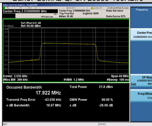
Band7-20MHz-QPSK-21100-100RB#0
