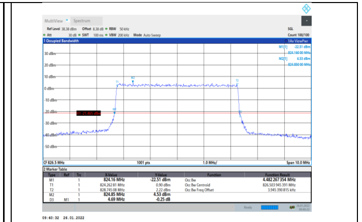
Band5-5MHz-16QAM-20425-25RB#0
