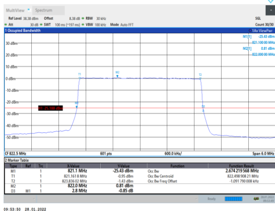
Band26-3MHz-QPSK-26775-15RB#0
