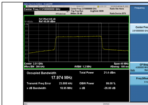
Band7-20MHz-QPSK-20850-100RB#0
