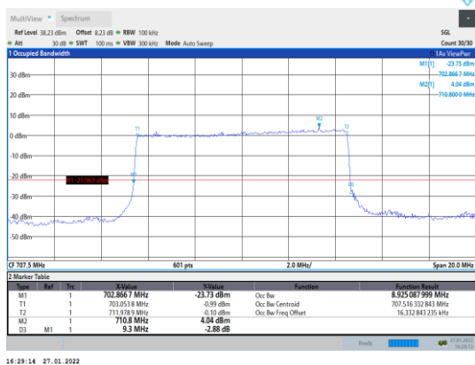
Band12-10MHz-QPSK-23095-50RB#0
