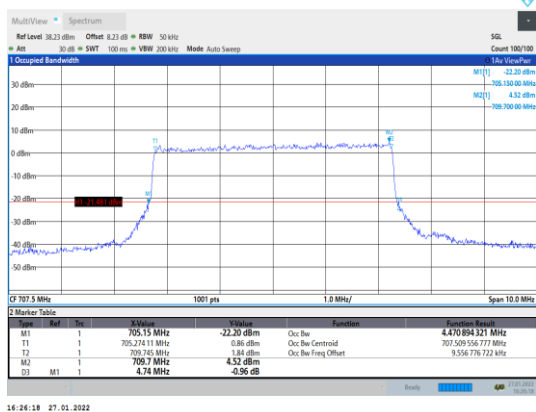
Band12-5MHz-QPSK-23095-25RB#0
