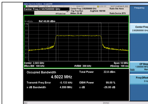
Band7-5MHz-QPSK-20775-25RB#0
