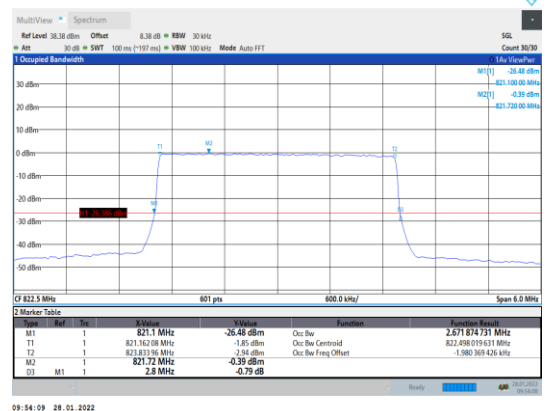
Band26-3MHz-16QAM-26775-15RB#0
