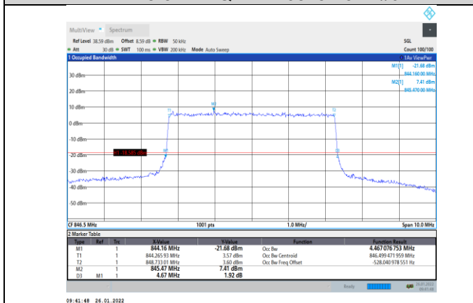
Band5-5MHz-QPSK-20625-25RB#0
