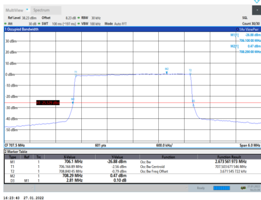
Band12-3MHz-QPSK-23095-15RB#0
