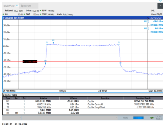
Band12-10MHz-QPSK-23060-50RB#0
