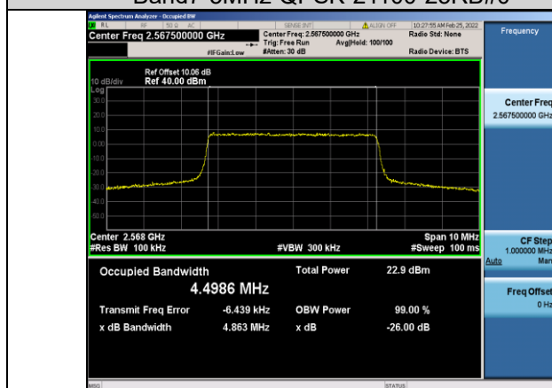
Band7-5MHz-QPSK-21425-25RB#0
