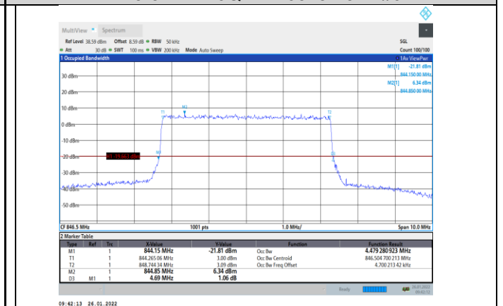
Band5-5MHz-16QAM-20625-25RB#0
