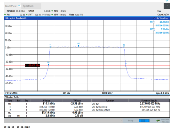
Band26-3MHz-16QAM-26705-15RB#0
