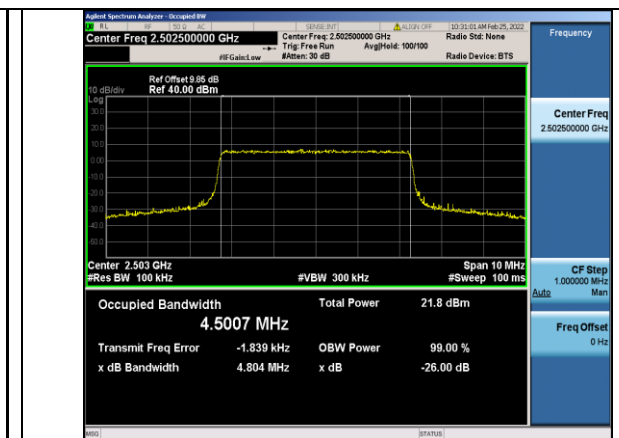
Band7-5MHz-16QAM-20775-25RB#0
