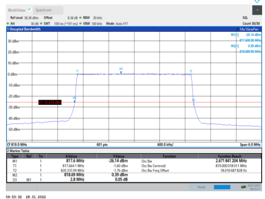
Band26-3MHz-16QAM-26740-15RB#0
