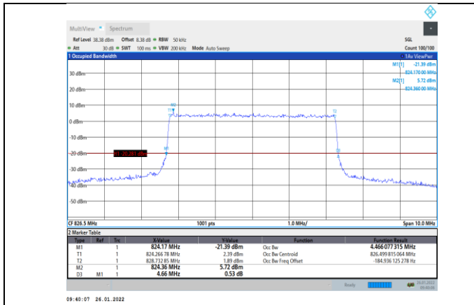
Band5-5MHz-QPSK-20425-25RB#0
