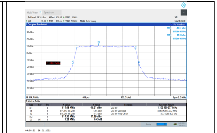
Band26-1.4MHz-16QAM-26697-6RB#0
