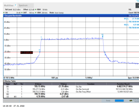
Band12-5MHz-16QAM-23095-25RB#0
