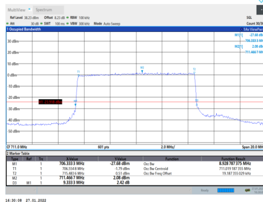
Band12-10MHz-16QAM-23130-50RB#0
