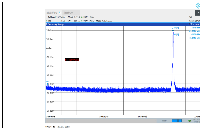
Band5-4132-30~1000MHz
