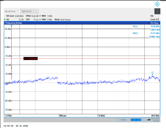
Band2-1.4MHz-16QAM-19193-1RB#0-Range2 :1000~20000MHz
