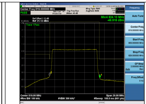
Band26-10MHz-QPSK-26740 Right-50RB#0
