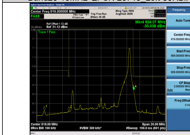
Band26-10MHz-QPSK-26740 Right-1RB#49
