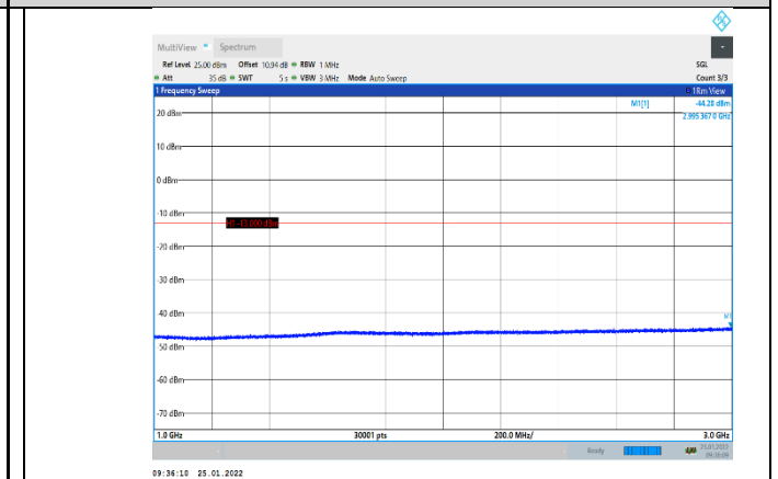
Band5-4182-1000~3000MHz
