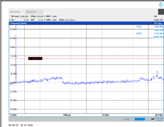
Band2-1.4MHz-16QAM-18607-1RB#0-Range :1000~20000MHz
