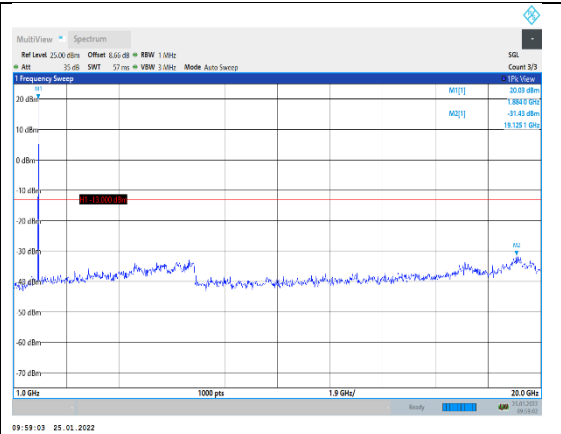
Band2-1.4MHz-16QAM-18900-1RB#0-Range2 :1000~20000MHz
