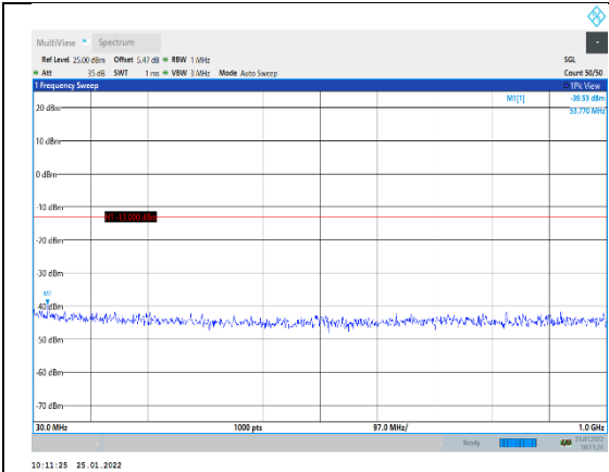
Band2-15MHz-QPSK-18675-1RB#0-Range1: 0~1000MHz
