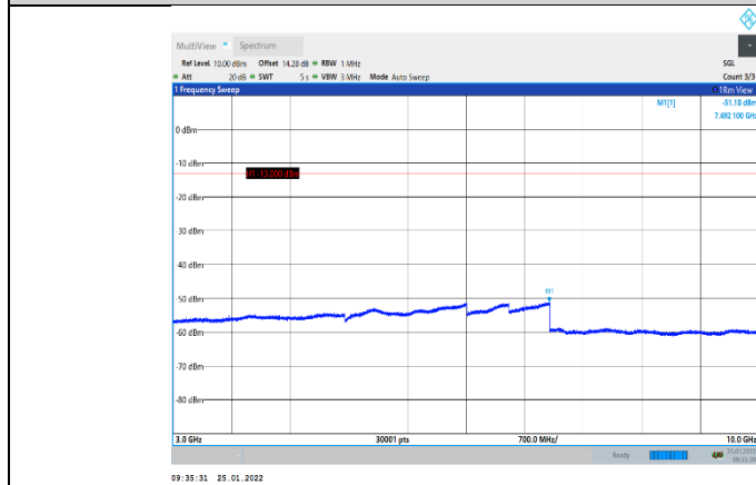
Band5-4132-3000~10000MHz
