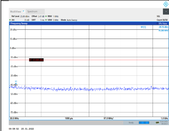
Band2-1.4MHz-16QAM-18900-1RB#0-Range :30~1000MHz
