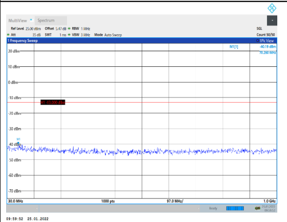
Band2-1.4MHz-16QAM-19193-1RB#0-Range1 :30~1000MHz
