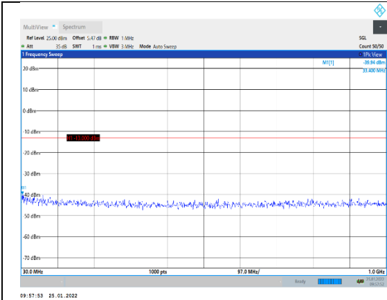
Band2-1.4MHz-16QAM-18607-1RB#0-Range :30~1000MHz
