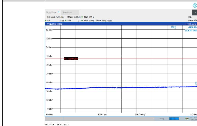
Band5-4132-1000~3000MHz
