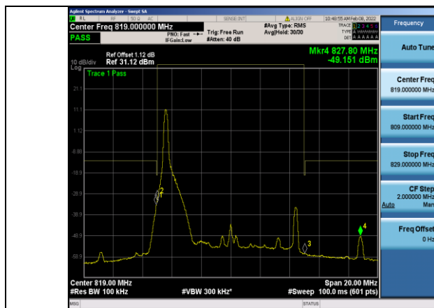
Band26-10MHz-QPSK-26740 Left-1RB#0
