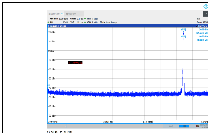
Band5-4233-30~1000MHz
