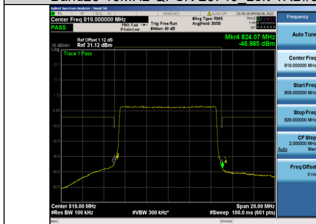
Band26-10MHz-QPSK-26740 Left-50RB#0
