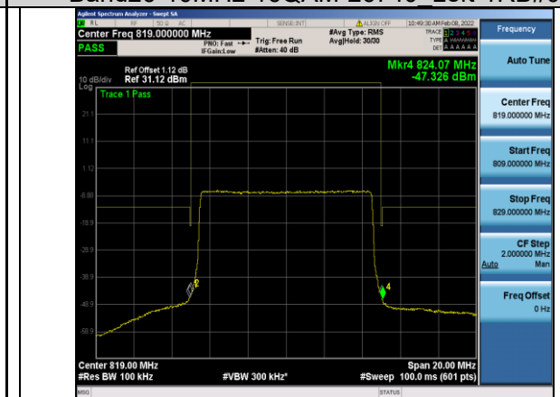
Band26-10MHz-16QAM-26740 Left-50RB#0
