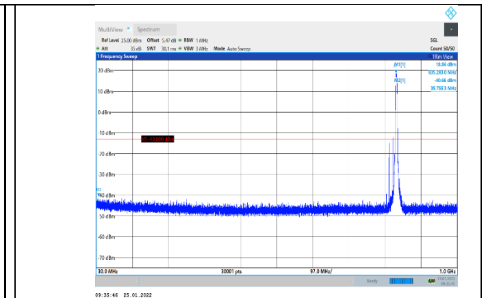
Band5-4182-30~1000MHz
