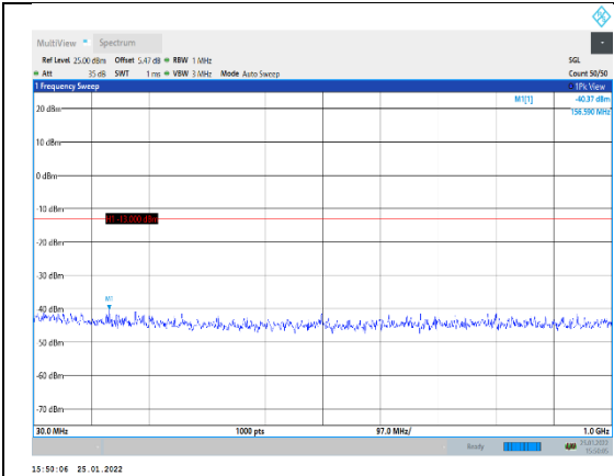
Band4-20MHz-16QAM-20050-1RB#0-Range1 30~1000MHz
