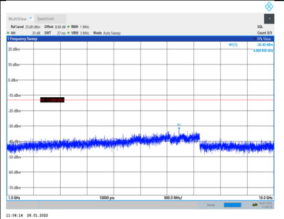
Band5-5MHz-16QAM-20525-1RB#0-Range2:1 000~10000MHz
