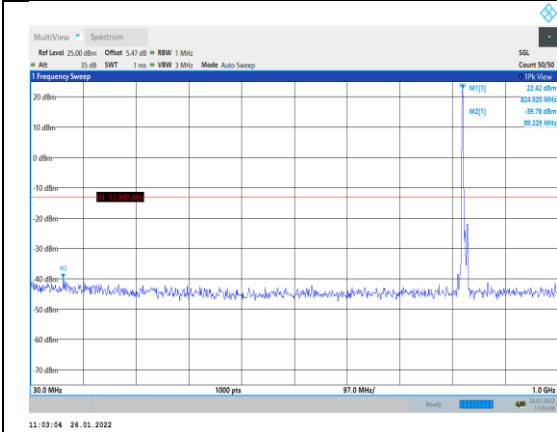
Band5-5MHz-16QAM-20425-1RB#0-Range1: 0~1000MHz
