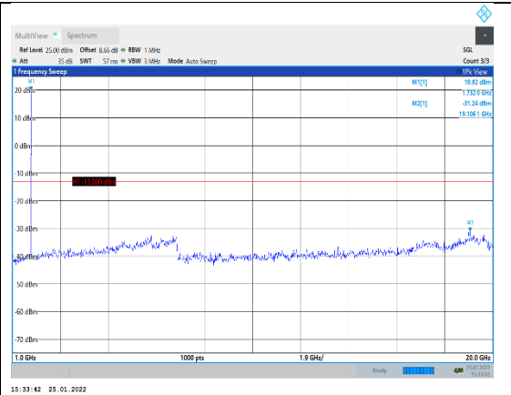
Band4-1.4MHz-16QAM-20175-1RB#0-Range2 :1000~20000MHz
