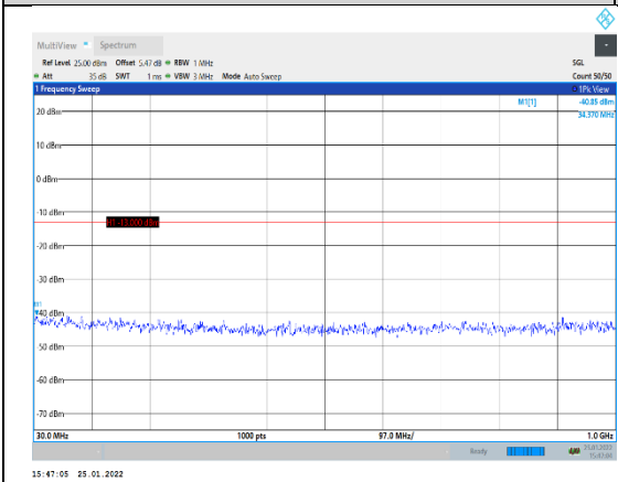
Band4-15MHz-QPSK-20175-1RB#0-Range1: 0~1000MHz
