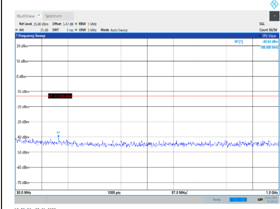
Band4-20MHz-QPSK-20175-1RB#0-Range1: 0~1000MHz
