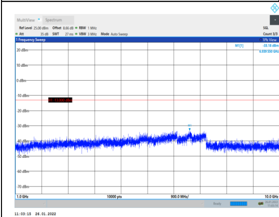
Band5-5MHz-16QAM-20425-1RB#0-Range2: 000~10000MHz
