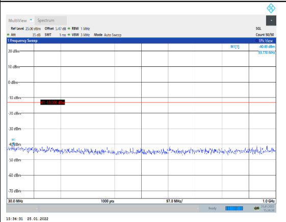
Band4-1.4MHz-16QAM-20393-1RB#0-Range1 :30~1000MHz
