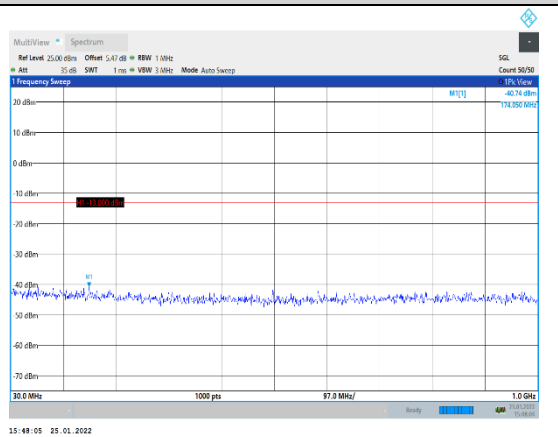
Band4-15MHz-QPSK-20325-1RB#0-Range1:3 0~1000MHz
