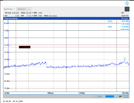
Band4-1.4MHz-16QAM-20393-1RB#0-Range2 :1000~20000MHz
