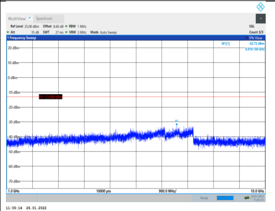
Band5-5MHz-16QAM-20625-1RB#0-Range2:1 000~10000MHz
