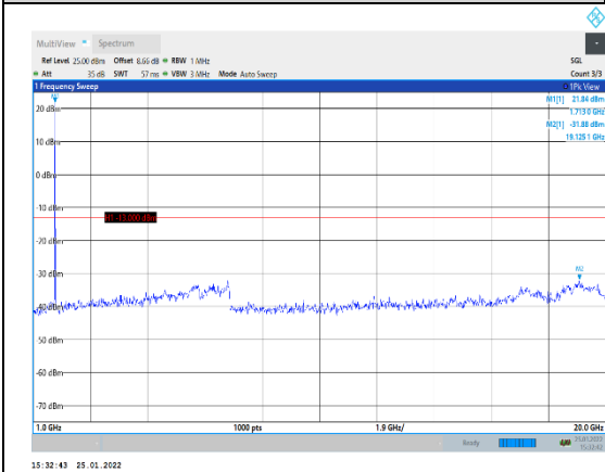
Band4-1.4MHz-16QAM-19957-1RB#0-Range :1000~20000MHz
