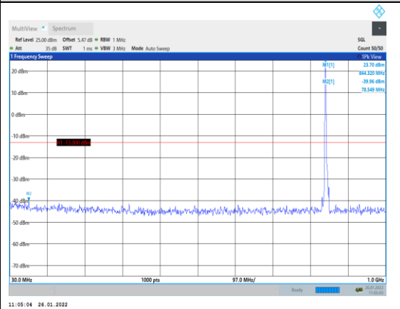
Band5-5MHz-16QAM-20625-1RB#0-Range1:3 0~1000MHz
