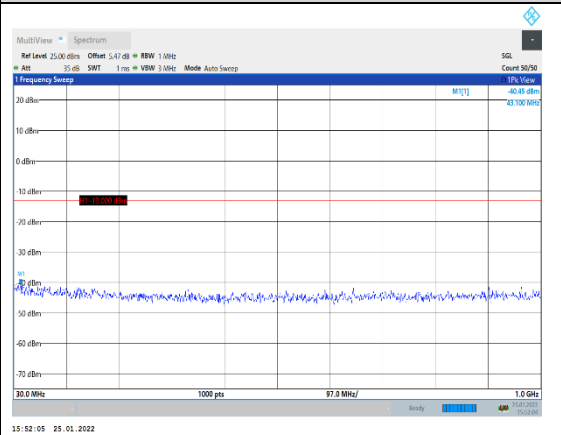
Band4-20MHz-16QAM-20300-1RB#0-Range1: 30~1000MHz
