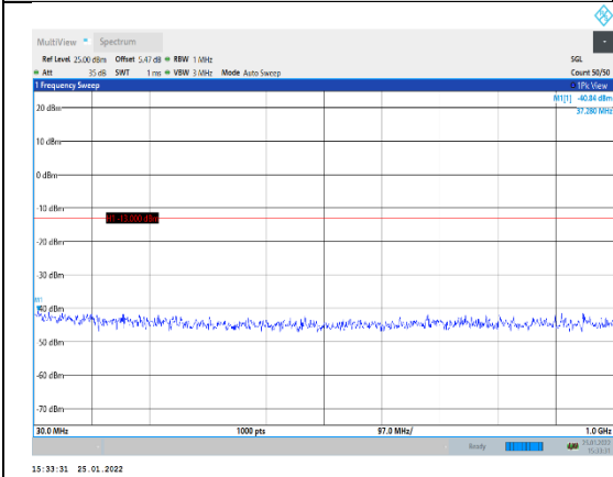
Band4-1.4MHz-16QAM-20175-1RB#0-Range :30~1000MHz
