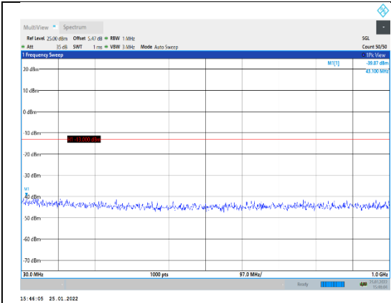
Band4-15MHz-QPSK-20025-1RB#0-Range1: 0~1000MHz
