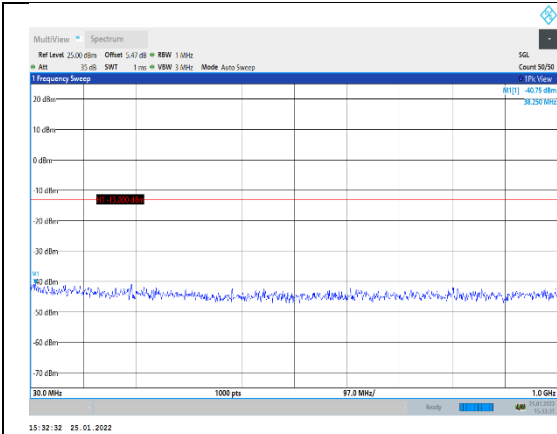
Band4-1.4MHz-16QAM-19957-1RB#0-Range :30~1000MHz
