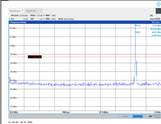
Band5-5MHz-16QAM-20525-1RB#0-Range1: 0~1000MHz
