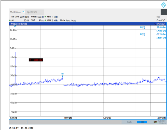
Band4-20MHz-16QAM-20050-1RB#0-Range2: 1000~20000MHz
