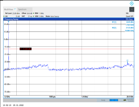
Band4-20MHz-16QAM-20300-1RB#0-Range2: 1000~20000MHz
