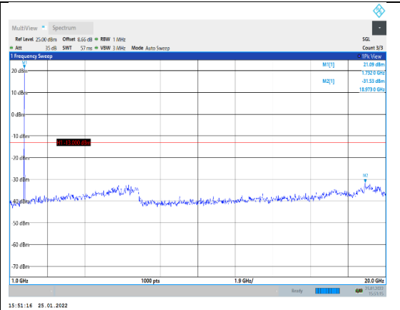
Band4-20MHz-16QAM-20175-1RB#0-Range2: 1000~20000MHz
