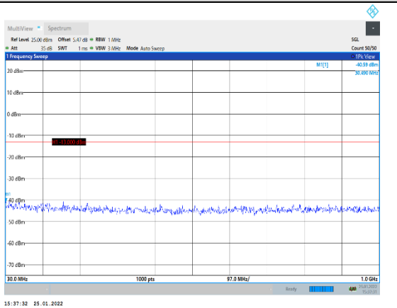
Band4-3MHz-QPSK-20385-1RB#0-Range1:30 ~1000MHz
