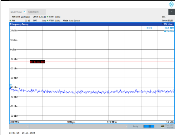
Band4-20MHz-16QAM-20175-1RB#0-Range1 30~1000MHz
