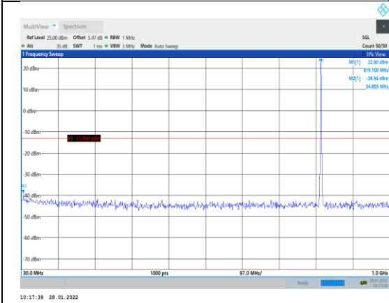
Band26-1.4MHz-QPSK-26740-1RB#0-Range :30~1000MHz
