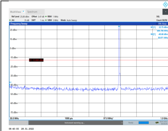
Band12-3MHz-QPSK-23025-1RB#0-Range1: 0~1000MHz
