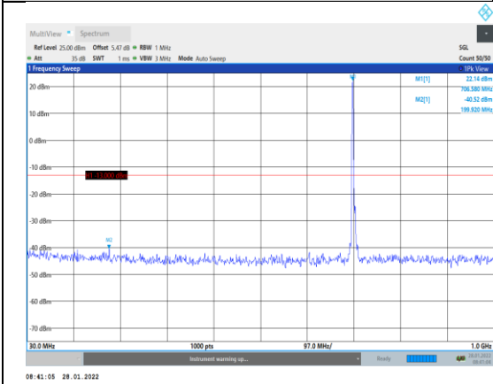
Band12-3MHz-QPSK-23095-1RB#0-Range1: 0~1000MHz
