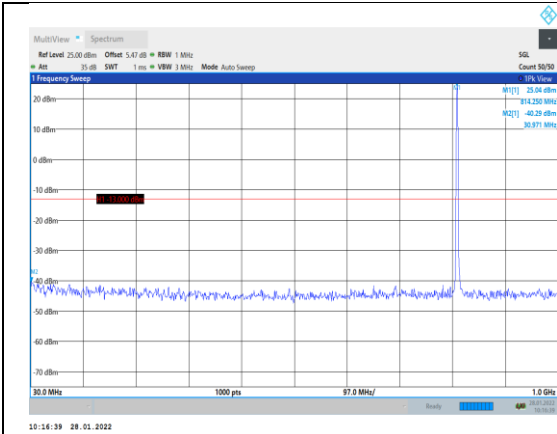
Band26-1.4MHz-QPSK-26697-1RB#0-Range :30~1000MHz
