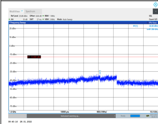
Band12-3MHz-QPSK-23025-1RB#0-Range2: 000~10000MHz
