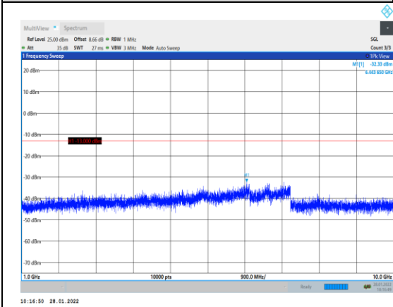
Band26-1.4MHz-QPSK-26697-1RB#0-Range :1000~10000MHz
