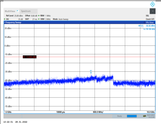
Band26-3MHz-16QAM-26740-1RB#0-Range2: 1000~10000MHz
