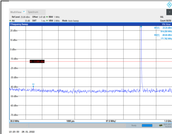
Band26-3MHz-16QAM-26705-1RB#0-Range1 30~1000MHz
