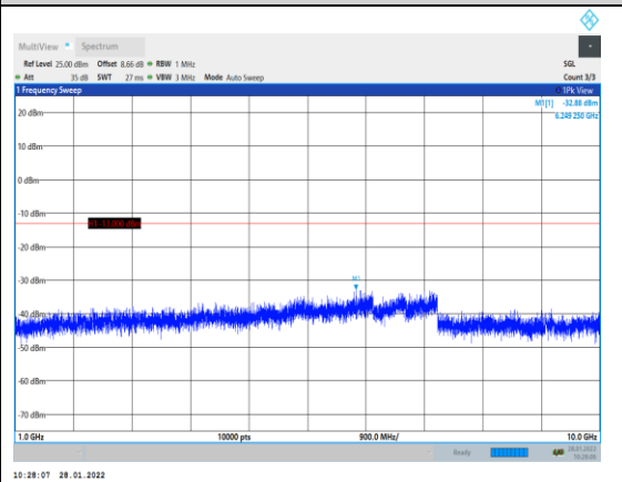
Band26-10MHz-16QAM-26740-1RB#0-Range 2:1000~10000MHz
