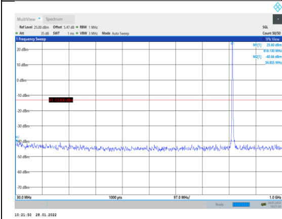
Band26-3MHz-16QAM-26740-1RB#0-Range1 30~1000MHz
