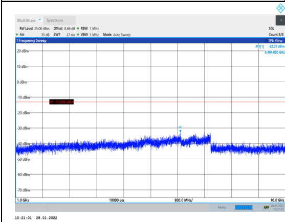
Band26-3MHz-16QAM-26705-1RB#0-Range2: 1000~10000MHz
