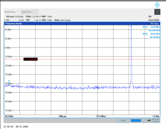
Band26-3MHz-16QAM-26775-1RB#0-Range1: 30~1000MHz
