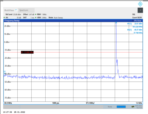
Band26-10MHz-16QAM-26740-1RB#0-Range 1:30~1000MHz
