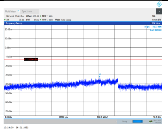
Band26-3MHz-16QAM-26775-1RB#0-Range2: 1000~10000MHz
