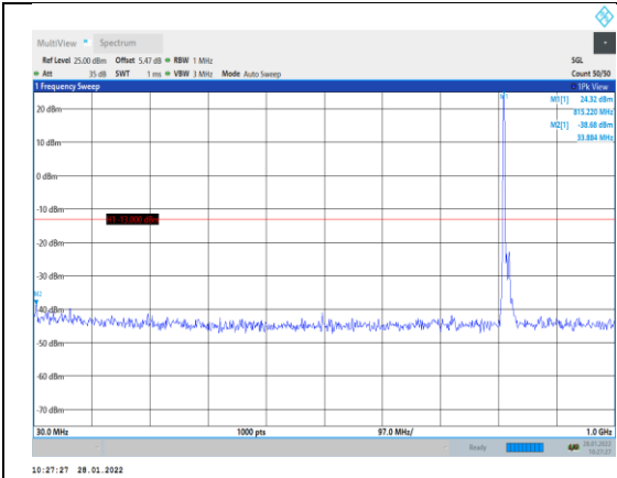
Band26-10MHz-QPSK-26740-1RB#0-Range 30~1000MHz
