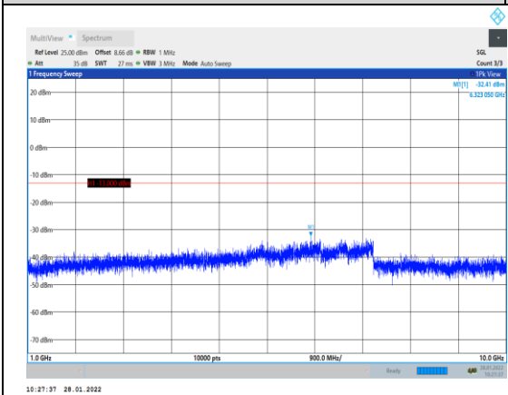
Band26-10MHz-QPSK-26740-1RB#0-Range2 1000~10000MHz
