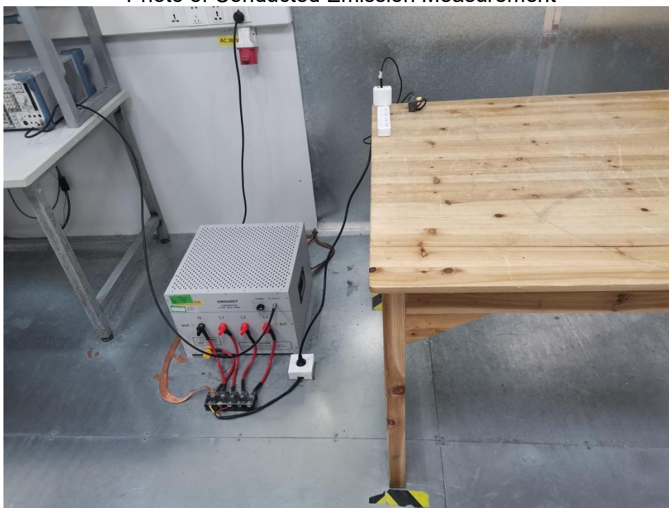
FCC ID: 2A39T-GSR3520 Photo of Conducted Emission Measurement
