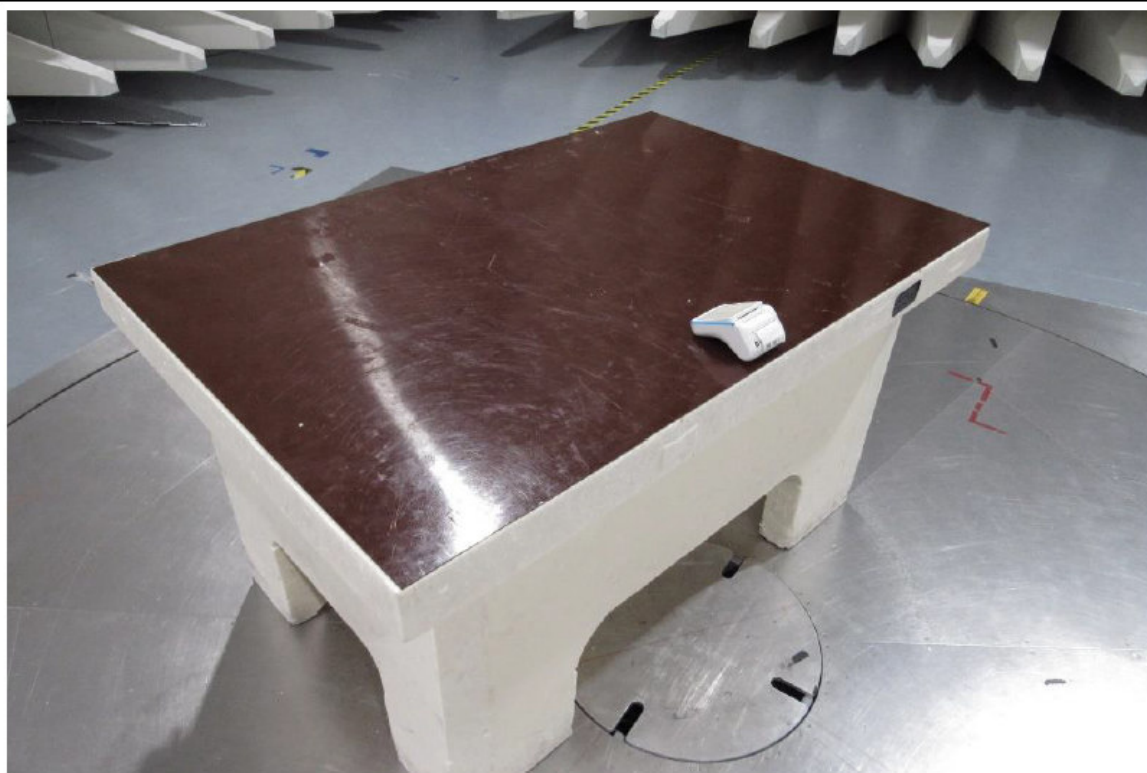
TEST SETUP 30 – 1000 MHz - CONFIGURATION 1 AC6
