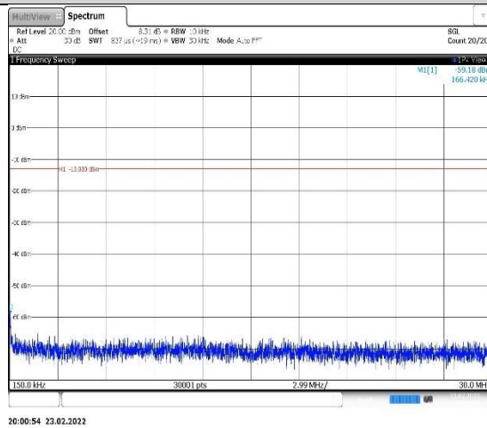
Band5-4132-1-0.15~30MHz
