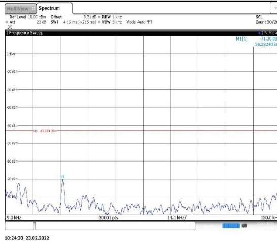
Band2-9538-0.009~0.15MHz
