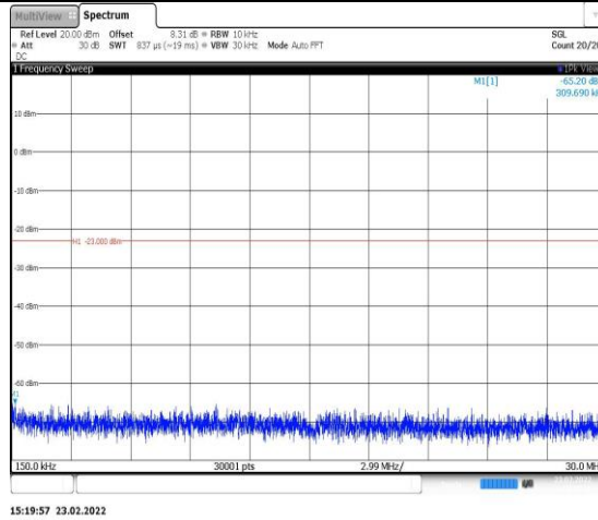
Band2-9538-1-0.15~30MHz
