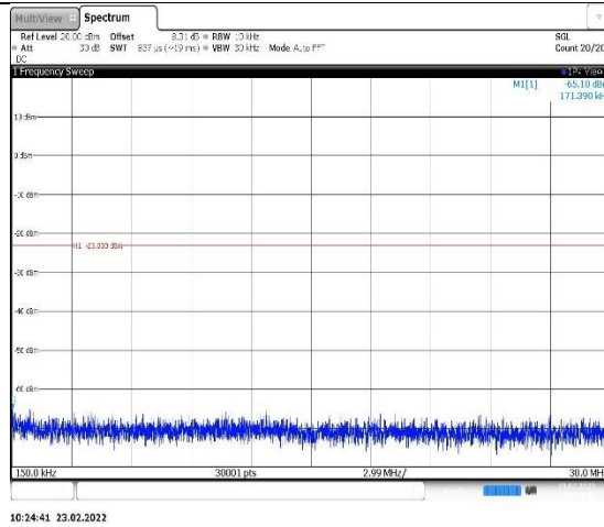
Band2-9538-0.15~30MHz
