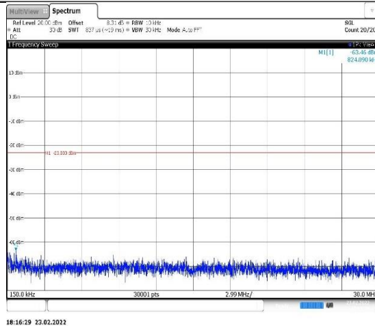
Band2-9262-1-0.15~30MHz
