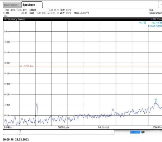
Band5-4132-1-0.009~0.15MHz
