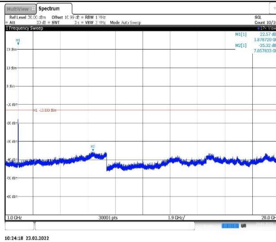
Band2-9400-1000~20000MHz
