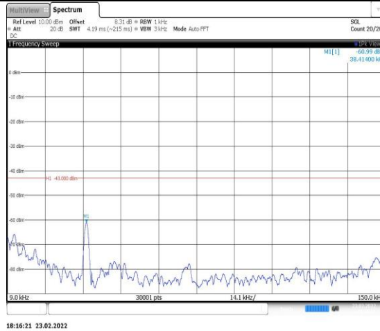
Band2-9262-1-0.009~0.15MHz
