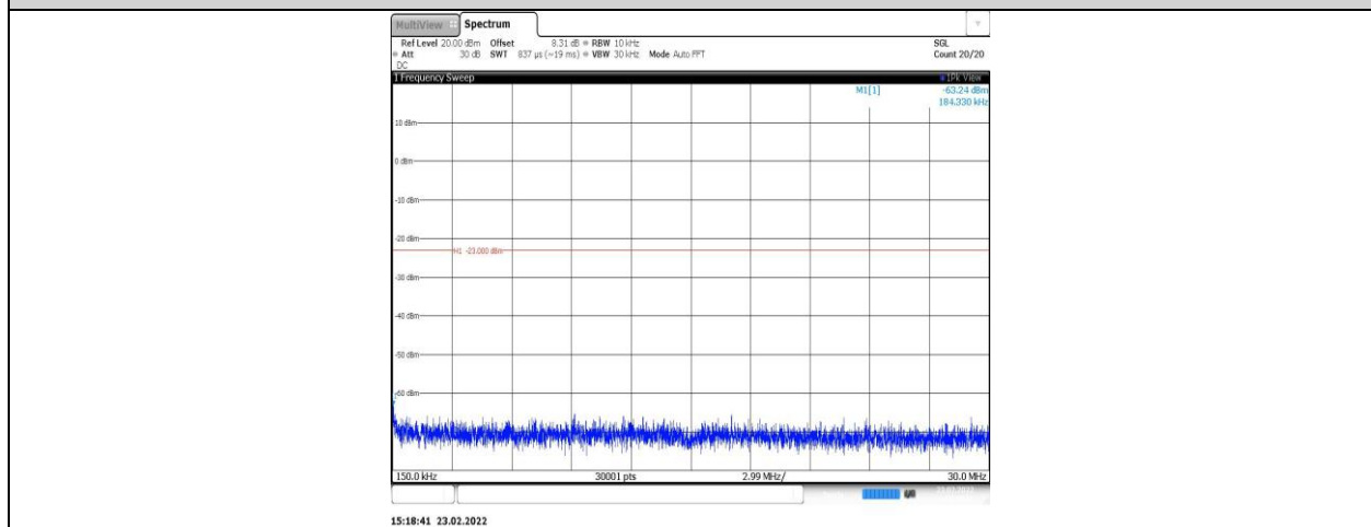
Band2-9400-1-0.15~30MHz
