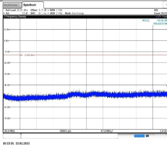
Band2-9400-30~1000MHz
