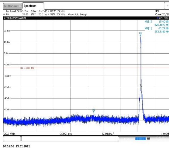
Band5-4132-1-30~1000MHz
