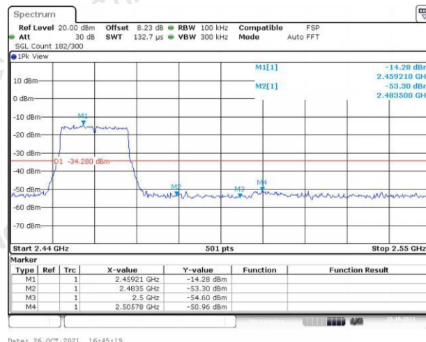
Right bandedge
