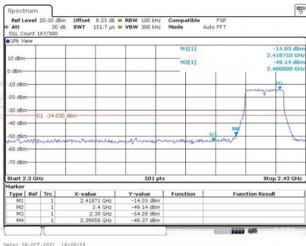
Left bandedge
