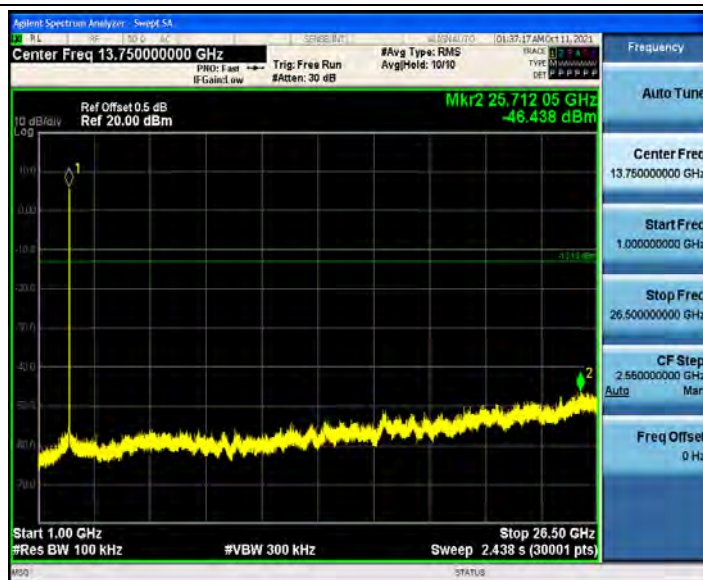
802.11b_2437_0~Reference
