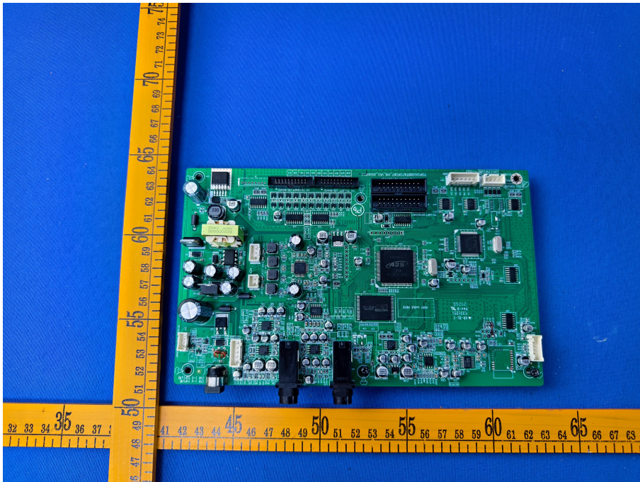
INTERNAL VIEW OF SAMPLE PCB
