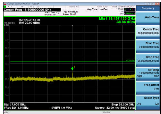
U-NII-2c ,Plot 4,7000MHz~26000MHz-802 .11n(20MHz),5700MHz,Ant1
