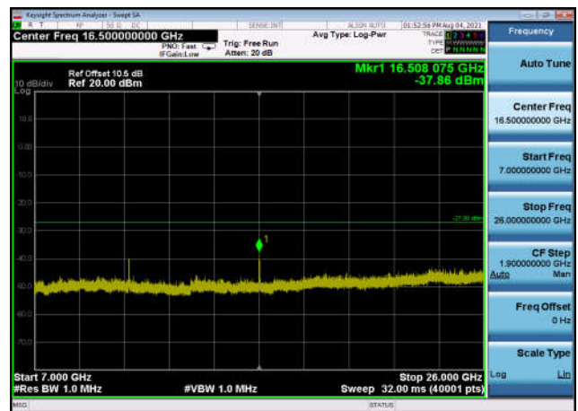
U-NII-2c ,Plot 4,7000MHz~26000MHz-802 .11a(20MHz),5500MHz,Ant1
