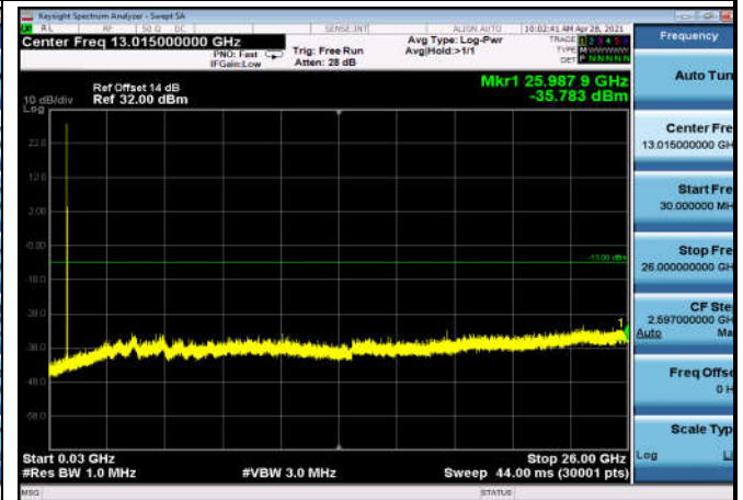
FDD05_MidRange_10MHz_30MHz~26GHz
