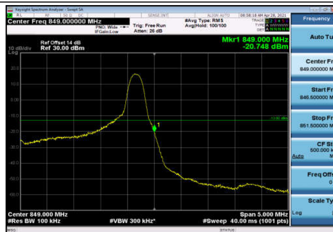
HighRange_FDD05_5MHz_846.5_fullIRB _High_QPSK
