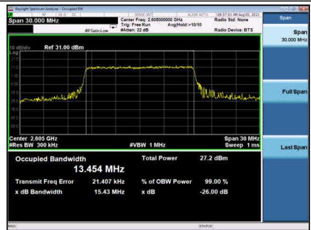
TDD41_MidRange_20_2605_Q16
