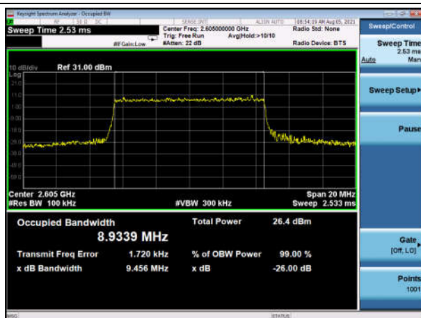
TDD41_MidRange_10_2605_QPSK
