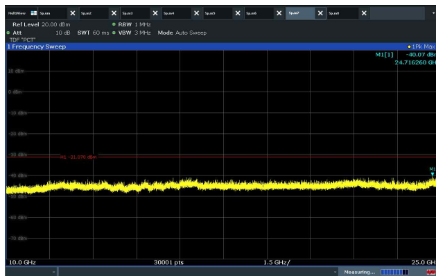
802.11b_CH Middle(Above 1 GHz)
