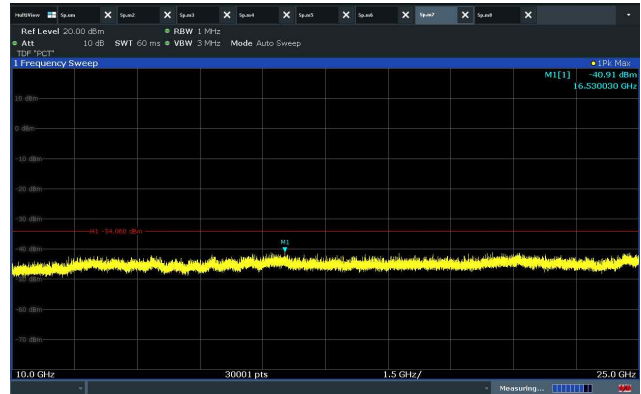
802.11g_CH Middle(Above 1 GHz)
