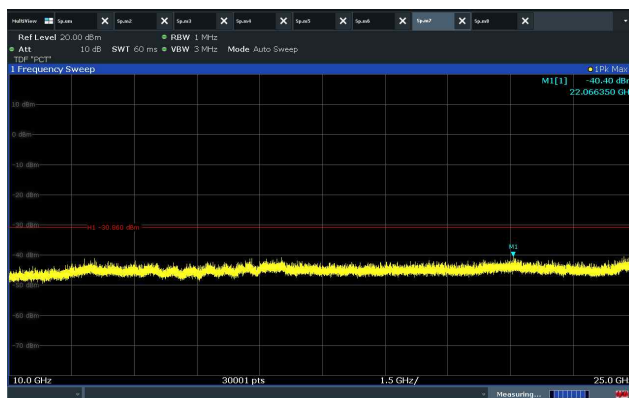
802.11b_CH High(Above 1 GHz)
