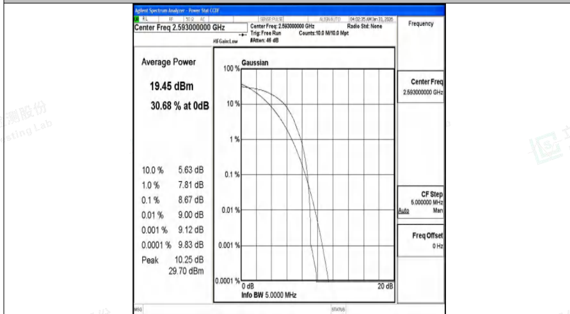
Band41-5MHz-16QAM-40620-1RB#0-PASS
