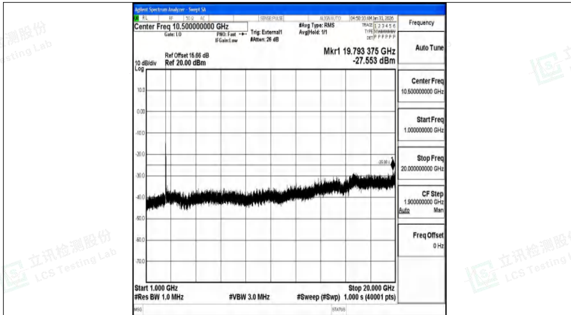
Band41_15MHz_16QAM_39725_1RB#0_1000~20000_1000~20000
