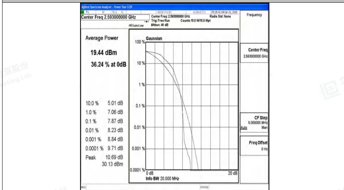
Band41-20MHz-QPSK-40620-1RB#0-PASS
