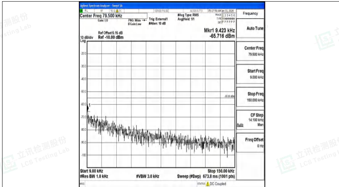
Band41_20MHz_QPSK_39750_1RB#0_0.009~0.15_0.009~0.15
