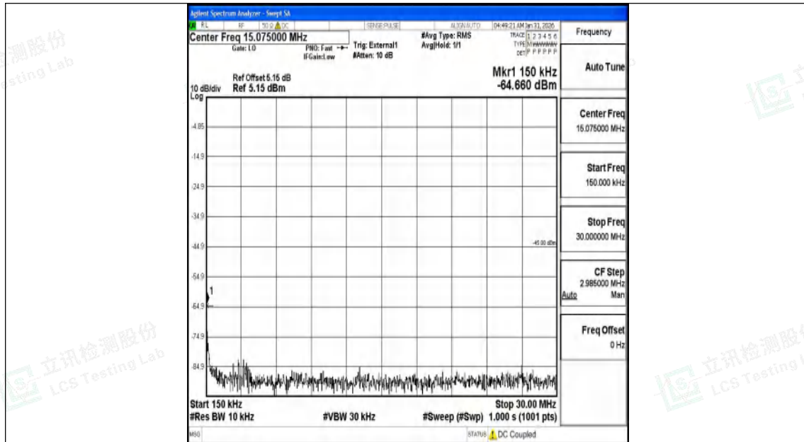
Band41_15MHz_16QAM_39725_1RB#0_0.15~30_0.15~30
