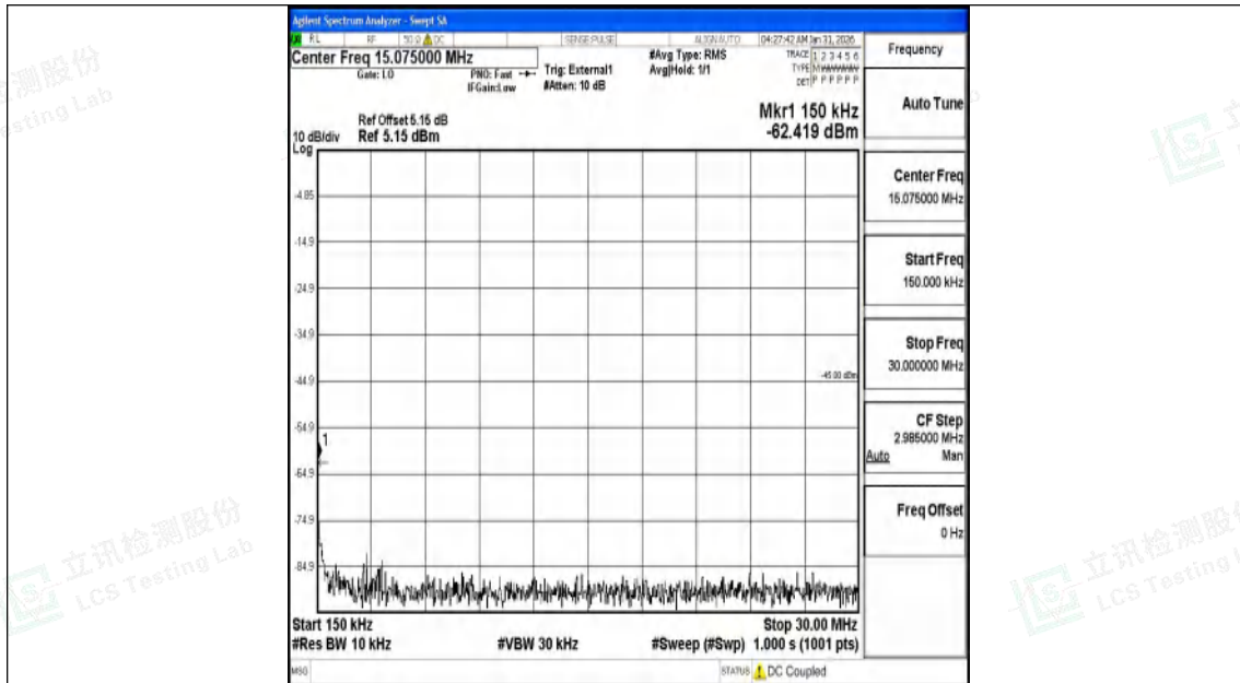
Band41_10MHz_16QAM_41540_1RB#0_0.15~30_0.15~30
