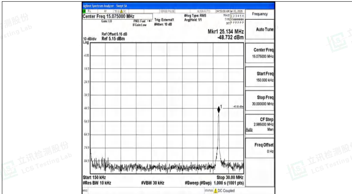
Band41_15MHz_16QAM_40620_1RB#0_0.15~30_0.15~30
