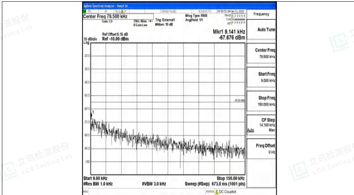
Band41_15MHz_QPSK_40620_1RB#0_0.009~0.15_0.009~0.15
