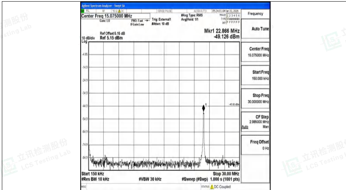
Band41_20MHz_16QAM_40620_1RB#0_0.15~30_0.15~30
