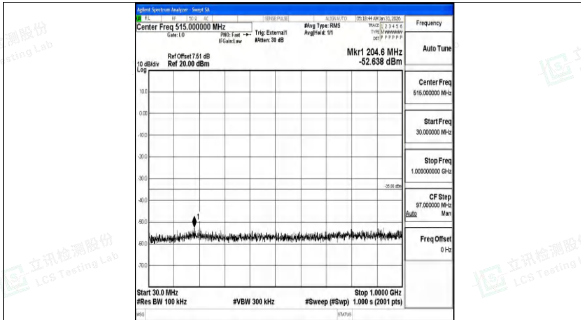
Band41_20MHz_QPSK_39750_1RB#0_30~1000_30~1000
