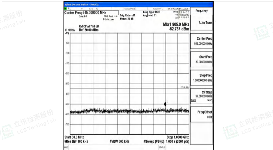
Band41_10MHz_QPSK_39700_1RB#0_30~1000_30~1000
