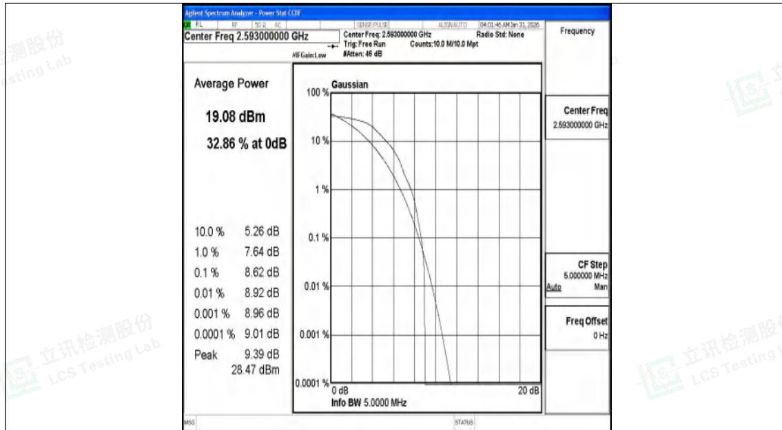
Band41-5MHz-QPSK-40620-1RB#0-PASS
