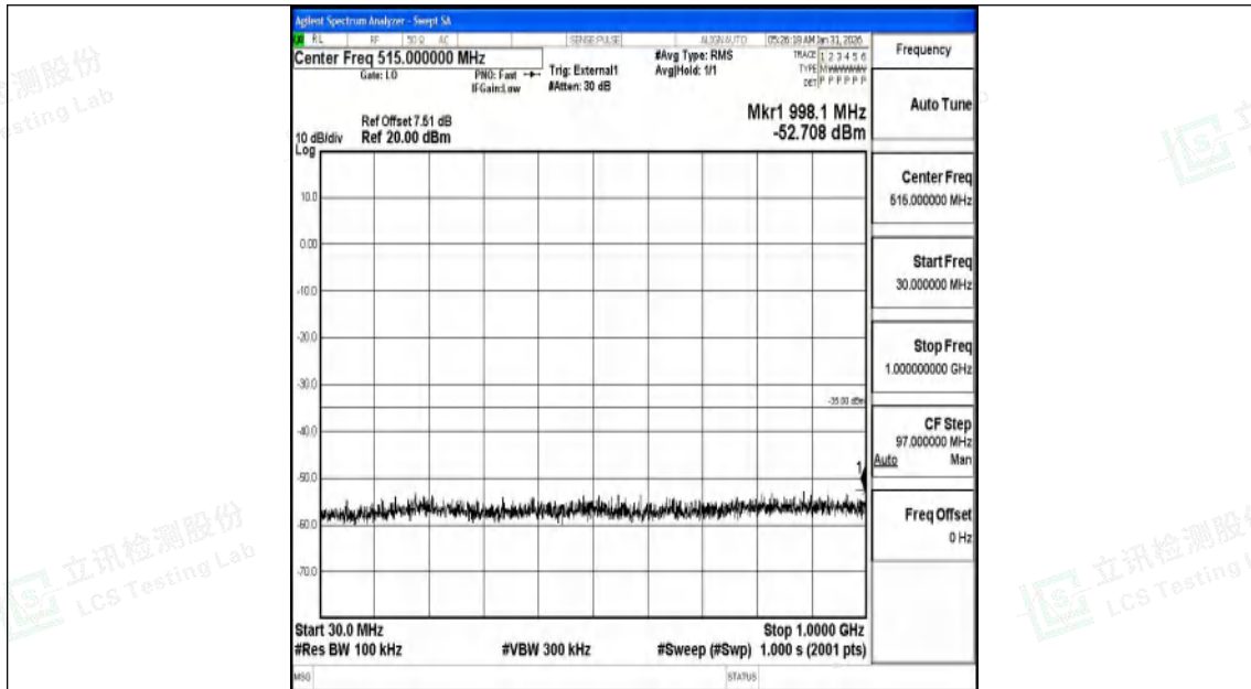
Band41_20MHz_QPSK_41490_1RB#0_30~1000_30~1000
