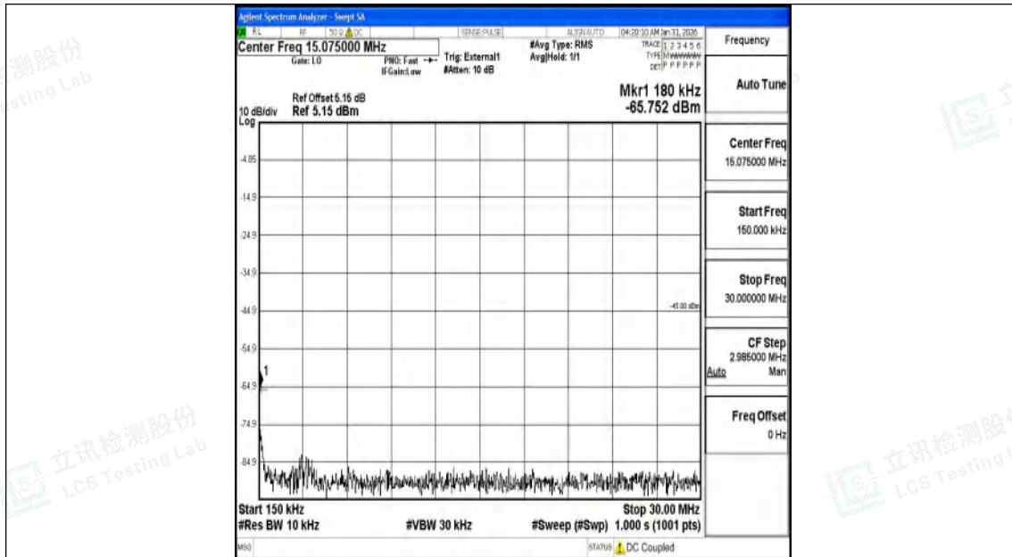
Band41_10MHz_16QAM_39700_1RB#0_0.15~30_0.15~30
