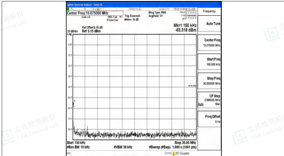
Band41_20MHz_16QAM_39750_1RB#0_0.15~30_0.15~30
