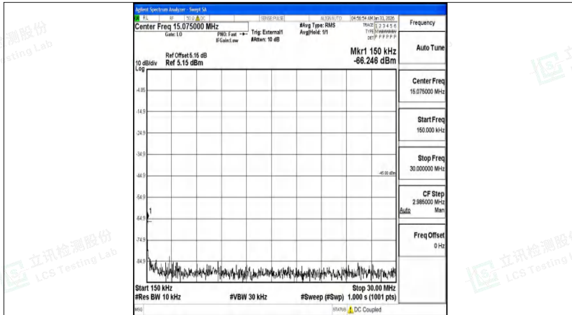
Band41_15MHz_16QAM_41515_1RB#0_0.15~30_0.15~30
