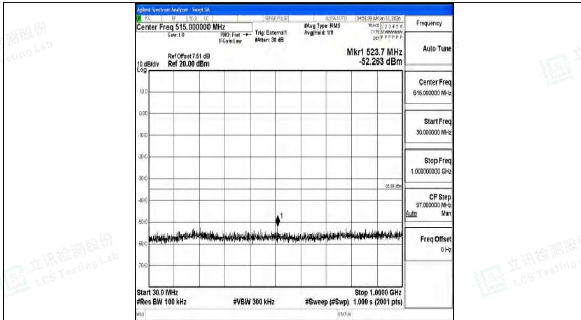
Band41_15MHz_QPSK_40620_1RB#0_30~1000_30~1000
