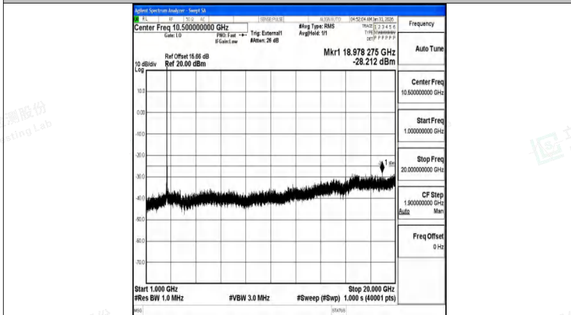
Band41_15MHz_QPSK_40620_1RB#0_1000~20000_1000~20000
