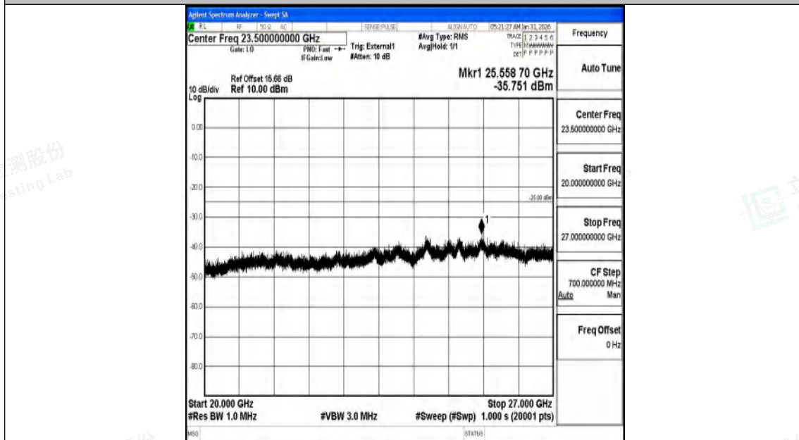
Band41_20MHz_16QAM_39750_1RB#0_20000~27000_20000~27000
