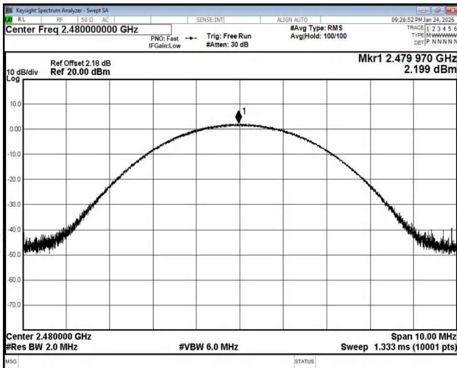
Peak Power NVNT 3-DH5 2480MHz Ant1
