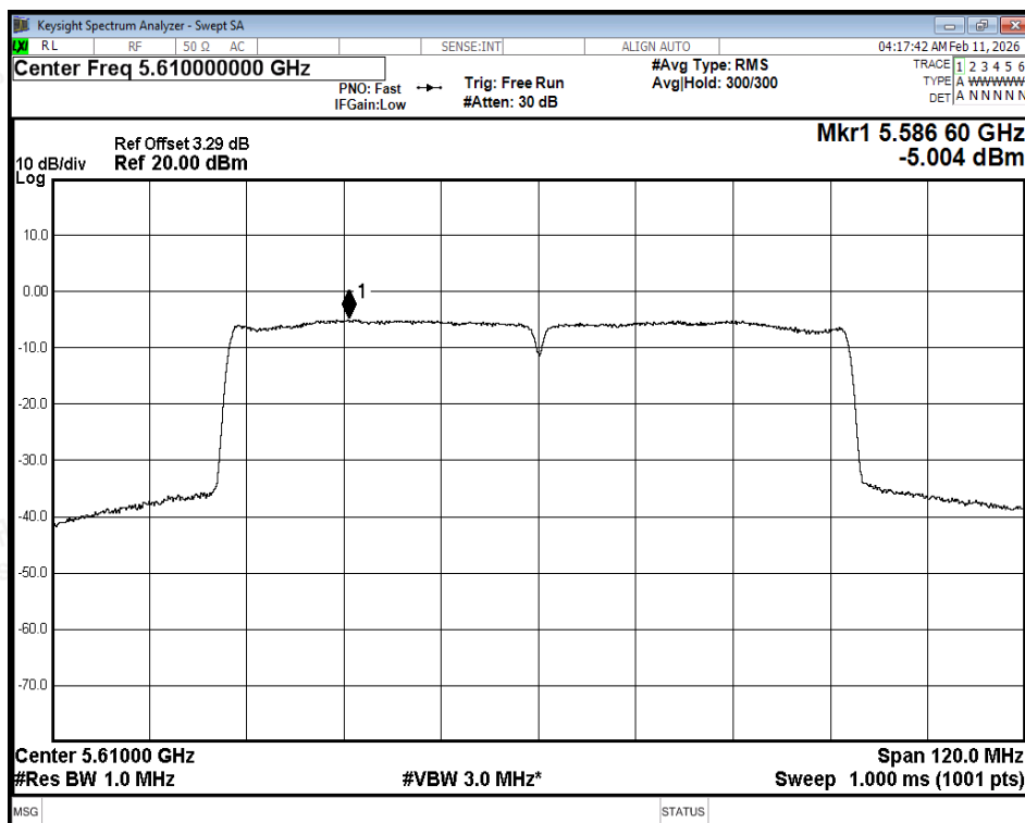
PSD NVNT ax80 5610MHz Ant2
