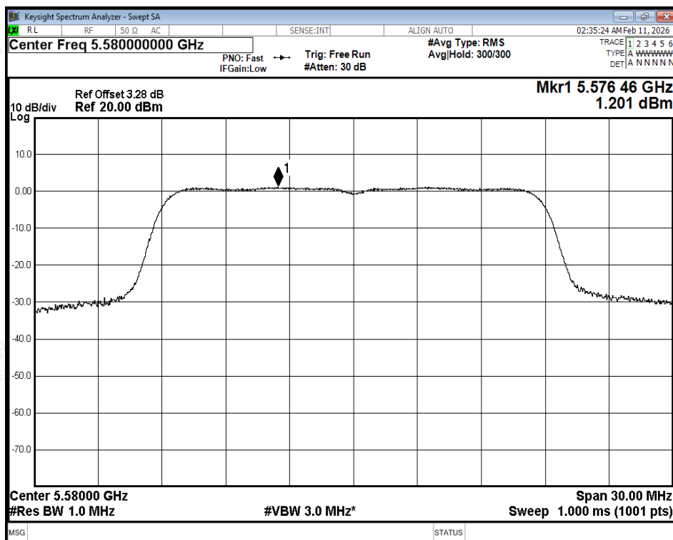
PSD NVNT ac20 5580MHz Ant2
