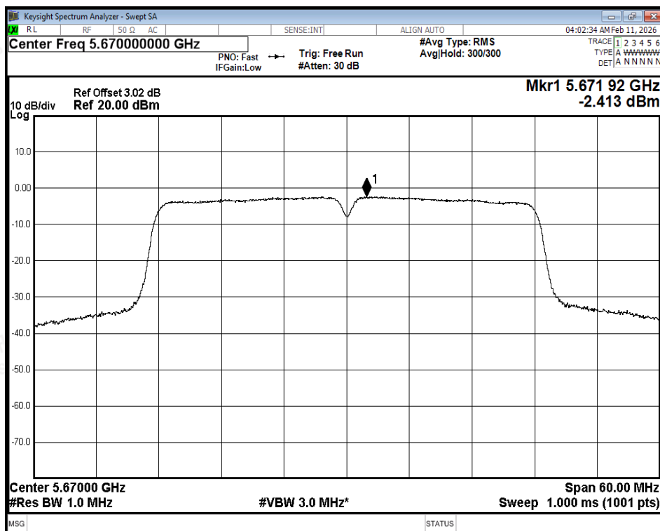
PSD NVNT ac40 5670MHz Ant2
