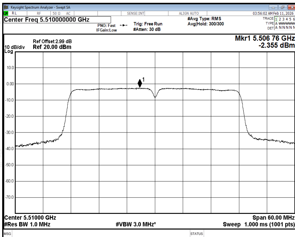
PSD NVNT ax40 5510MHz Ant2
