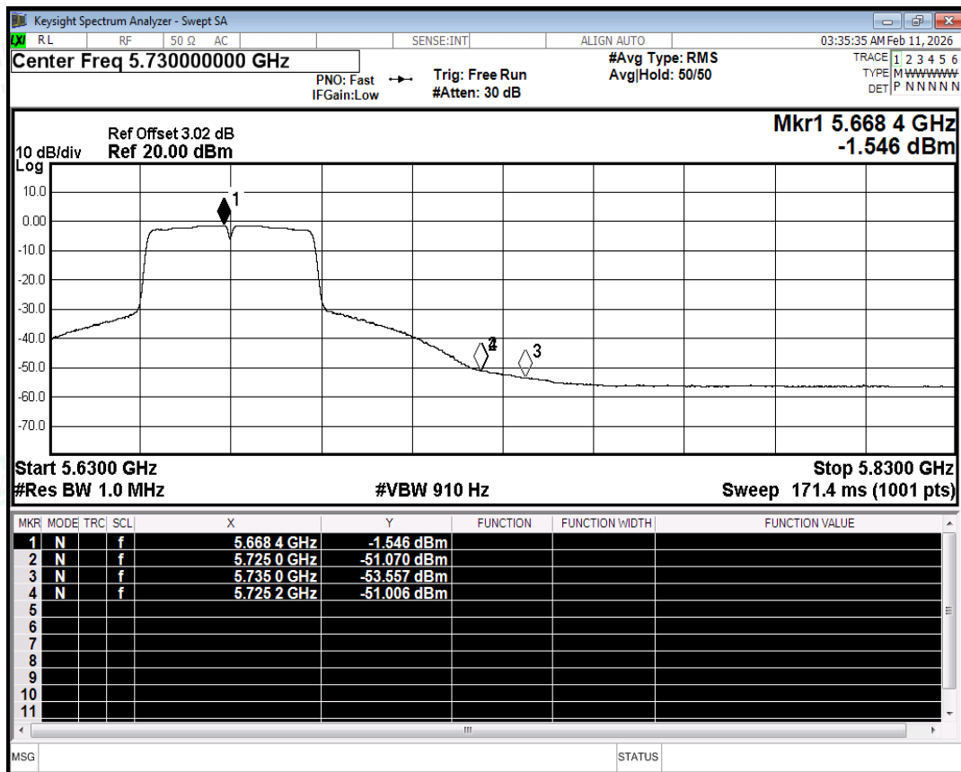
Restrict Band NVNT n40 5670MHz Ant2 Peak
