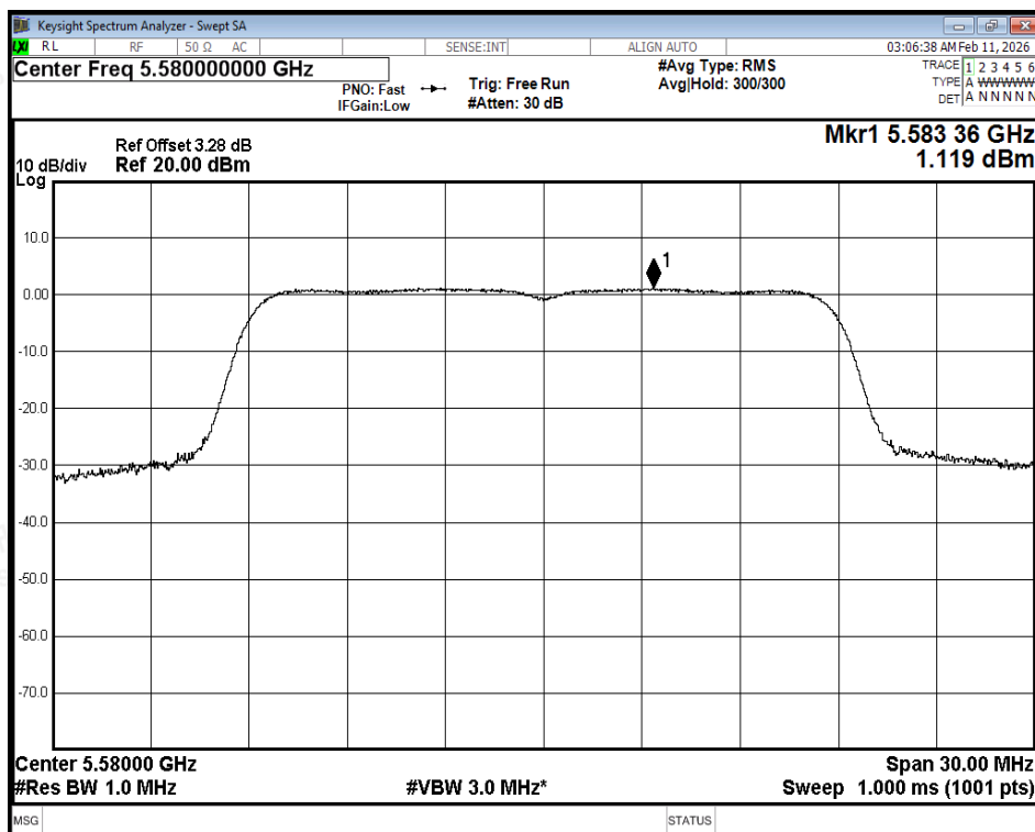
PSD NVNT ax20 5580MHz Ant2
