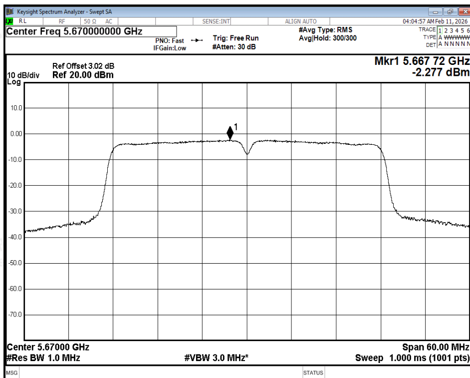
PSD NVNT ax40 5670MHz Ant2
