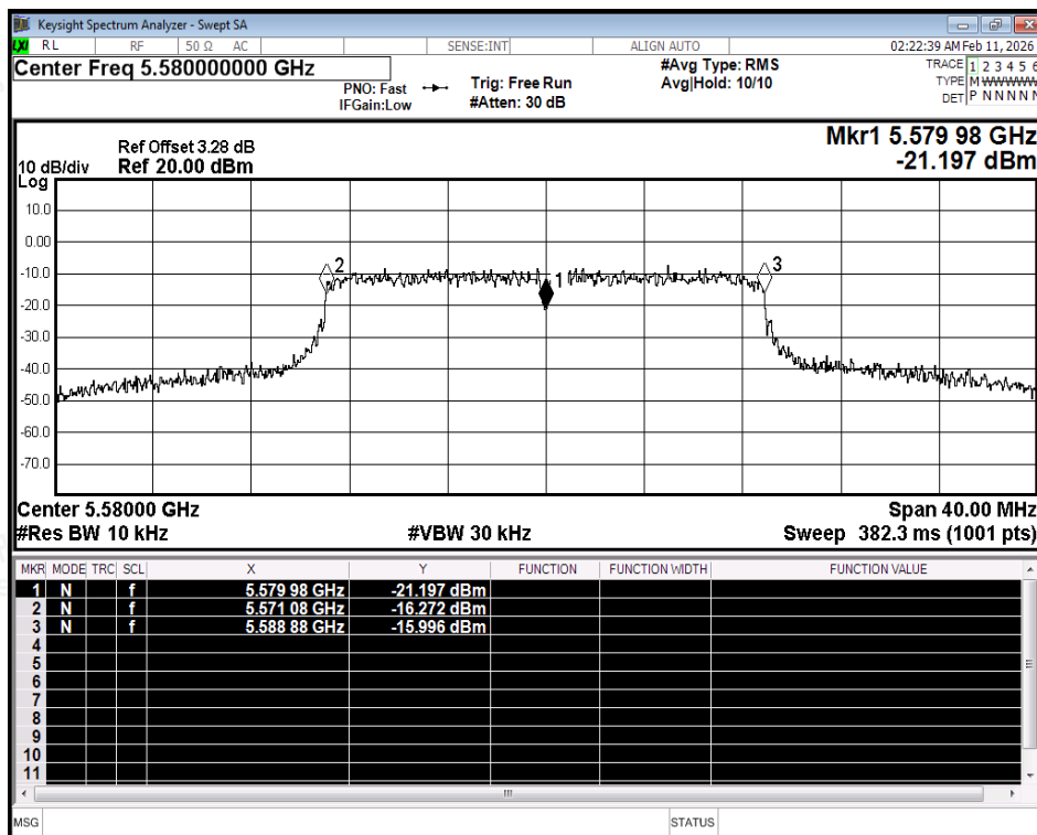
Freq. Stability NVNT n20 5580MHz Ant2
