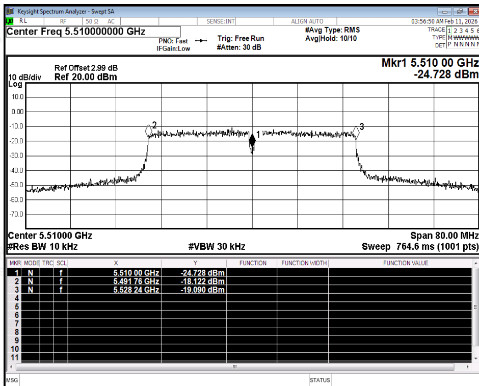
Freq. Stability NVNT ax40 5510MHz Ant2
