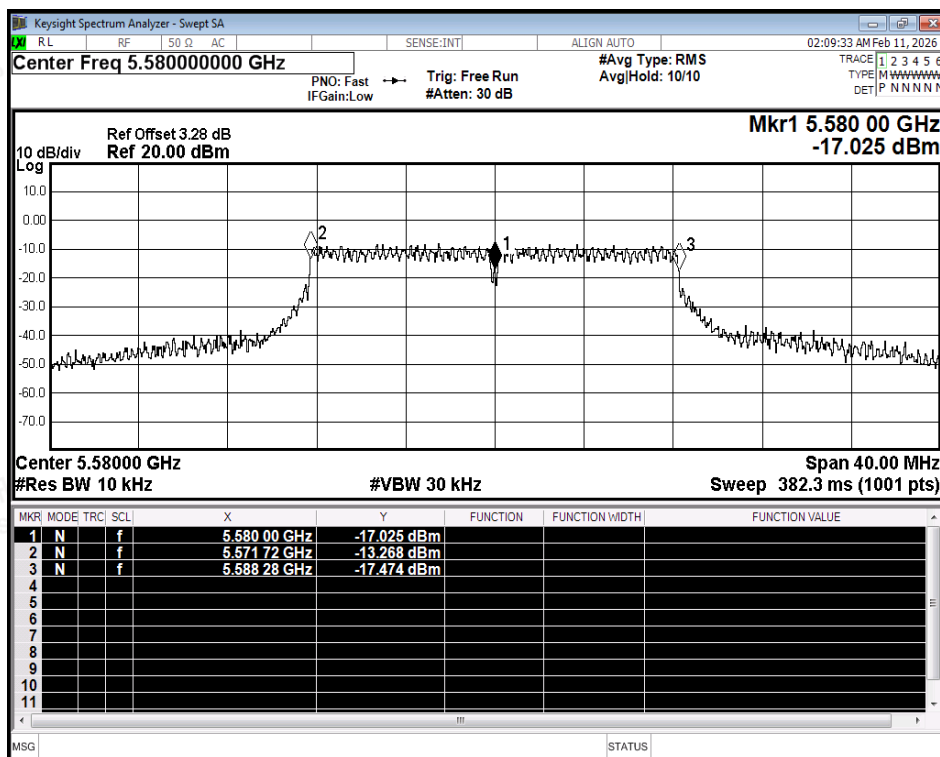
Freq. Stability NVNT a 5580MHz Ant2
