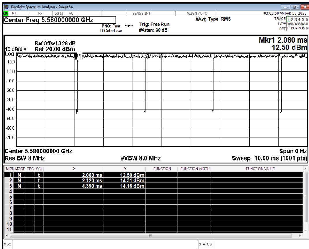
Duty Cycle NVNT ax20 5580MHz Ant2
