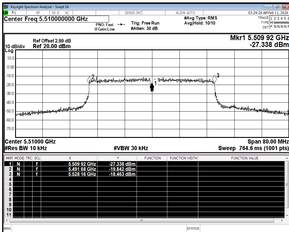
Freq. Stability NVNT n40 5510MHz Ant2
