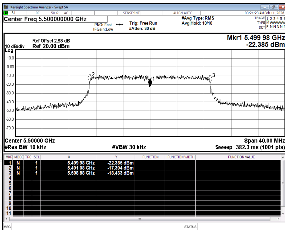
Freq. Stability NVNT ax20 5500MHz Ant2
