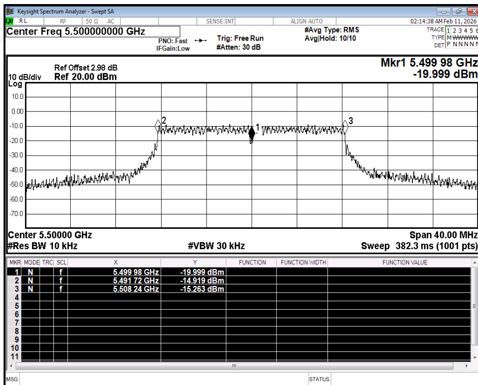
Freq. Stability NVNT a 5500MHz Ant2
