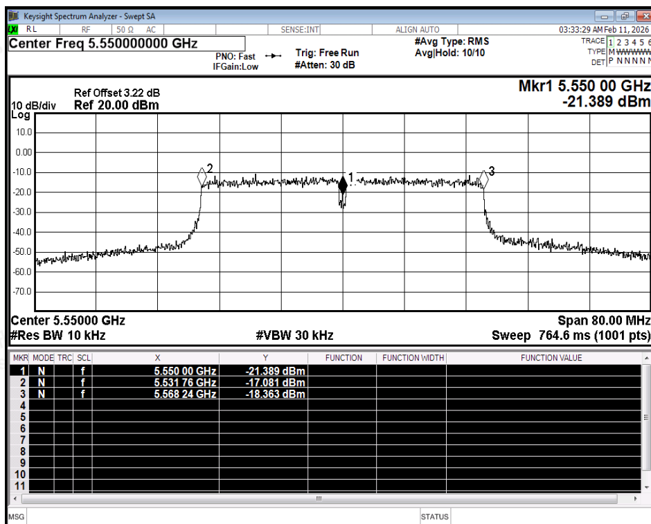
Freq. Stability NVNT n40 5550MHz Ant2
