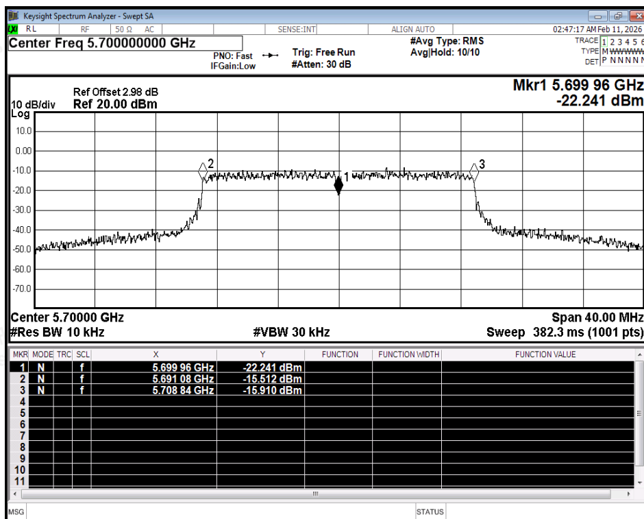
Freq. Stability NVNT ac20 5700MHz Ant2
