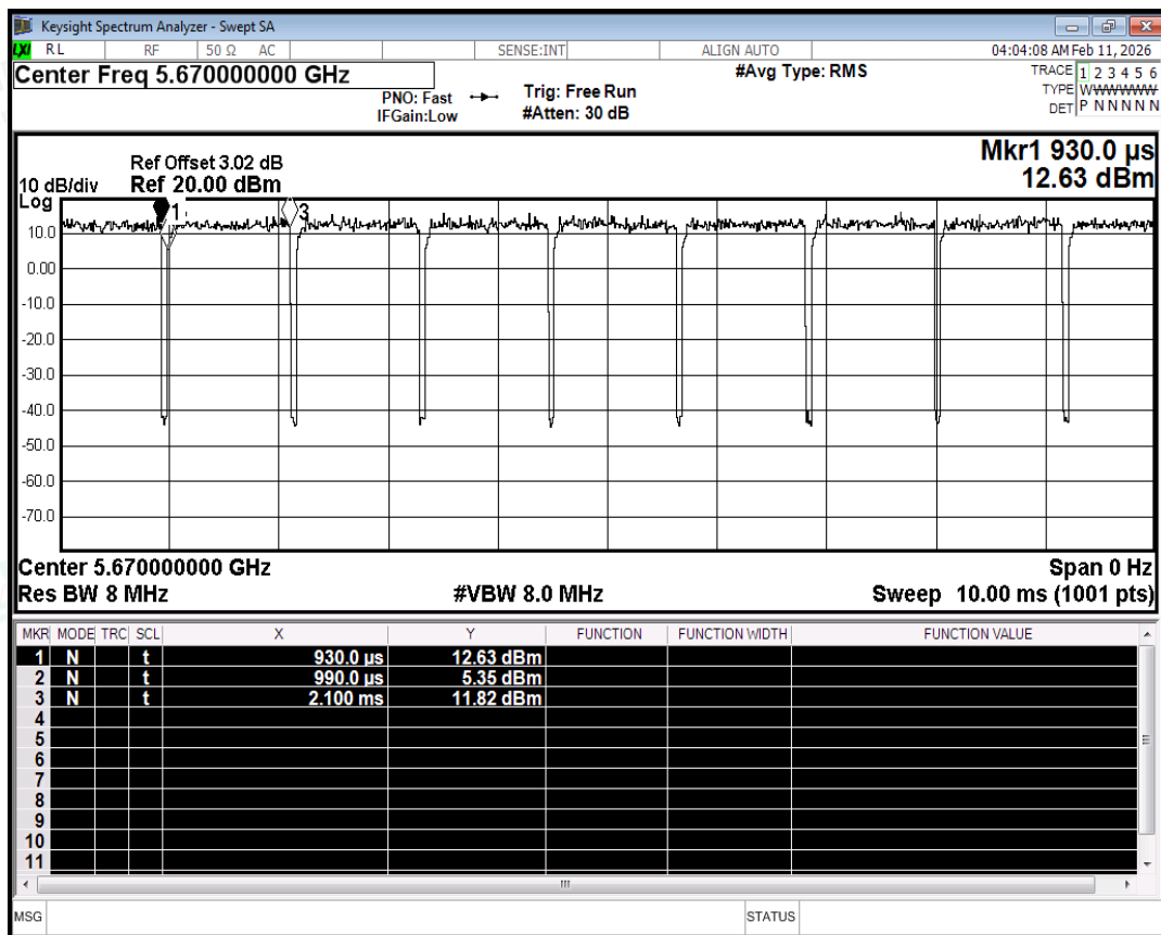
Duty Cycle NVNT ax40 5670MHz Ant2
