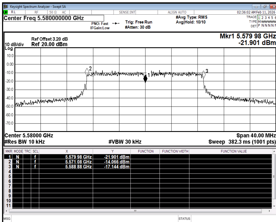
Freq. Stability NVNT ac20 5580MHz Ant2
