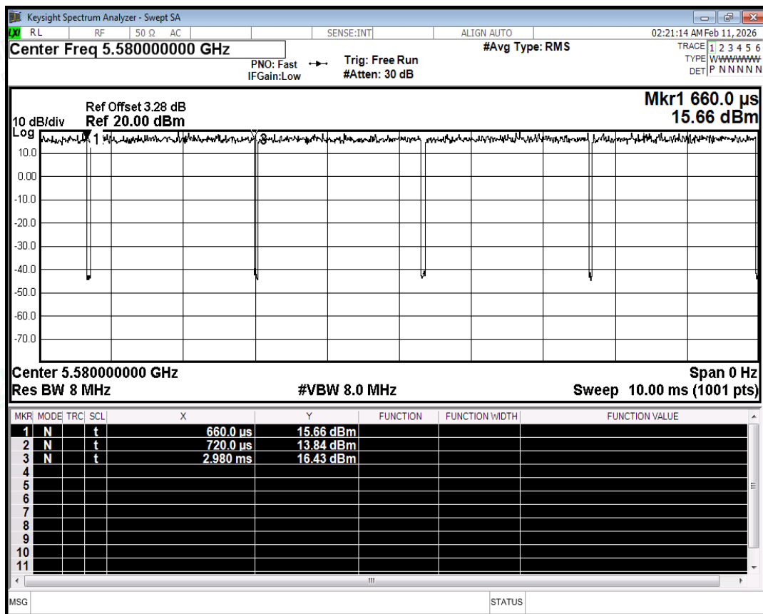
Duty Cycle NVNT n20 5580MHz Ant2
