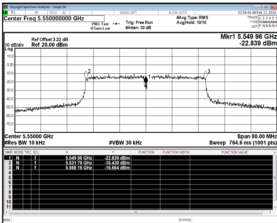
Freq. Stability NVNT ax40 5550MHz Ant2
