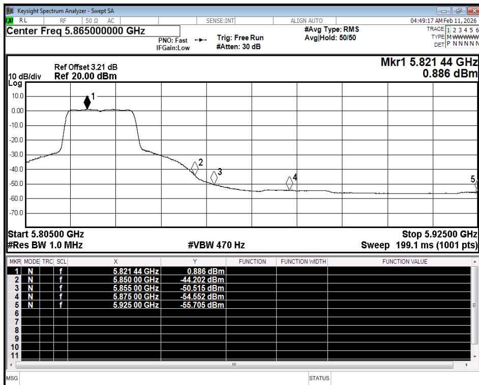
Restrict Band NVNT ax20 5825MHz Ant2 Average
