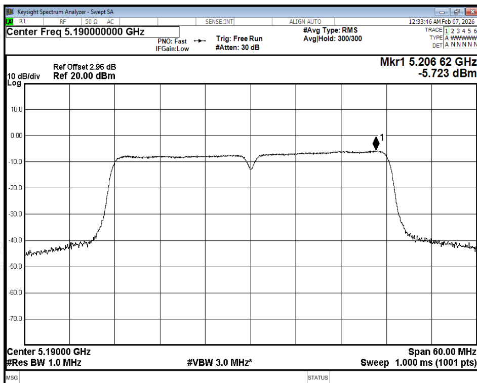
PSD NVNT ax40 5190MHz Ant2
