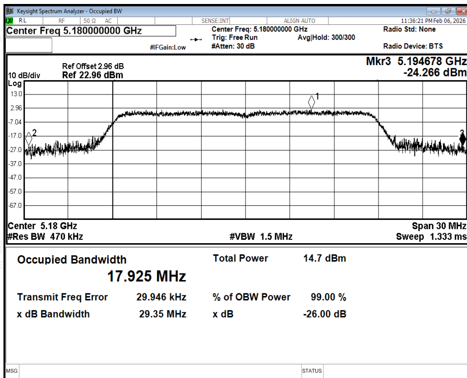
-26dB Bandwidth NVNT ac20 5180MHz Ant2
