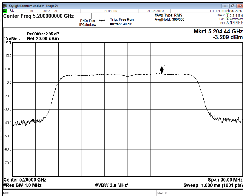
PSD NVNT n20 5200MHz Ant2
