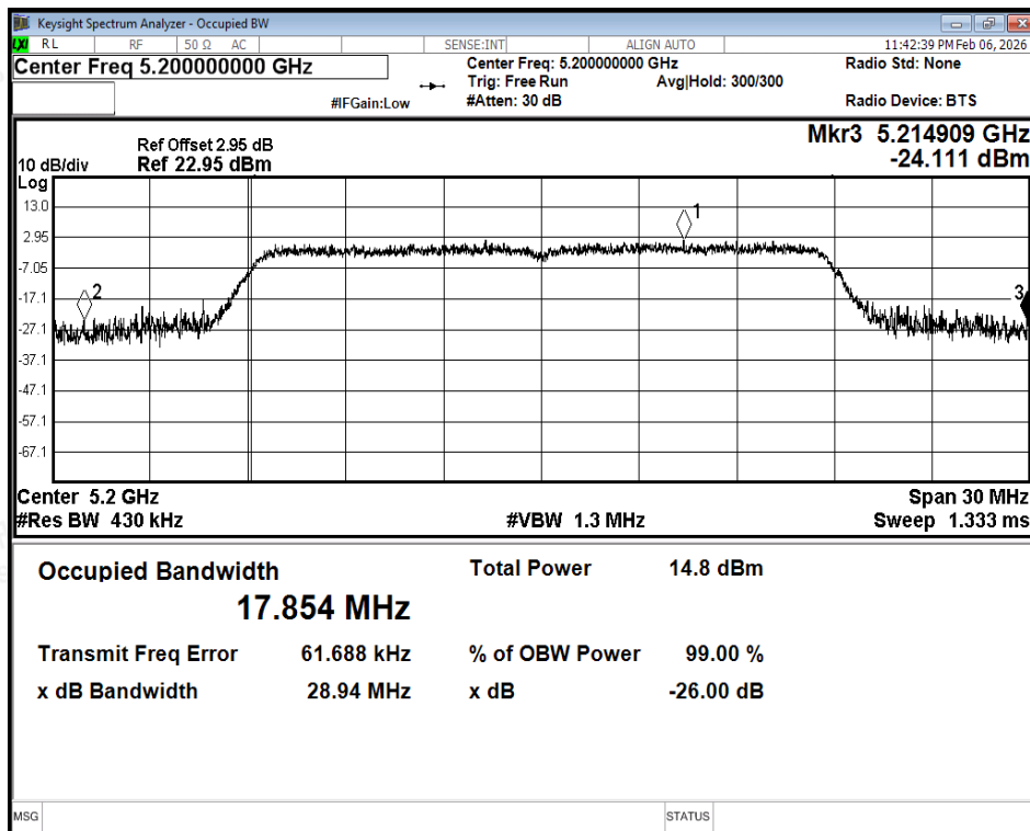
-26dB Bandwidth NVNT ac20 5200MHz Ant2
