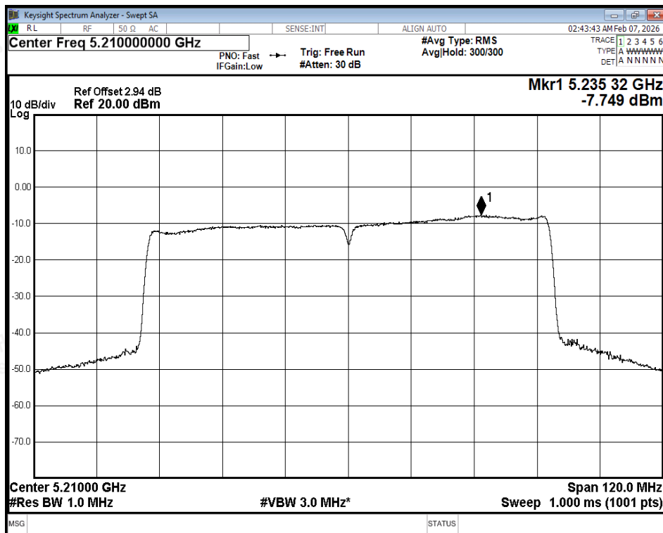
PSD NVNT ax80 5210MHz Ant2
