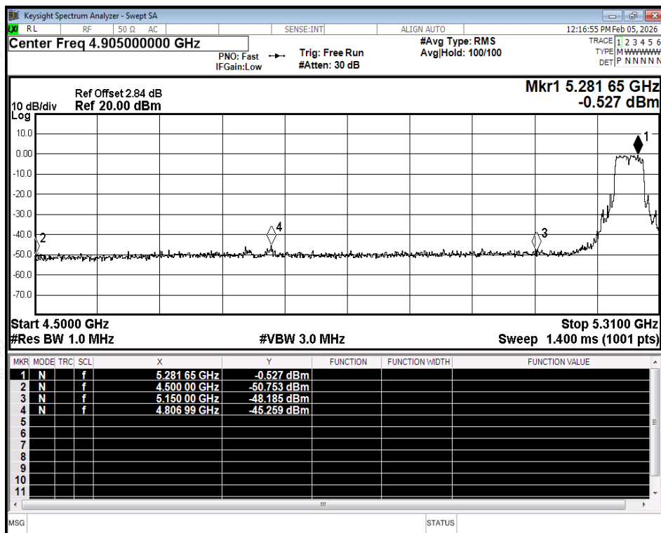
Restrict Band NVNT ax40 5270MHz Ant1 Peak
