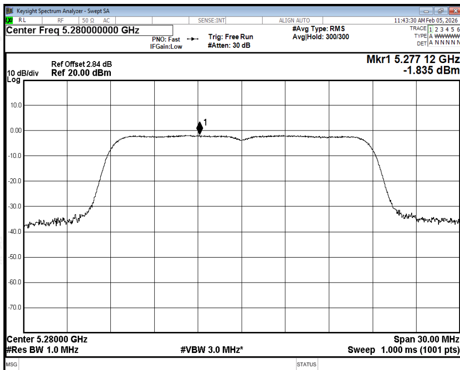
PSD NVNT n20 5280MHz Ant1
