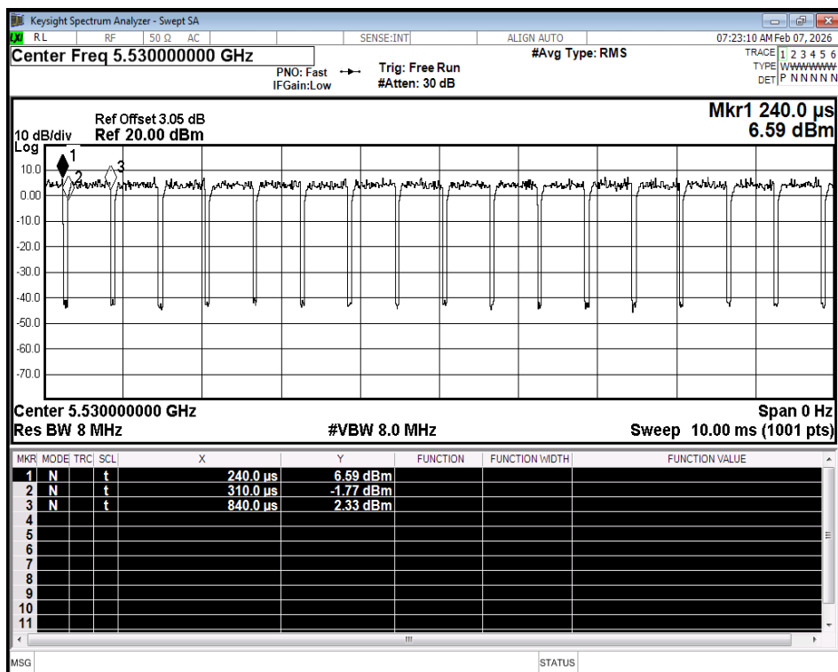
Duty Cycle NVNT ac80 5530MHz Ant2
