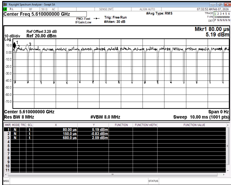
Duty Cycle NVNT ax80 5610MHz Ant2
