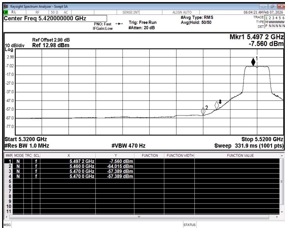
Restrict Band NVNT ac20 5500MHz Ant2 Average
