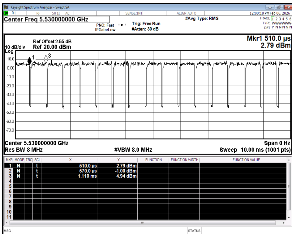
Duty Cycle NVNT ax80 5530MHz Ant1
