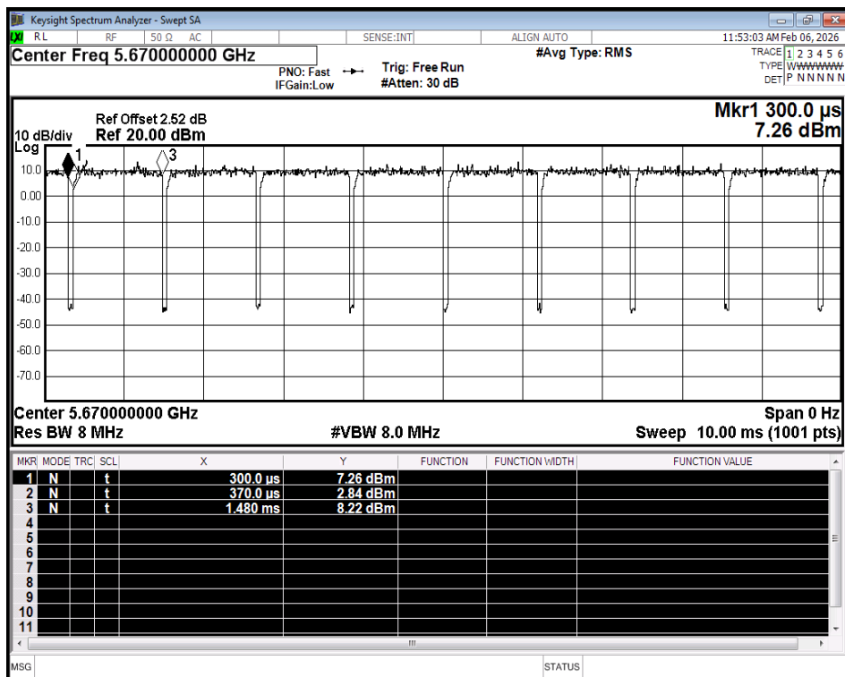
Duty Cycle NVNT ax40 5670MHz Ant1
