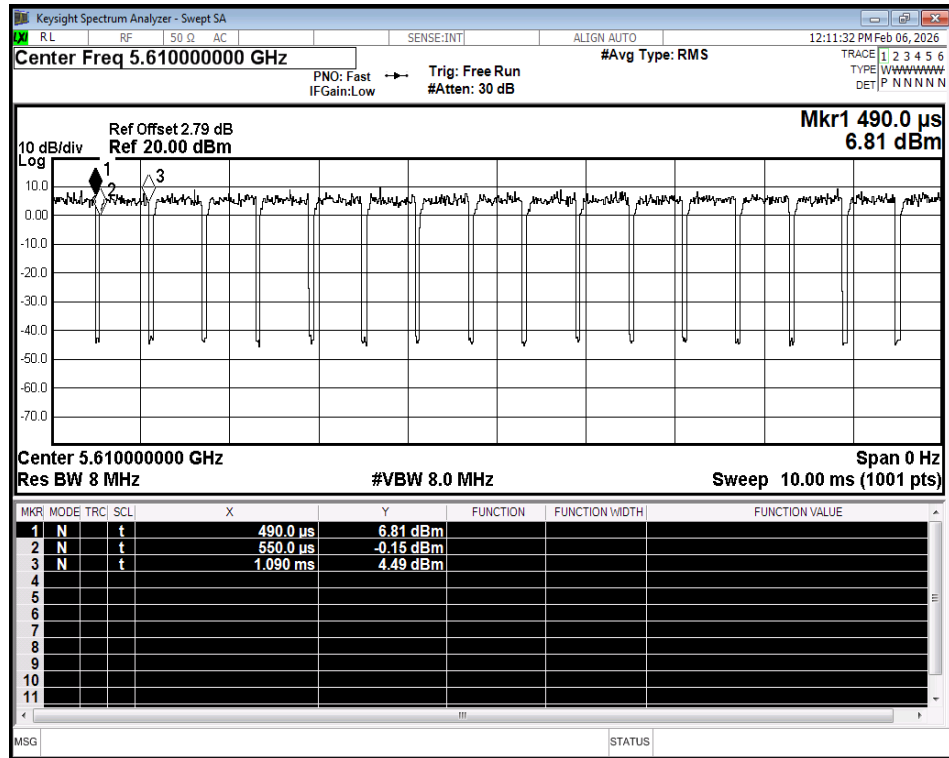
Duty Cycle NVNT ax80 5610MHz Ant1
