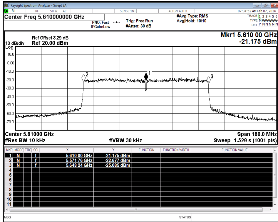
Freq. Stability NVNT ax80 5610MHz Ant2
