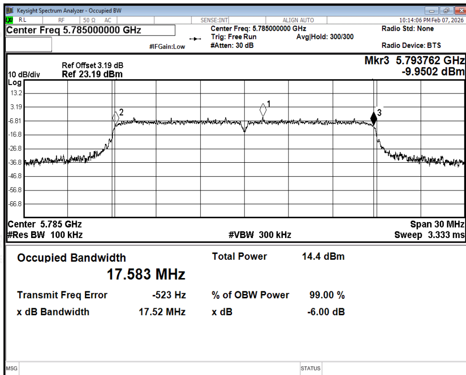
-6dB Bandwidth NVNT ac20 5785MHz Ant2
