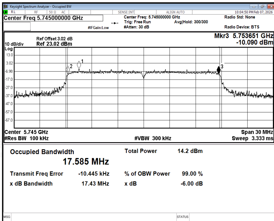
-6dB Bandwidth NVNT ac20 5745MHz Ant2
