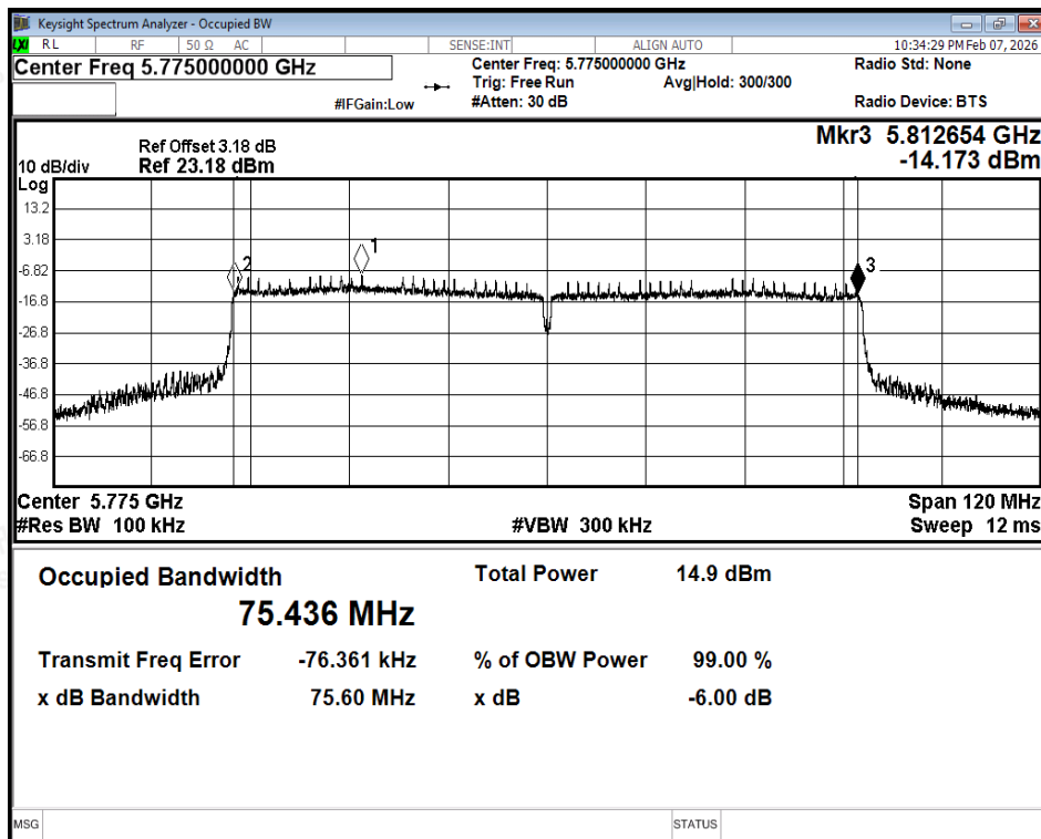
-6dB Bandwidth NVNT ac80 5775MHz Ant2
