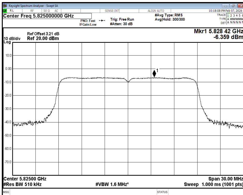
PSD NVNT ax20 5825MHz Ant2
