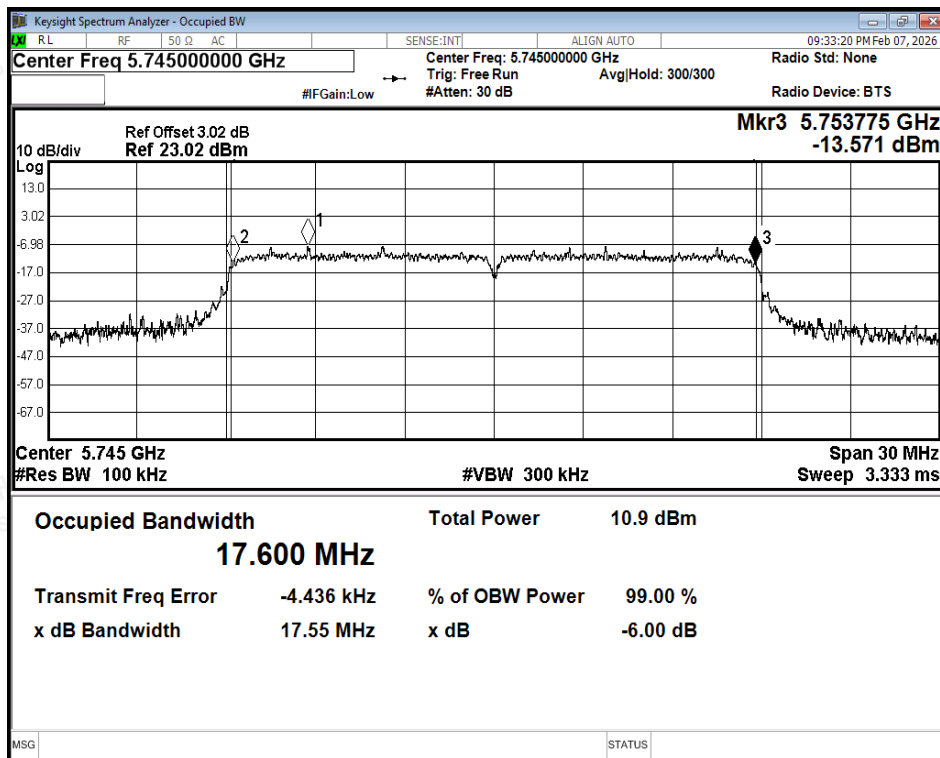
-6dB Bandwidth NVNT n20 5745MHz Ant2
