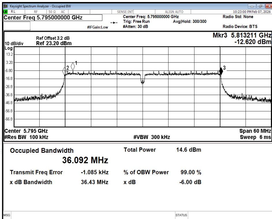
-6dB Bandwidth NVNT n40 5795MHz Ant2
