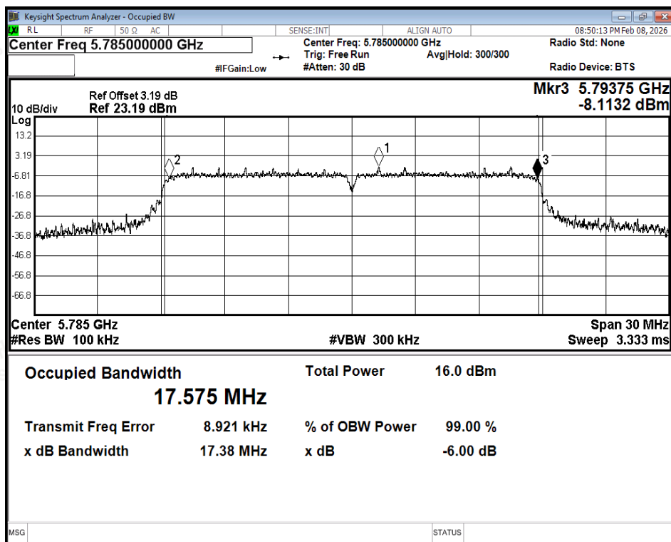
-6dB Bandwidth NVNT ac20 5785MHz Ant1
