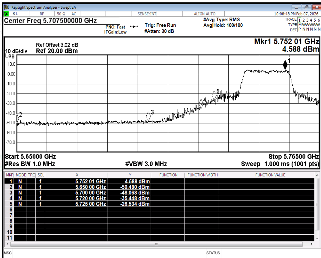
Restrict Band NVNT ax20 5745MHz Ant2 Peak
