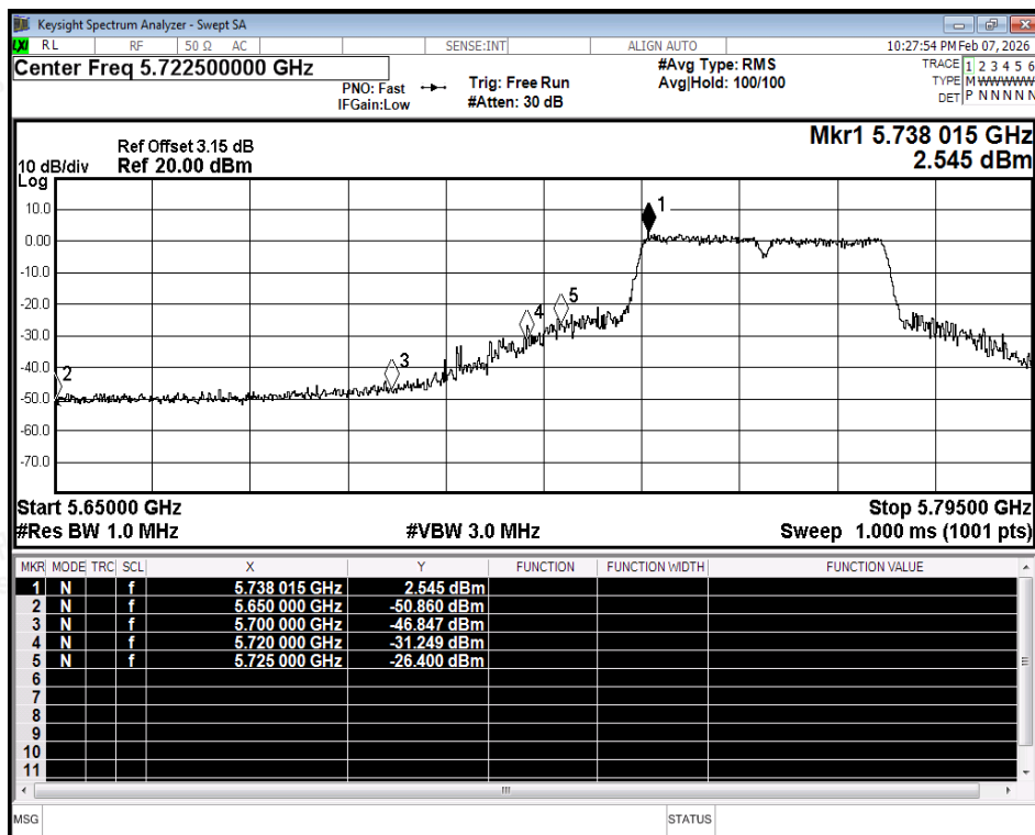
Restrict Band NVNT ax40 5755MHz Ant2 Peak
