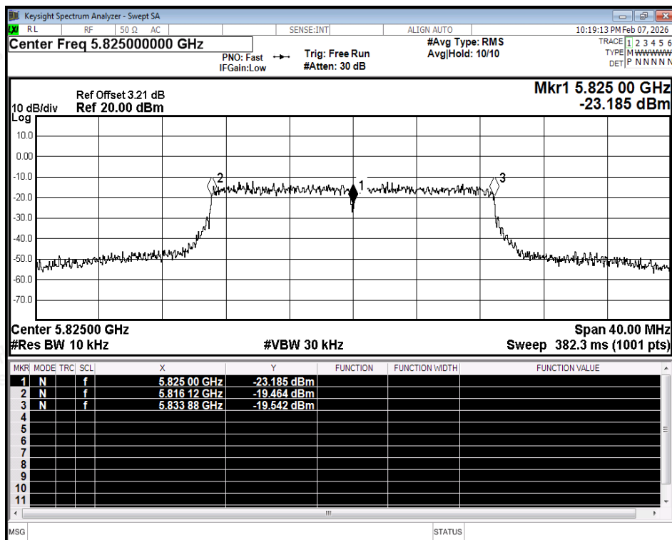
Freq. Stability NVNT ax20 5825MHz Ant2
