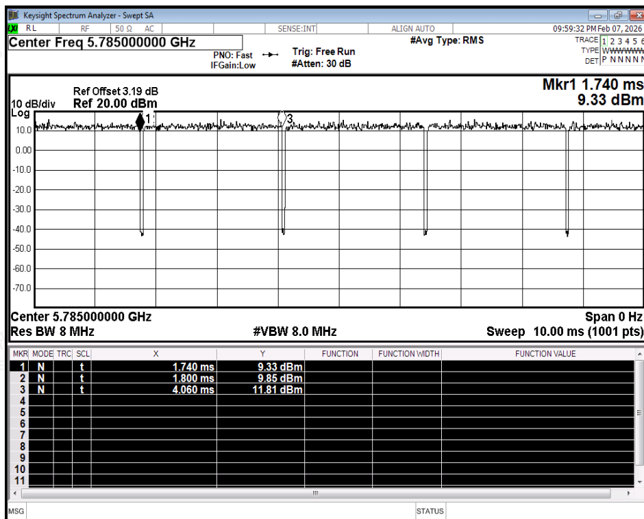
Duty Cycle NVNT n20 5785MHz Ant2
