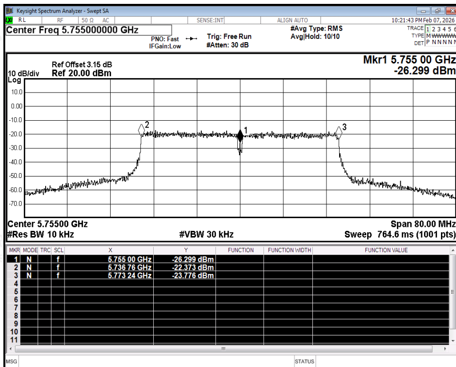
Freq. Stability NVNT n40 5755MHz Ant2
