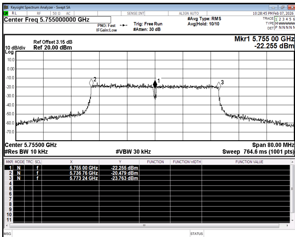
Freq. Stability NVNT ax40 5755MHz Ant2
