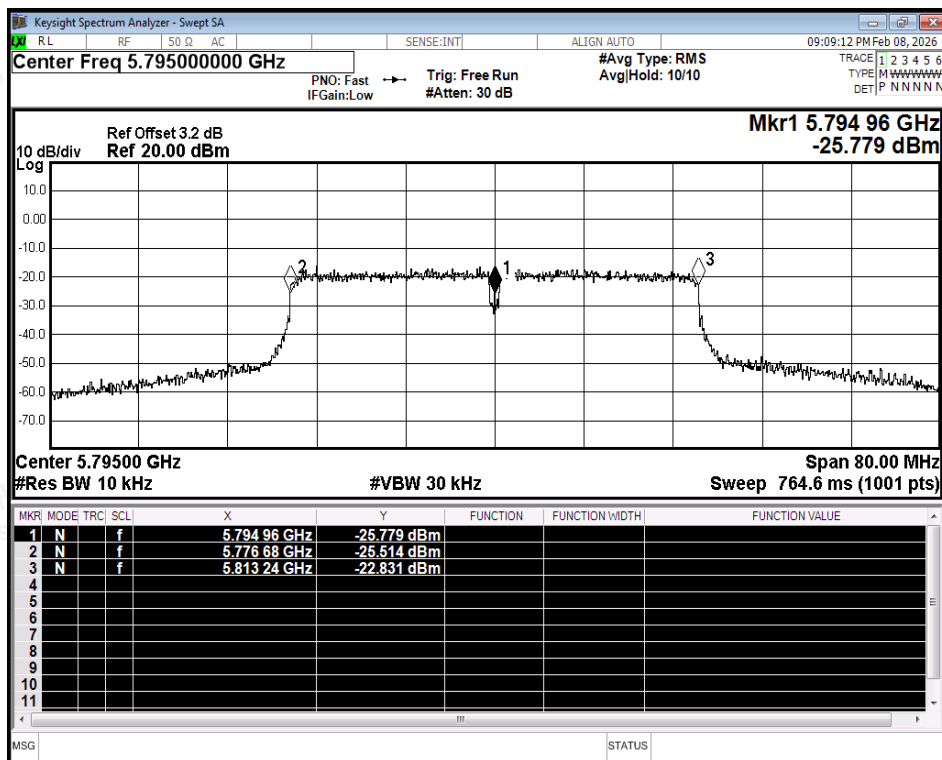
Freq. Stability NVNT ac40 5795MHz Ant1
