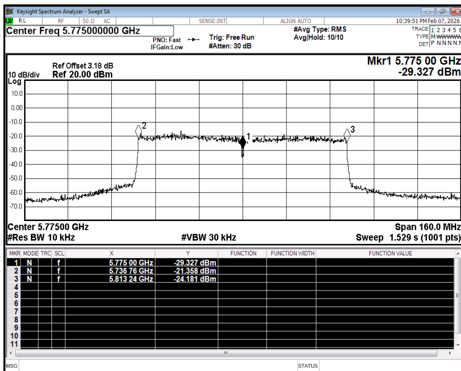
Freq. Stability NVNT ax80 5775MHz Ant2
