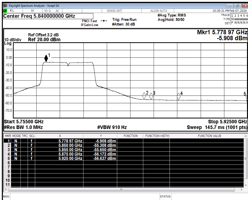
Restrict Band NVNT ac40 5795MHz Ant2 Average
