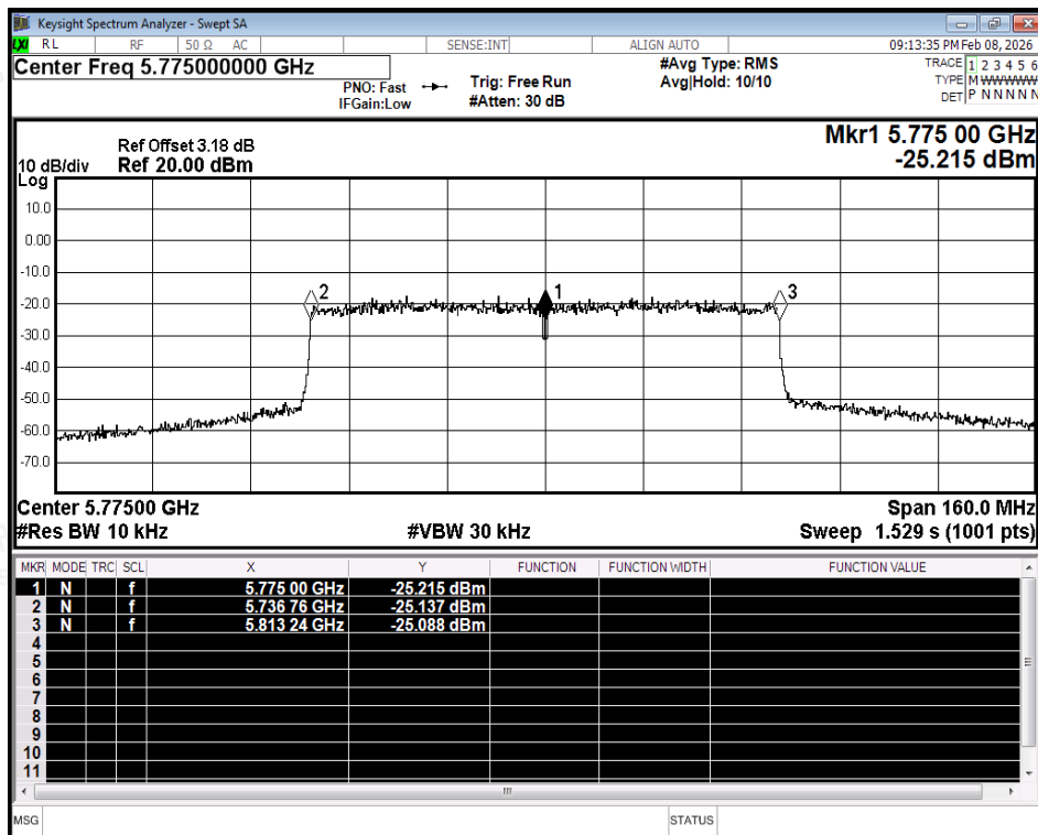
Freq. Stability NVNT ac80 5775MHz Ant1
