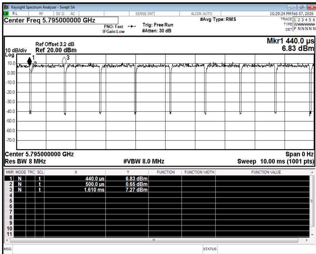
Duty Cycle NVNT ac40 5795MHz Ant2
