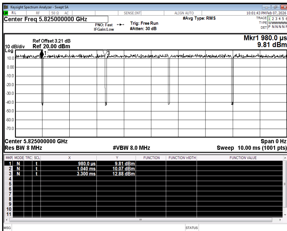
Duty Cycle NVNT n20 5825MHz Ant2
