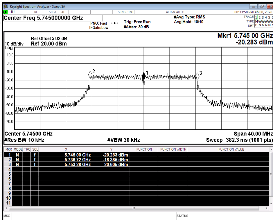
Freq. Stability NVNT a 5745MHz Ant1
