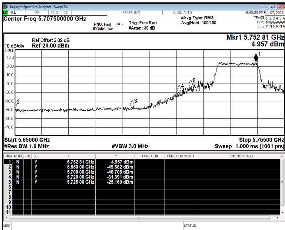
Restrict Band NVNT ac20 5745MHz Ant2 Peak
