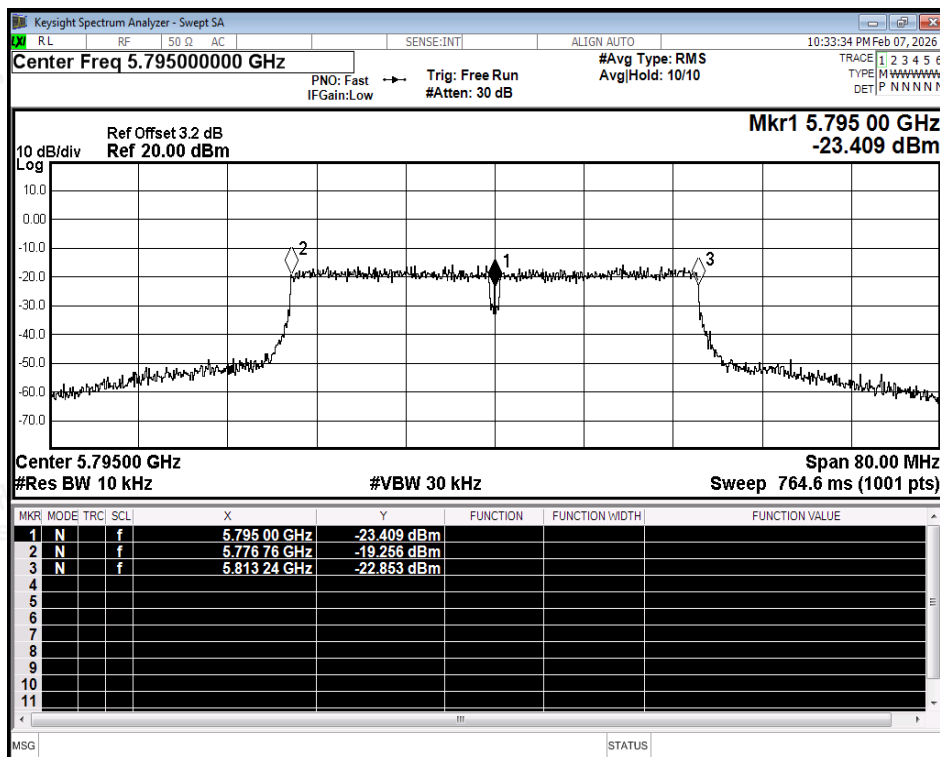
Freq. Stability NVNT ax40 5795MHz Ant2
