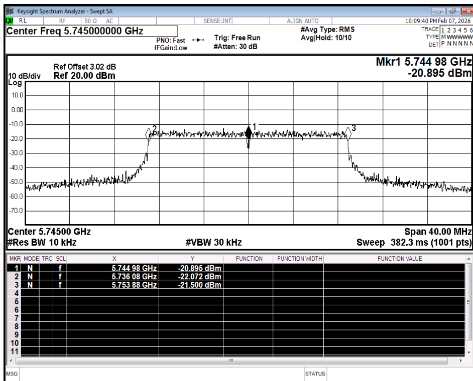
Freq. Stability NVNT ax20 5745MHz Ant2
