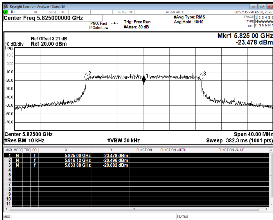
Freq. Stability NVNT ax20 5825MHz Ant1
