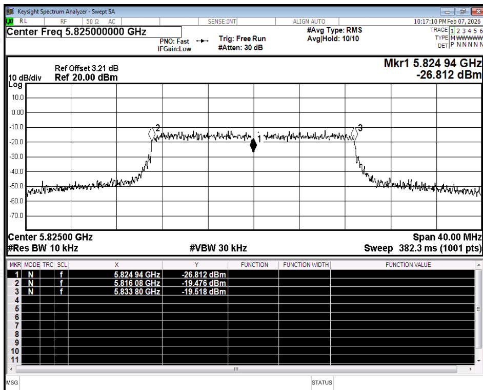
Freq. Stability NVNT ac20 5825MHz Ant2
