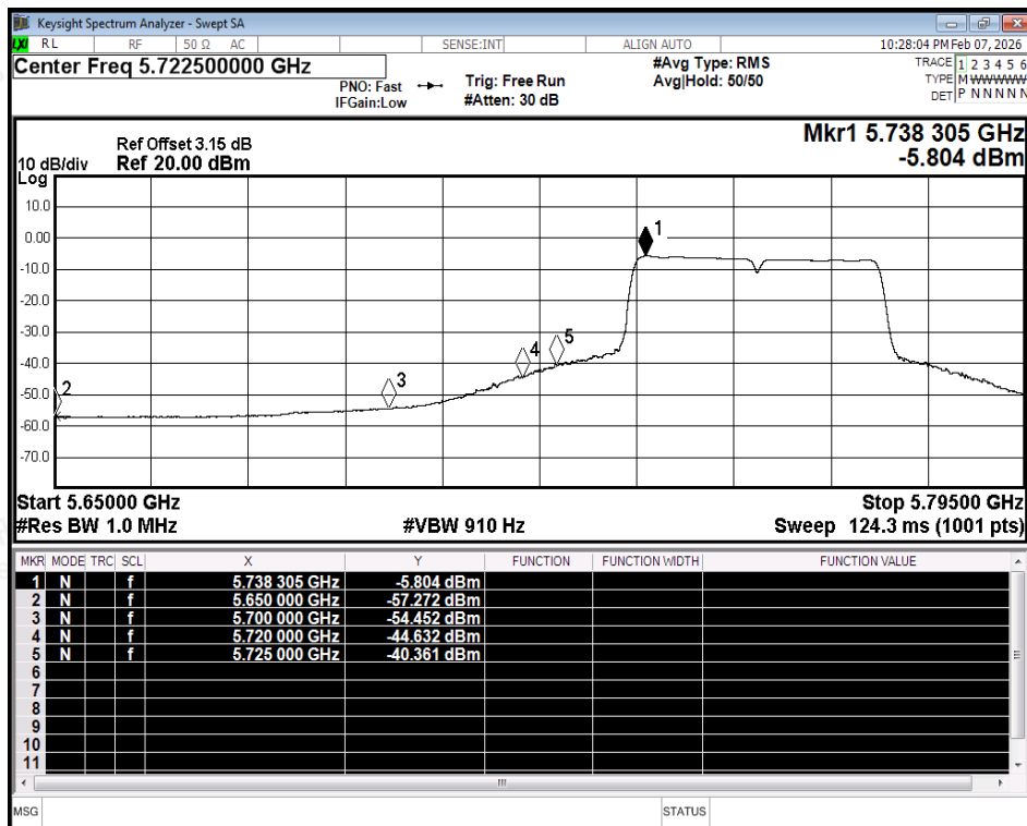
Restrict Band NVNT ax40 5755MHz Ant2 Average
