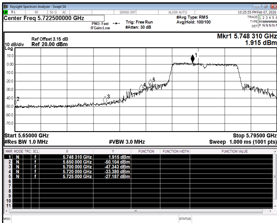
Restrict Band NVNT ac40 5755MHz Ant2 Peak
