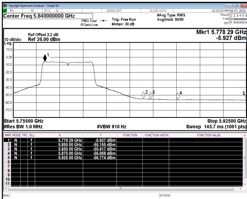
Restrict Band NVNT ax40 5795MHz Ant2 Average
