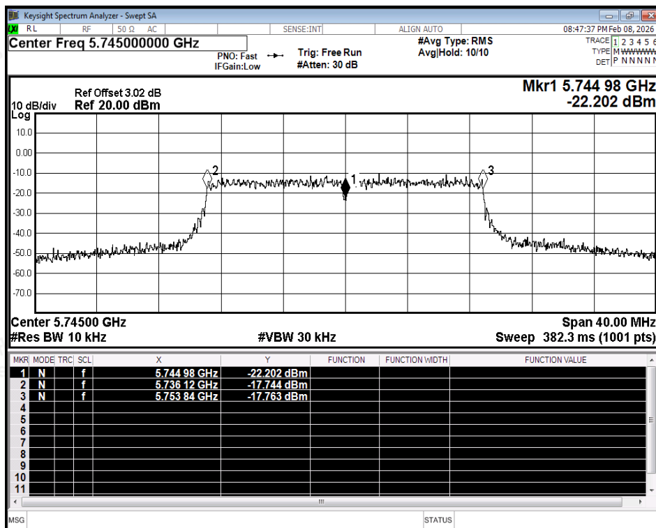
Freq. Stability NVNT ac20 5745MHz Ant1
