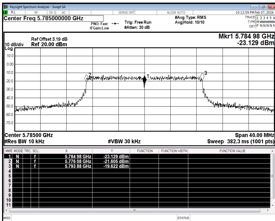
Freq. Stability NVNT ax20 5785MHz Ant2
