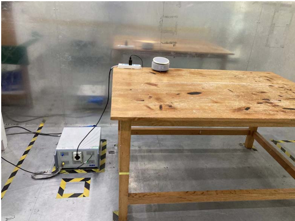
Conducted setup (Bluetooth)
