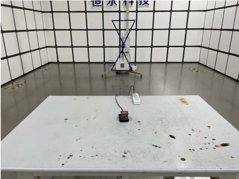
Radiated Test (Above 30MHz) AC power in
