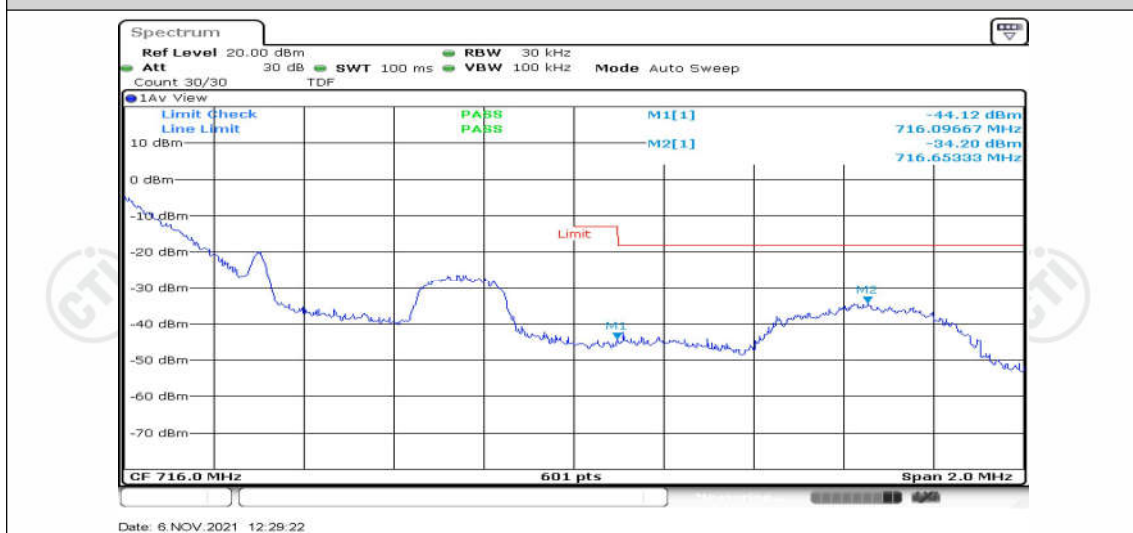
Band12-1.4MHz-QPSK-23173-1RB#5
