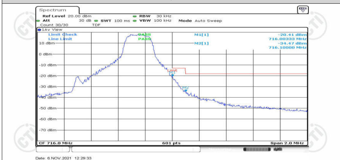
Band12-1.4MHz-QPSK-23173-6RB#0
