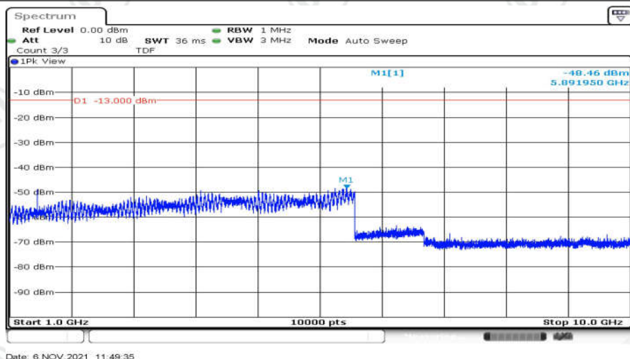
Band12-1.4MHz-QPSK-23095-1RB#0-Range1:30~1000MHz
