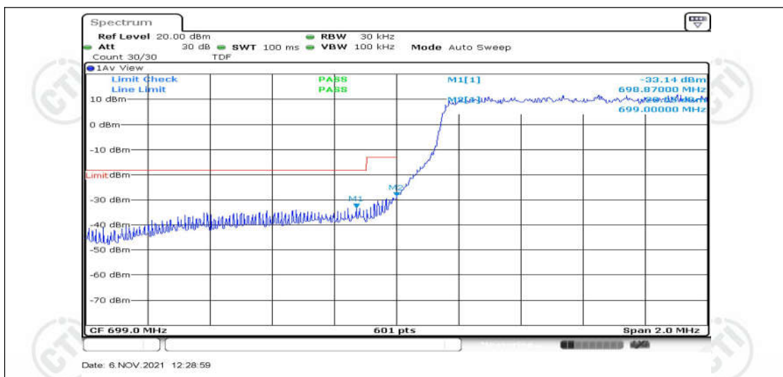
Band12-1.4MHz-QPSK-23173-1RB#0
