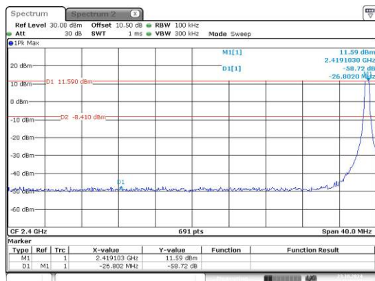
2419MHz-Low
