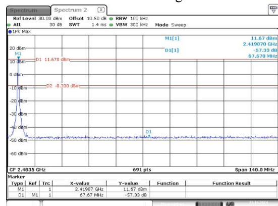
2419MHz-High
